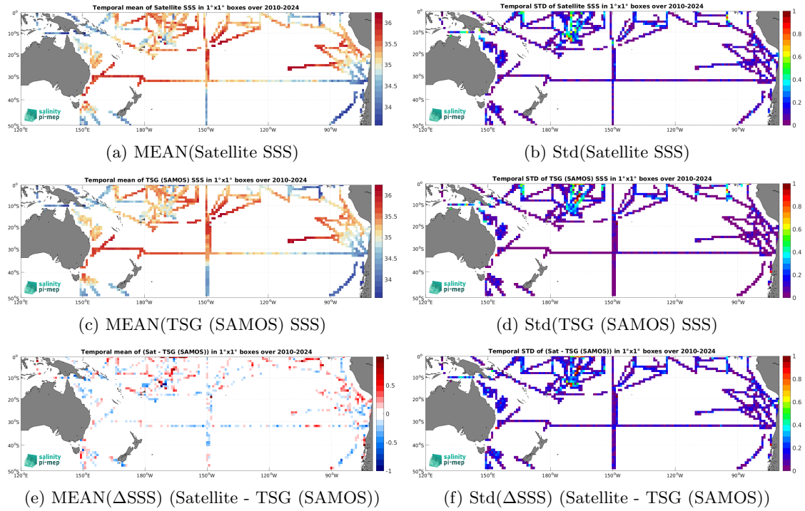
Figure 7: Temporal mean (left) and Std (right) of SSS from SMOS SSS L3 v332 - 9 Days (CATDS-CPDC) (top), TSG (SAMOS) (middle), and of \Delta SSS (Satellite - TSG (SAMOS)). Only match-up pairs are used to generate these maps.
