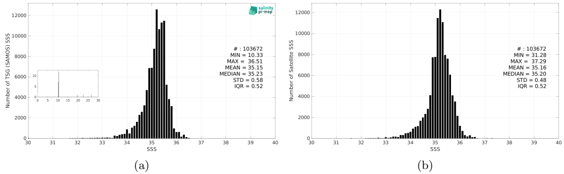
Figure 3: Histograms of SSS from TSG (SAMOS) (a) and SMOS SSS L3 v332 - 9 Days (CATDS-CPDC) (b) considering all match-up pairs per bins of 0.1 over the South Pacific Ocean Pi-MEP region and for the full satellite product period.
