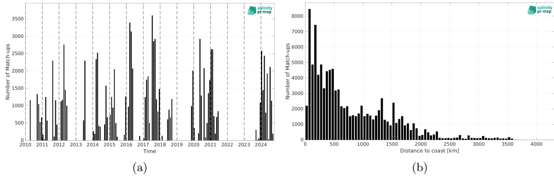
Figure 2: Number of match-ups between TSG (SAMOS) and SMOS SSS L3 v332 - 9 Days (CATDS-CPDC) SSS as a function of time (a) and as function of the distance to coast (b) over the South Pacific Ocean Pi-MEP region and for the full satellite product period.
