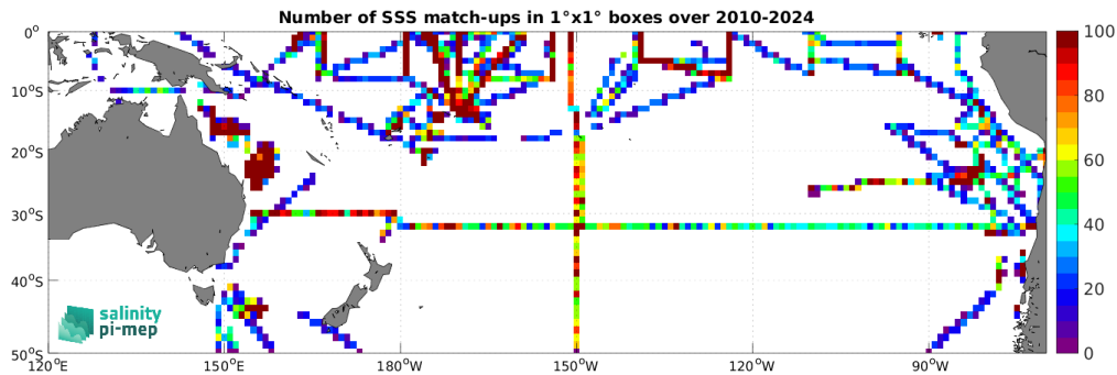
Figure 5: Number of SSS match-ups between TSG (SAMOS) SSS and the SMOS SSS L3 v332 - 9 Days (CATDS-CPDC) SSS product for the South Pacific Ocean Pi-MEP region over 1^\circ \times 1^\circ boxes and for the full satellite product period.
