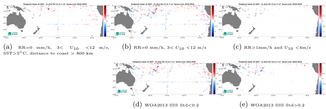
Figure 14: Temporal mean gridded over spatial boxes of size 1^\circ \times 1^\circ of \Delta\text{SSS} (SMOS SSS L3 v332 - 9 Days (CATDS-CPDC) - TSG (SAMOS)) for 5 different subdatasets corresponding to: RR=0 mm/h, 3 < U_{10} < 12 m/s, SST > 5°C, distance to coast > 800 km (a), RR=0 mm/h, 3 < U_{10} < 12 m/s (b), RR > 1mm/h and U_{10} < 4 m/s (c), WOA2013 SSS Std < 0.2 (d), WOA2013 SSS Std > 0.2 (e).
