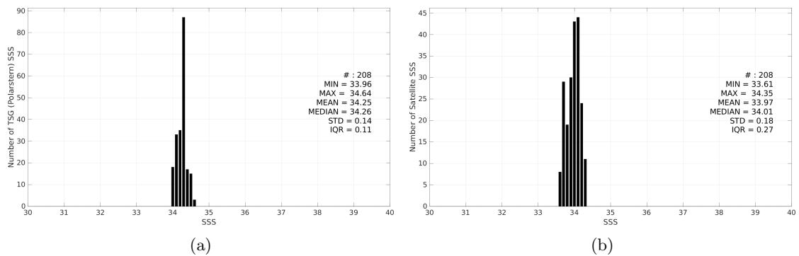
Figure 3: Histograms of SSS from TSG (Polarstern) (a) and SMOS SSS L3 v332 - 9 Days (CATDS-CPDC) (b) considering all match-up pairs per bins of 0.1 over the South Pacific Ocean Pi-MEP region and for the full satellite product period.
