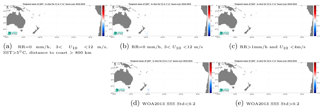
Figure 14: Temporal mean gridded over spatial boxes of size 1^\circ \times 1^\circ of \Delta SSS (SMOS SSS L3 v332 - 9 Days (CATDS-CPDC) - TSG (Polarstern)) for 5 different subdatasets corresponding to:RR=0 mm/h, 3 < U_{10} < 12 m/s, SST >5^\circ\text{C} , distance to coast > 800 km (a), RR=0 mm/h, 3 < U_{10} < 12 m/s (b), RR >1 mm/h and U_{10} < 4 m/s (c), WOA2013 SSS Std <0.2 (d), WOA2013 SSS Std >0.2 (e).
