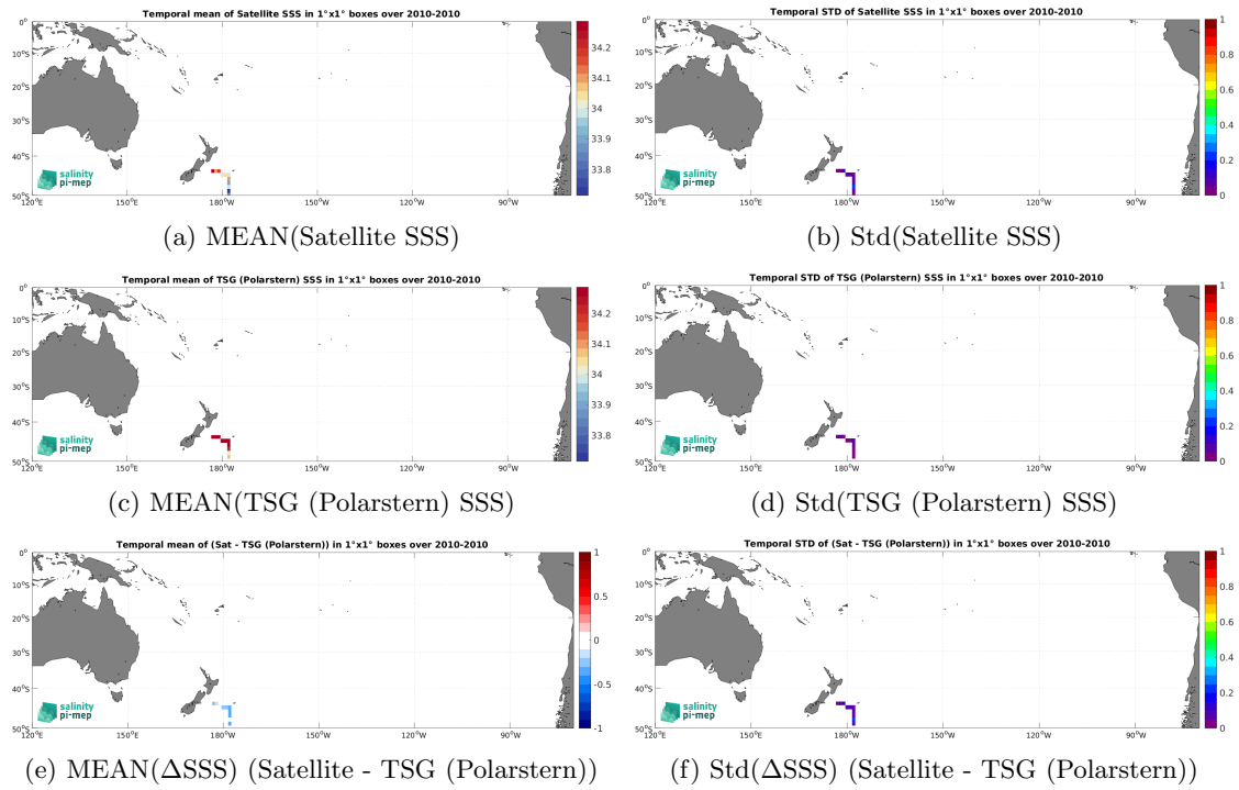
Figure 7: Temporal mean (left) and Std (right) of SSS from SMOS SSS L3 v332 - 9 Days (CATDS-CPDC) (top), TSG (Polarstern) (middle), and of \Delta SSS (Satellite - TSG (Polarstern)). Only match-up pairs are used to generate these maps.
