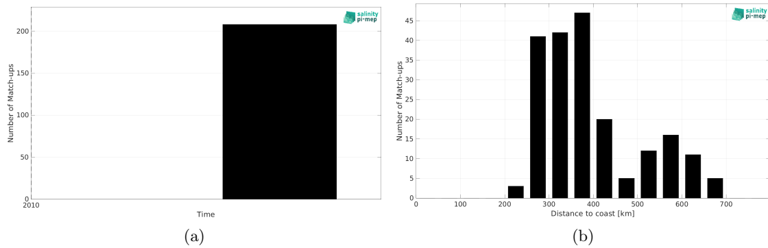
Figure 2: Number of match-ups between TSG (Polarstern) and SMOS SSS L3 v332 - 9 Days (CATDS-CPDC) SSS as a function of time (a) and as function of the distance to coast (b) over the South Pacific Ocean Pi-MEP region and for the full satellite product period.
