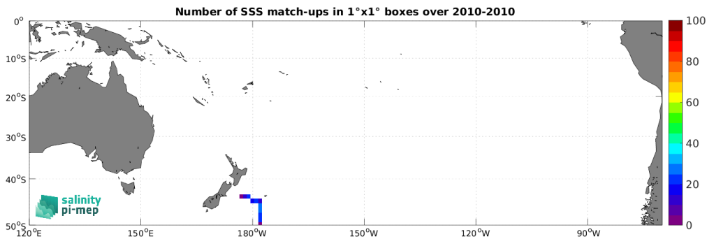
Figure 5: Number of SSS match-ups between TSG (Polarstern) SSS and the SMOS SSS L3 v332 - 9 Days (CATDS-CPDC) SSS product for the South Pacific Ocean Pi-MEP region over 1^\circ \times 1^\circ boxes and for the full satellite product period.
