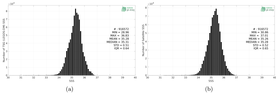
Figure 2: Histograms of SSS from TSG (LEGOS-DM) (a) and SMOS SSS L3 v332 - 9 Days (CATDS-CPDC) (b) considering all match-up pairs per bins of 0.1 over the South Pacific Ocean Pi-MEP region and for the full satellite product period.
