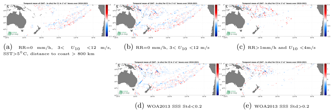
Figure 12: Temporal mean gridded over spatial boxes of size 1^\circ \times 1^\circ of \Delta SSS (SMOS SSS L3 v332 - 9 Days (CATDS-CPDC) - TSG (LEGOS-DM)) for 5 different subdatasets corresponding to:RR=0 mm/h, 3 < U_{10} < 12 m/s, SST >5^\circ C, distance to coast > 800 km (a), RR=0 mm/h, 3 < U_{10} < 12 m/s (b), RR >1 mm/h and U_{10} < 4 m/s (c), WOA2013 SSS Std <0.2 (d), WOA2013 SSS Std >0.2 (e).
