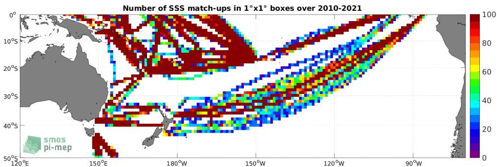
Figure 4: Number of SSS match-ups between TSG (LEGOS-DM) SSS and the SMOS SSS L3 v332 - 9 Days (CATDS-CPDC) SSS product for the South Pacific Ocean Pi-MEP region over 1^\circ \times 1^\circ boxes and for the full satellite product period.
