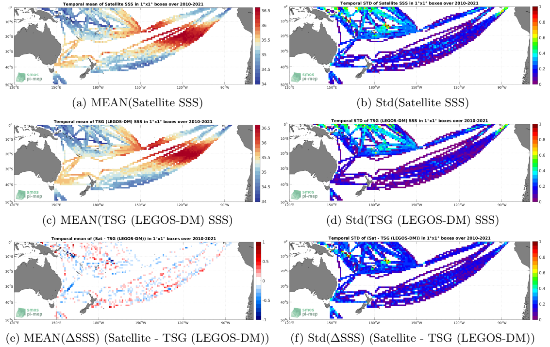
Figure 6: Temporal mean (left) and Std (right) of SSS from SMOS SSS L3 v332 - 9 Days (CATDS-CPDC) (top), TSG (LEGOS-DM) (middle), and of \Delta SSS (Satellite - TSG (LEGOS-DM)). Only match-up pairs are used to generate these maps.
