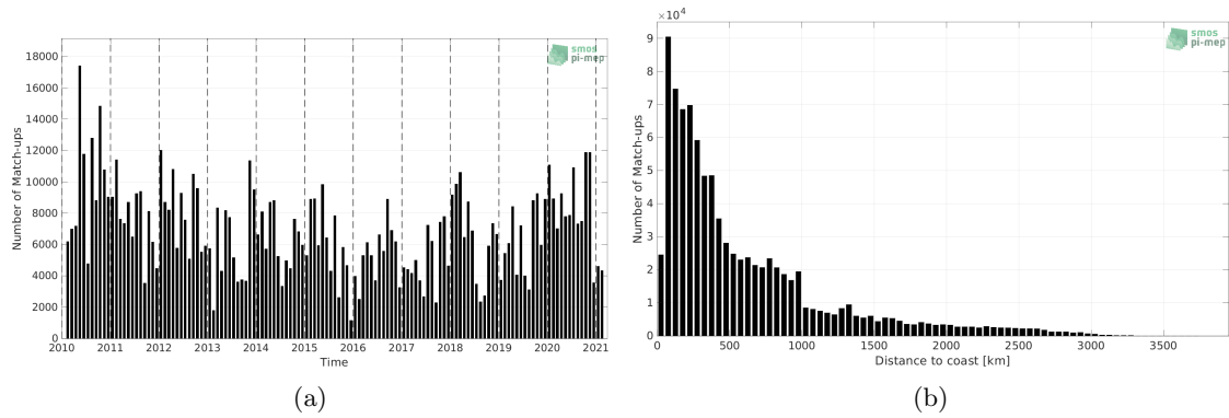
Figure 1: Number of match-ups between TSG (LEGOS-DM) and SMOS SSS L3 v332 - 9 Days (CATDS-CPDC) SSS as a function of time (a) and as function of the distance to coast (b) over the South Pacific Ocean Pi-MEP region and for the full satellite product period.
