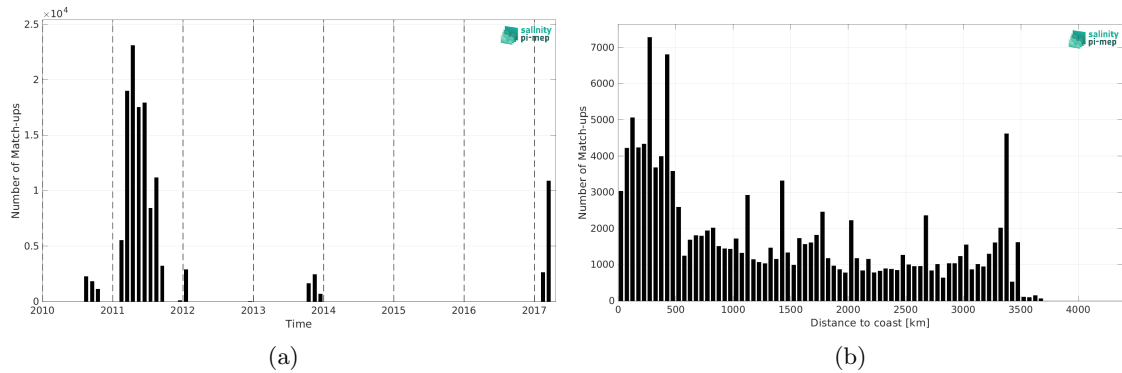
Figure 1: Number of match-ups between TSG (GOSUD-Sailing-ship) and SMOS SSS L3 v332 - 9 Days (CATDS-CPDC) SSS as a function of time (a) and as function of the distance to coast (b) over the South Pacific Ocean Pi-MEP region and for the full satellite product period.
