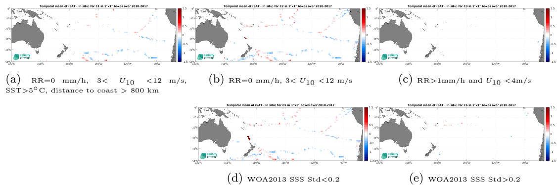
Figure 12: Temporal mean gridded over spatial boxes of size 1^\circ \times 1^\circ of \Delta\text{SSS} (SMOS SSS L3 v332 - 9 Days (CATDS-CPDC) - TSG (GOSUD-Sailing-ship)) for 5 different subdatasets corresponding to:RR=0 mm/h, 3 < U_{10} < 12 m/s, SST>5°C, distance to coast > 800 km (a), RR=0 mm/h, 3 < U_{10} < 12 m/s (b), RR>1mm/h and U_{10} < 4 m/s (c), WOA2013 SSS Std<0.2 (d), WOA2013 SSS Std>0.2 (e).
