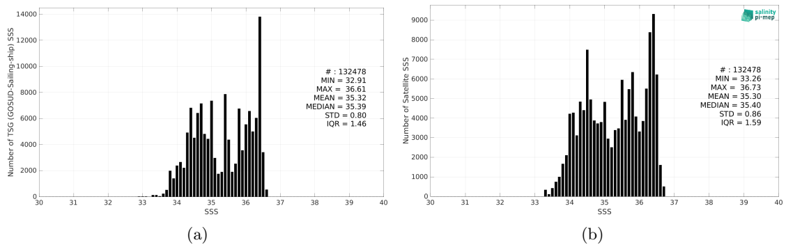
Figure 2: Histograms of SSS from TSG (GOSUD-Sailing-ship) (a) and SMOS SSS L3 v332 - 9 Days (CATDS-CPDC) (b) considering all match-up pairs per bins of 0.1 over the South Pacific Ocean Pi-MEP region and for the full satellite product period.
