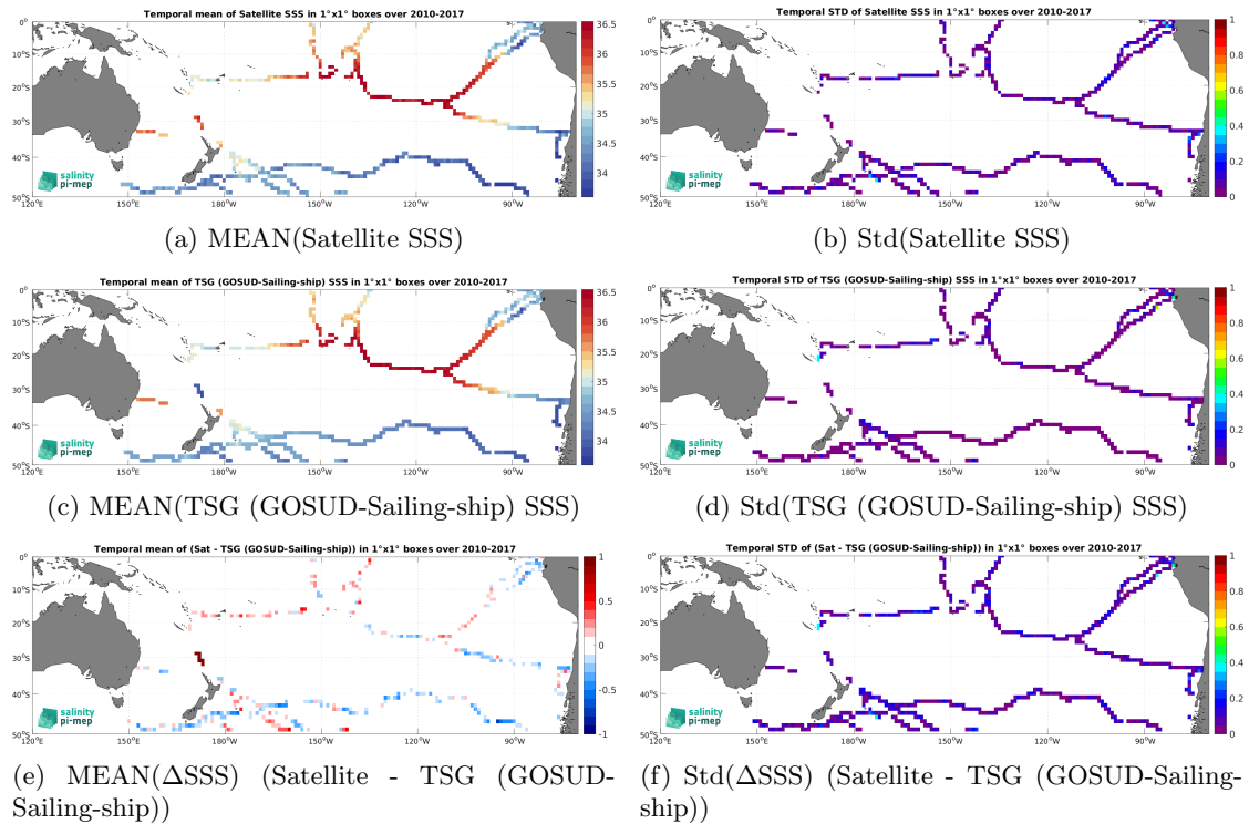
Figure 6: Temporal mean (left) and Std (right) of SSS from SMOS SSS L3 v332 - 9 Days (CATDS-CPDC) (top), TSG (GOSUD-Sailing-ship) (middle), and of \Delta SSS (Satellite - TSG (GOSUD-Sailing-ship)). Only match-up pairs are used to generate these maps.
