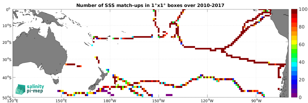
Figure 4: Number of SSS match-ups between TSG (GOSUD-Sailing-ship) SSS and the SMOS SSS L3 v332 - 9 Days (CATDS-CPDC) SSS product for the South Pacific Ocean Pi-MEP region over 1^\circ \times 1^\circ boxes and for the full satellite product period.
