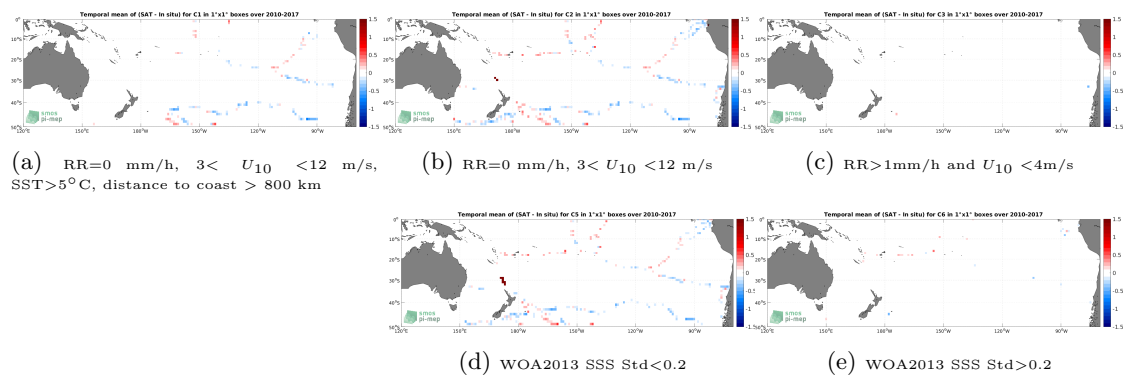
Figure 12: Temporal mean gridded over spatial boxes of size 1^\circ \times 1^\circ of \Delta SSS (SMOS SSS L3 v332 - 9 Days (CATDS-CPDC) - TSG (GOSUD-Sailing-ship)) for 5 different subdatasets corresponding to:RR=0 mm/h, 3 < U_{10} < 12 m/s, SST >5^\circ C, distance to coast > 800 km (a), RR=0 mm/h, 3 < U_{10} < 12 m/s (b), RR >1 mm/h and U_{10} < 4 m/s (c), WOA2013 SSS Std <0.2 (d), WOA2013 SSS Std >0.2 (e).
