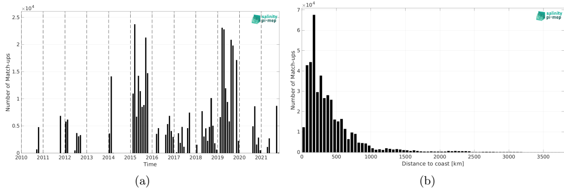
Figure 2: Number of match-ups between TSG (GOSUD-Research-vessel) and SMOS SSS L3 v332 - 9 Days (CATDS-CPDC) SSS as a function of time (a) and as function of the distance to coast (b) over the South Pacific Ocean Pi-MEP region and for the full satellite product period.
