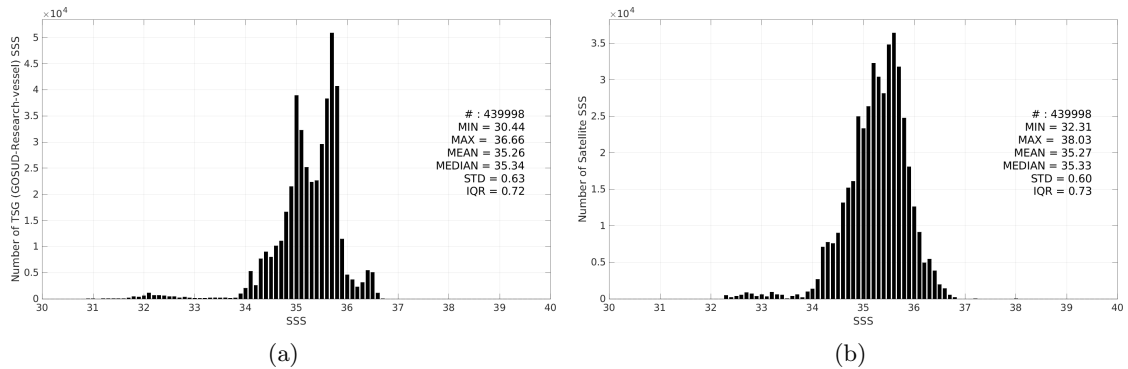
Figure 3: Histograms of SSS from TSG (GOSUD-Research-vessel) (a) and SMOS SSS L3 v332 - 9 Days (CATDS-CPDC) (b) considering all match-up pairs per bins of 0.1 over the South Pacific Ocean Pi-MEP region and for the full satellite product period.
