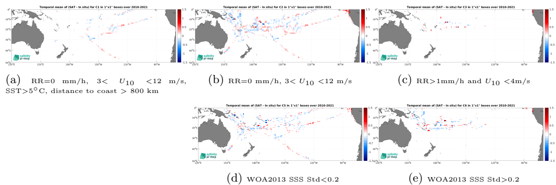
Figure 14: Temporal mean gridded over spatial boxes of size 1^\circ \times 1^\circ of \Delta SSS (SMOS SSS L3 v332 - 9 Days (CATDS-CPDC) - TSG (GOSUD-Research-vessel)) for 5 different subdatasets corresponding to:RR=0 mm/h, 3 < U_{10} < 12 m/s, SST >5^\circ C, distance to coast > 800 km (a), RR=0 mm/h, 3 < U_{10} < 12 m/s (b), RR >1 mm/h and U_{10} < 4 m/s (c), WOA2013 SSS Std <0.2 (d), WOA2013 SSS Std >0.2 (e).
