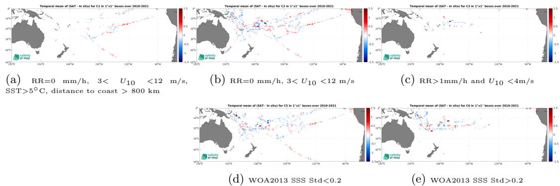
Figure 12: Temporal mean gridded over spatial boxes of size 1^\circ \times 1^\circ of \Delta\text{SSS} (SMOS SSS L3 v332 - 9 Days (CATDS-CPDC) - TSG (GOSUD-Research-vessel)) for 5 different subdatasets corresponding to:RR=0 mm/h, 3 < U_{10} < 12 m/s, SST>5°C, distance to coast > 800 km (a), RR=0 mm/h, 3 < U_{10} < 12 m/s (b), RR>1mm/h and U_{10} < 4 m/s (c), WOA2013 SSS Std<0.2 (d), WOA2013 SSS Std>0.2 (e).
