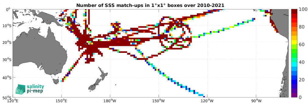
Figure 4: Number of SSS match-ups between TSG (GOSUD-Research-vessel) SSS and the SMOS SSS L3 v332 - 9 Days (CATDS-CPDC) SSS product for the South Pacific Ocean Pi-MEP region over 1^\circ \times 1^\circ boxes and for the full satellite product period.
