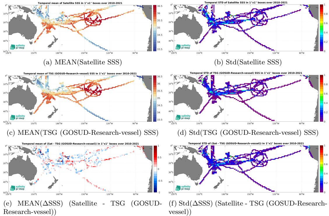
Figure 6: Temporal mean (left) and Std (right) of SSS from SMOS SSS L3 v332 - 9 Days (CATDS-CPDC) (top), TSG (GOSUD-Research-vessel) (middle), and of \Delta SSS (Satellite - TSG (GOSUD-Research-vessel)). Only match-up pairs are used to generate these maps.
