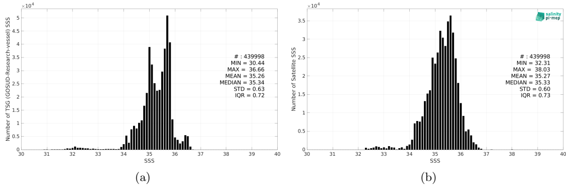
Figure 2: Histograms of SSS from TSG (GOSUD-Research-vessel) (a) and SMOS SSS L3 v332 - 9 Days (CATDS-CPDC) (b) considering all match-up pairs per bins of 0.1 over the South Pacific Ocean Pi-MEP region and for the full satellite product period.
