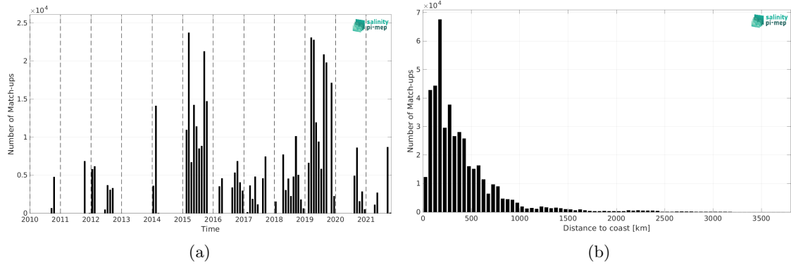
Figure 1: Number of match-ups between TSG (GOSUD-Research-vessel) and SMOS SSS L3 v332 - 9 Days (CATDS-CPDC) SSS as a function of time (a) and as function of the distance to coast (b) over the South Pacific Ocean Pi-MEP region and for the full satellite product period.
