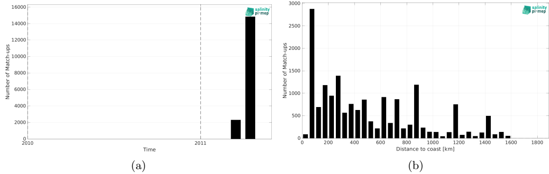
Figure 2: Number of match-ups between TSG (CSIC-UTM) and SMOS SSS L3 v332 - 9 Days (CATDS-CPDC) SSS as a function of time (a) and as function of the distance to coast (b) over the South Pacific Ocean Pi-MEP region and for the full satellite product period.
