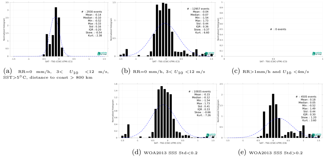
Figure 15: Normalized histogram of \Delta SSS (SMOS SSS L3 v332 - 9 Days (CATDS-CPDC) - TSG (CSIC-UTM)) for 5 different subdatasets corresponding to: RR=0 mm/h, 3 < U_{10} < 12 m/s, SST>5°C, distance to coast > 800 km (a), RR=0 mm/h, 3 < U_{10} < 12 m/s (b), RR>1mm/h and U_{10} < 4 m/s (c), WOA2013 SSS Std<0.2 (d), WOA2013 SSS Std>0.2 (e).
