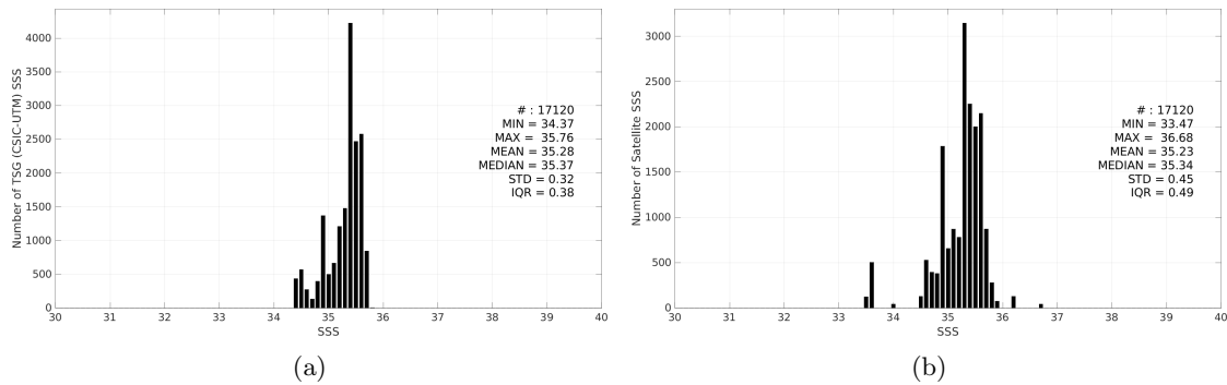
Figure 3: Histograms of SSS from TSG (CSIC-UTM) (a) and SMOS SSS L3 v332 - 9 Days (CATDS-CPDC) (b) considering all match-up pairs per bins of 0.1 over the South Pacific Ocean Pi-MEP region and for the full satellite product period.
