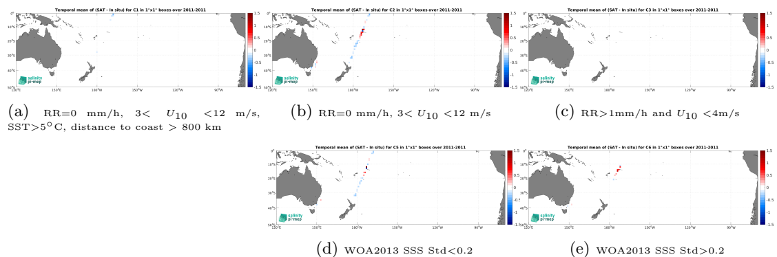
Figure 14: Temporal mean gridded over spatial boxes of size 1^\circ \times 1^\circ of \Delta SSS (SMOS SSS L3 v332 - 9 Days (CATDS-CPDC) - TSG (CSIC-UTM)) for 5 different subdatasets corresponding to: RR=0 mm/h, 3 < U_{10} < 12 m/s, SST > 5°C, distance to coast > 800 km (a), RR=0 mm/h, 3 < U_{10} < 12 m/s (b), RR > 1mm/h and U_{10} < 4 m/s (c), WOA2013 SSS Std < 0.2 (d), WOA2013 SSS Std > 0.2 (e).
