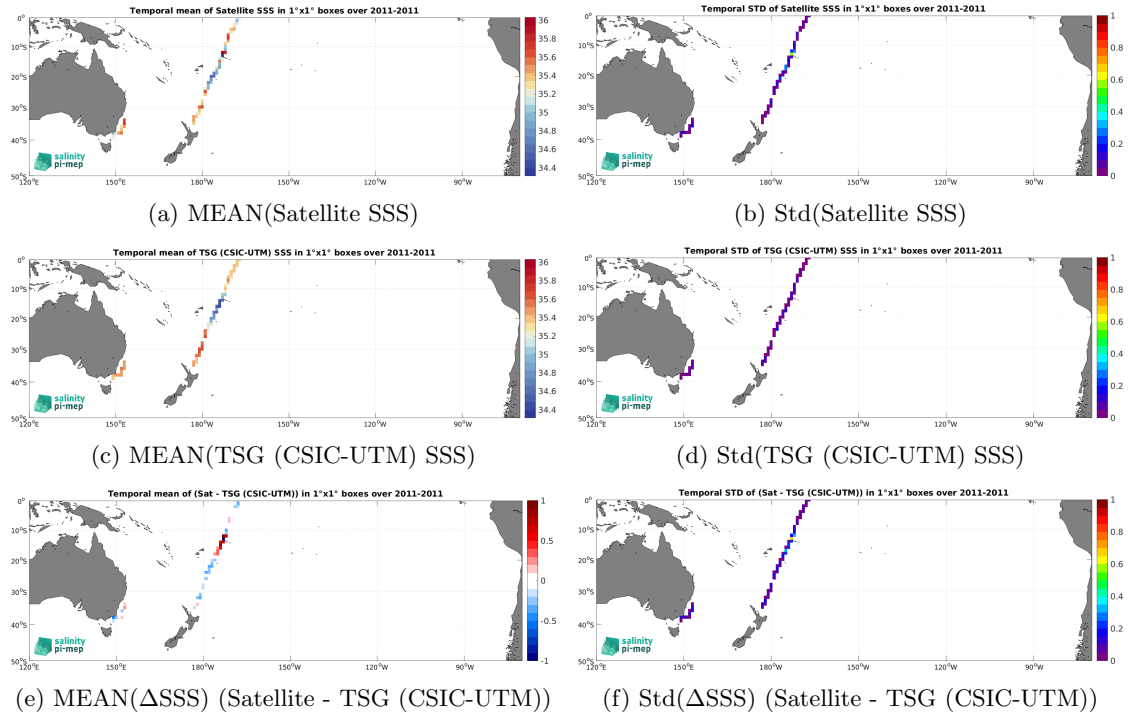
Figure 7: Temporal mean (left) and Std (right) of SSS from SMOS SSS L3 v332 - 9 Days (CATDS-CPDC) (top), TSG (CSIC-UTM) (middle), and of \Delta SSS (Satellite - TSG (CSIC-UTM)). Only match-up pairs are used to generate these maps.
