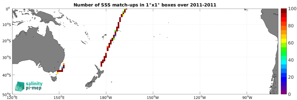
Figure 5: Number of SSS match-ups between TSG (CSIC-UTM) SSS and the SMOS SSS L3 v332 - 9 Days (CATDS-CPDC) SSS product for the South Pacific Ocean Pi-MEP region over 1^\circ \times 1^\circ boxes and for the full satellite product period.
