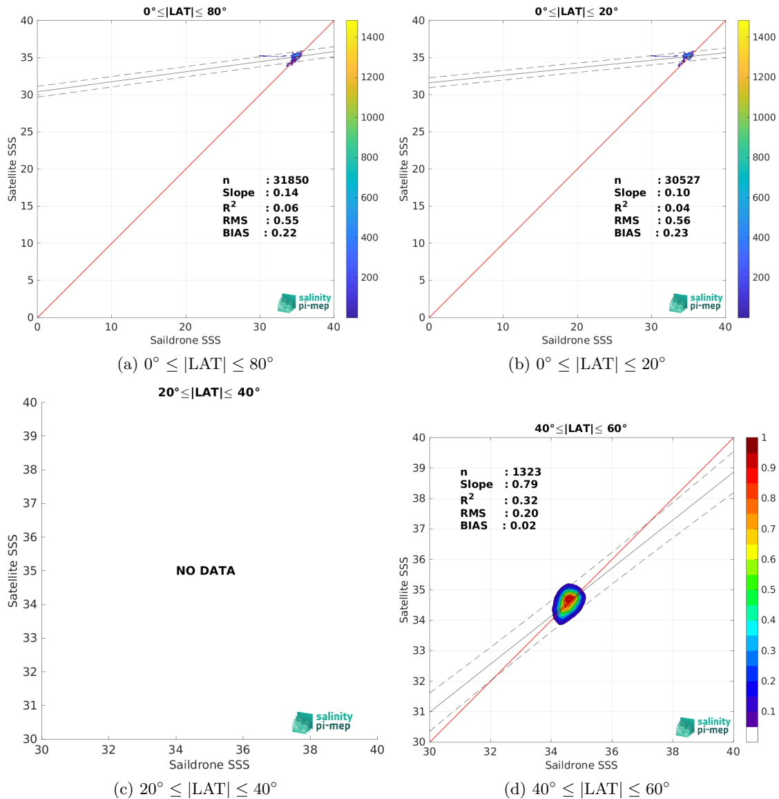
Figure 10: Contour maps of the concentration of SMOS SSS L3 v332 - 9 Days (CATDS-CPDC) SSS (y-axis) versus Sairdrone SSS (x-axis) at match-up pairs for different latitude bands. For each plot, the red line shows x=y . The black thin and dashed lines indicate a linear fit through the data cloud and the \pm 95\% confidence levels, respectively. The number match-up pairs n , the slope and R^2 coefficient of the linear fit, the root mean square (RMS) and the mean bias between satellite and in situ data are indicated for each latitude band in each plots.
