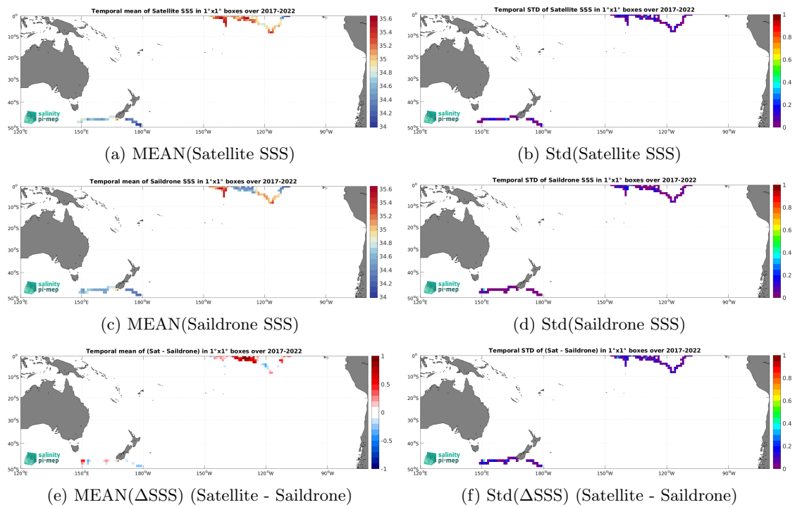
Figure 6: Temporal mean (left) and Std (right) of SSS from SMOS SSS L3 v332 - 9 Days (CATDS-CPDC) (top), Saildrone (middle), and of \Delta SSS (Satellite - Saildrone). Only match-up pairs are used to generate these maps.
