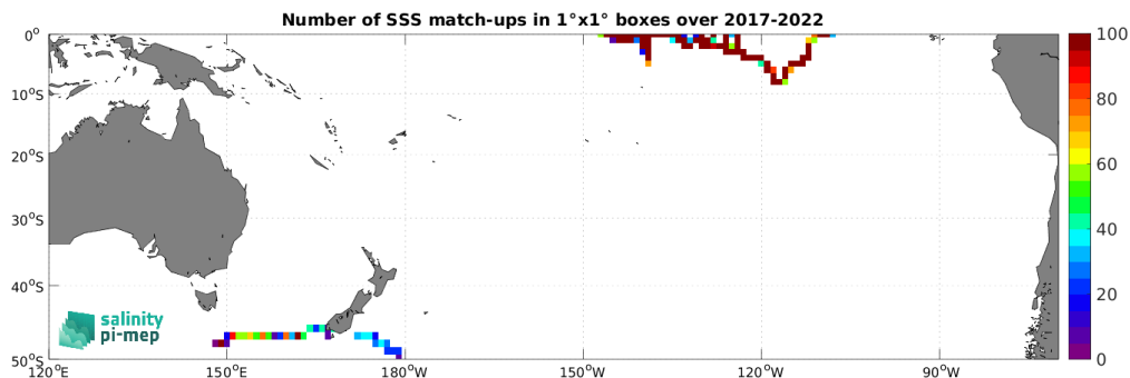
Figure 4: Number of SSS match-ups between Saildrone SSS and the SMOS SSS L3 v332 - 9 Days (CATDS-CPDC) SSS product for the South Pacific Ocean Pi-MEP region over 1^\circ \times 1^\circ boxes and for the full satellite product period.
