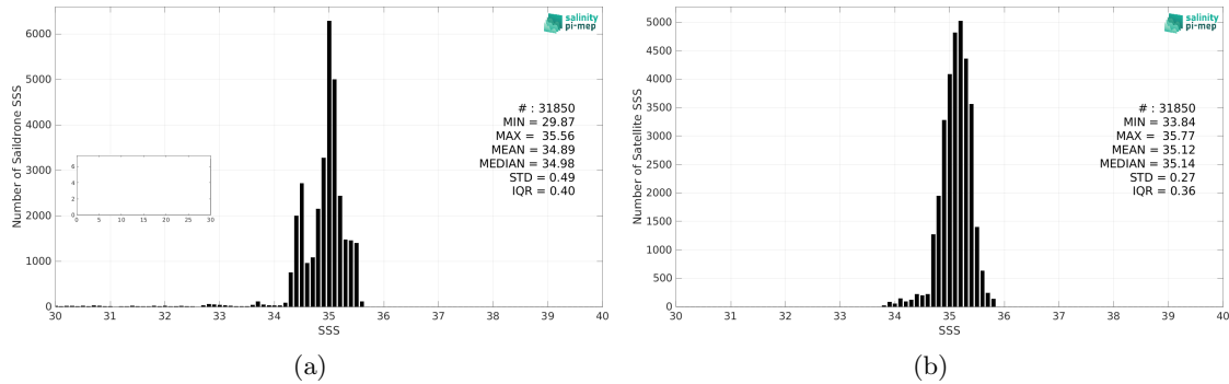
Figure 2: Histograms of SSS from Saildrone (a) and SMOS SSS L3 v332 - 9 Days (CATDS-CPDC) (b) considering all match-up pairs per bins of 0.1 over the South Pacific Ocean Pi-MEP region and for the full satellite product period.
