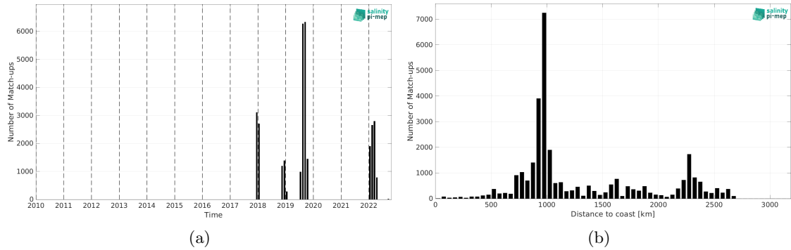
Figure 1: Number of match-ups between Saildrone and SMOS SSS L3 v332 - 9 Days (CATDS-CPDC) SSS as a function of time (a) and as function of the distance to coast (b) over the South Pacific Ocean Pi-MEP region and for the full satellite product period.
