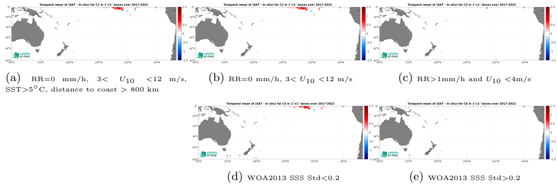
Figure 12: Temporal mean gridded over spatial boxes of size 1^\circ \times 1^\circ of \Delta SSS (SMOS SSS L3 v332 - 9 Days (CATDS-CPDC) - Sairdrone) for 5 different subdatasets corresponding to:RR=0 mm/h, 3 < U_{10} < 12 m/s, SST >5^\circ C, distance to coast > 800 km (a), RR=0 mm/h, 3 < U_{10} < 12 m/s (b), RR >1 mm/h and U_{10} < 4 m/s (c), WOA2013 SSS Std <0.2 (d), WOA2013 SSS Std >0.2 (e).
