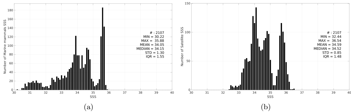
Figure 3: Histograms of SSS from Marine mammals (a) and SMOS SSS L3 v332 - 9 Days (CATDS-CPDC) (b) considering all match-up pairs per bins of 0.1 over the South Pacific Ocean Pi-MEP region and for the full satellite product period.
