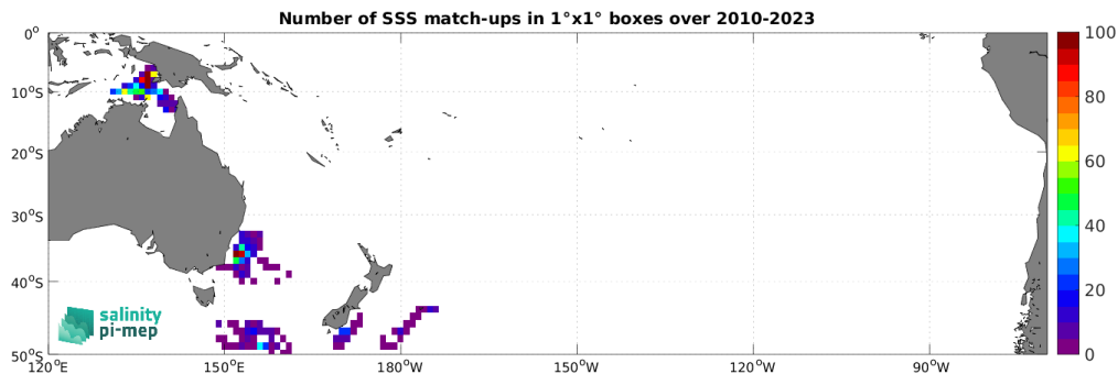
Figure 5: Number of SSS match-ups between Marine mammals SSS and the SMOS SSS L3 v332 - 9 Days (CATDS-CPDC) SSS product for the South Pacific Ocean Pi-MEP region over 1^\circ \times 1^\circ boxes and for the full satellite product period.
