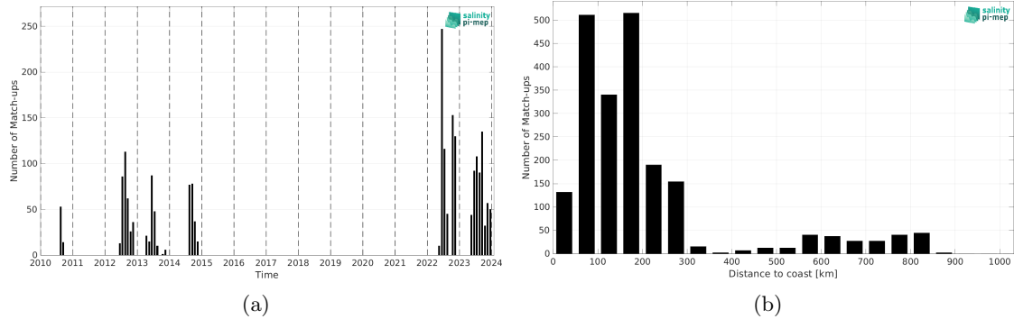
Figure 2: Number of match-ups between Marine mammals and SMOS SSS L3 v332 - 9 Days (CATDS-CPDC) SSS as a function of time (a) and as function of the distance to coast (b) over the South Pacific Ocean Pi-MEP region and for the full satellite product period.
