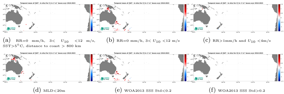
Figure 14: Temporal mean gridded over spatial boxes of size 1^\circ \times 1^\circ of \Delta SSS (SMOS SSS L3 v332 - 9 Days (CATDS-CPDC) - Marine mammals) for 6 different subdatasets corresponding to:RR=0 mm/h, 3 < U_{10} < 12 m/s, SST >5^\circ C, distance to coast > 800 km (a), RR=0 mm/h, 3 < U_{10} < 12 m/s (b), RR >1 mm/h and U_{10} < 4 m/s (c),MLD <20 m (d),WOA2013 SSS Std <0.2 (e),WOA2013 SSS Std >0.2 (f).
