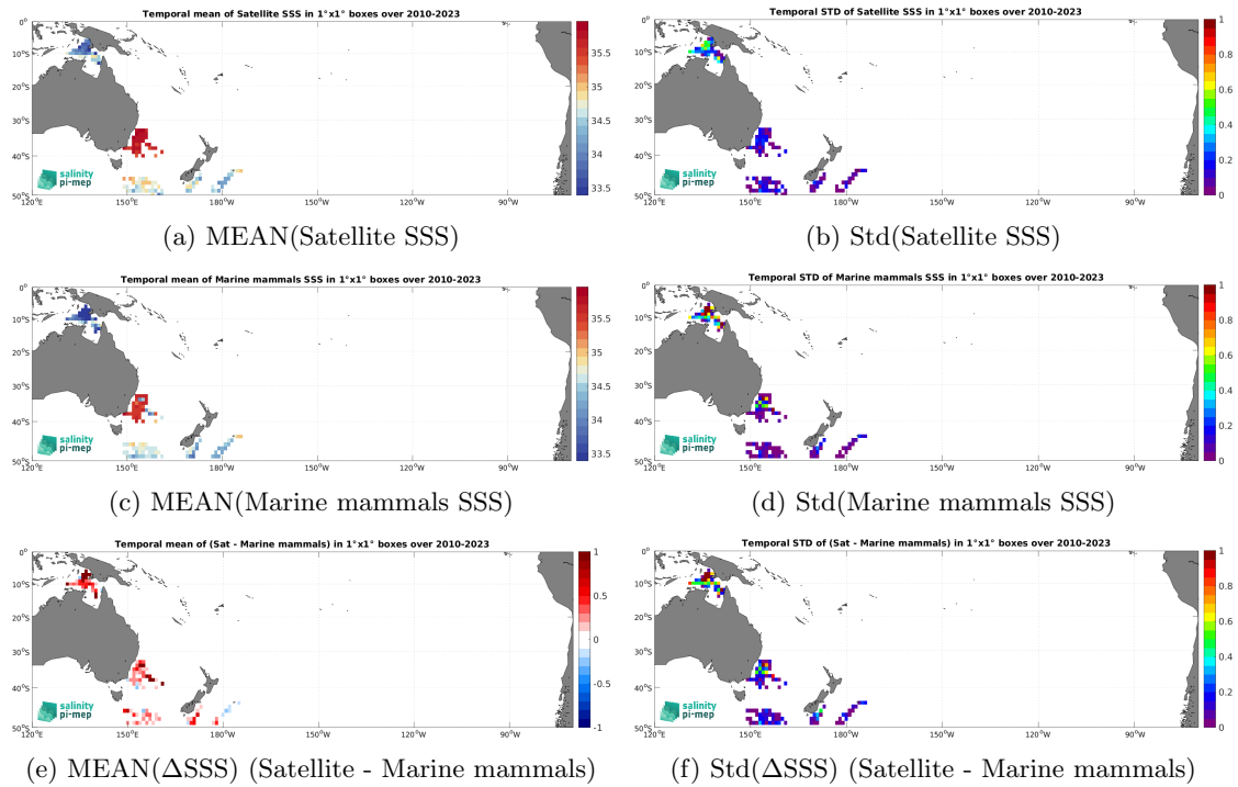
Figure 7: Temporal mean (left) and Std (right) of SSS from SMOS SSS L3 v332 - 9 Days (CATDS-CPDC) (top), Marine mammals (middle), and of \Delta SSS (Satellite - Marine mammals). Only match-up pairs are used to generate these maps.
