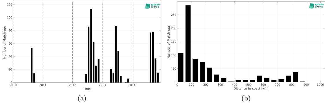
Figure 1: Number of match-ups between Marine mammals and SMOS SSS L3 v332 - 9 Days (CATDS-CPDC) SSS as a function of time (a) and as function of the distance to coast (b) over the South Pacific Ocean Pi-MEP region and for the full satellite product period.
