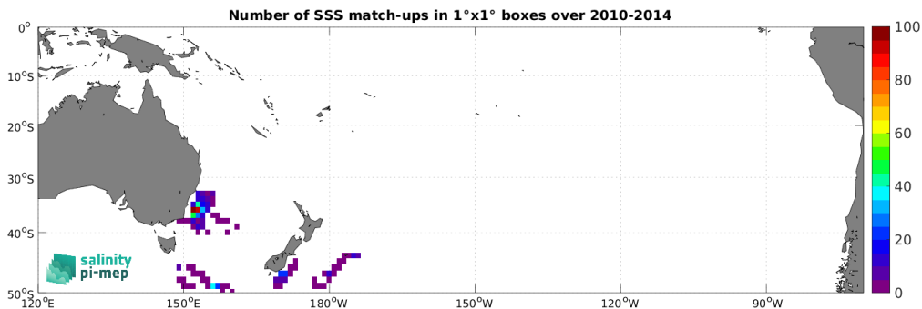
Figure 4: Number of SSS match-ups between Marine mammals SSS and the SMOS SSS L3 v332 - 9 Days (CATDS-CPDC) SSS product for the South Pacific Ocean Pi-MEP region over 1^\circ \times 1^\circ boxes and for the full satellite product period.
