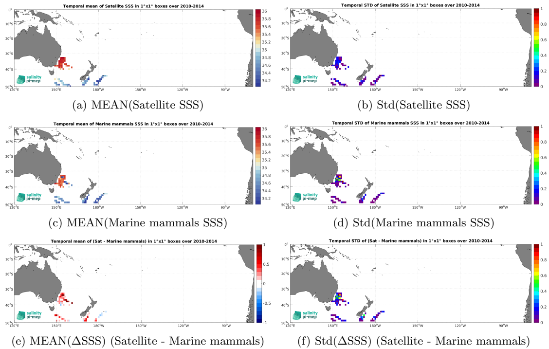
Figure 6: Temporal mean (left) and Std (right) of SSS from SMOS SSS L3 v332 - 9 Days (CATDS-CPDC) (top), Marine mammals (middle), and of \Delta SSS (Satellite - Marine mammals). Only match-up pairs are used to generate these maps.
