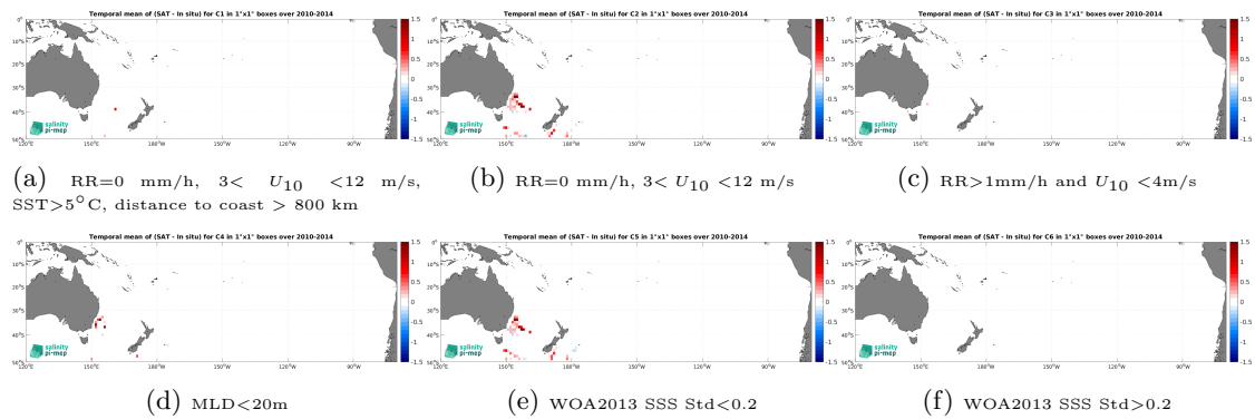
Figure 12: Temporal mean gridded over spatial boxes of size 1^\circ \times 1^\circ of \Delta SSS (SMOS SSS L3 v332 - 9 Days (CATDS-CPDC) - Marine mammals) for 6 different subdatasets corresponding to:RR=0 mm/h, 3 < U_{10} < 12 m/s, SST > 5^\circ\text{C} , distance to coast > 800 km (a), RR=0 mm/h, 3 < U_{10} < 12 m/s (b), RR > 1 mm/h and U_{10} < 4 m/s (c),MLD < 20 m (d),WOA2013 SSS Std < 0.2 (e),WOA2013 SSS Std > 0.2 (f).
