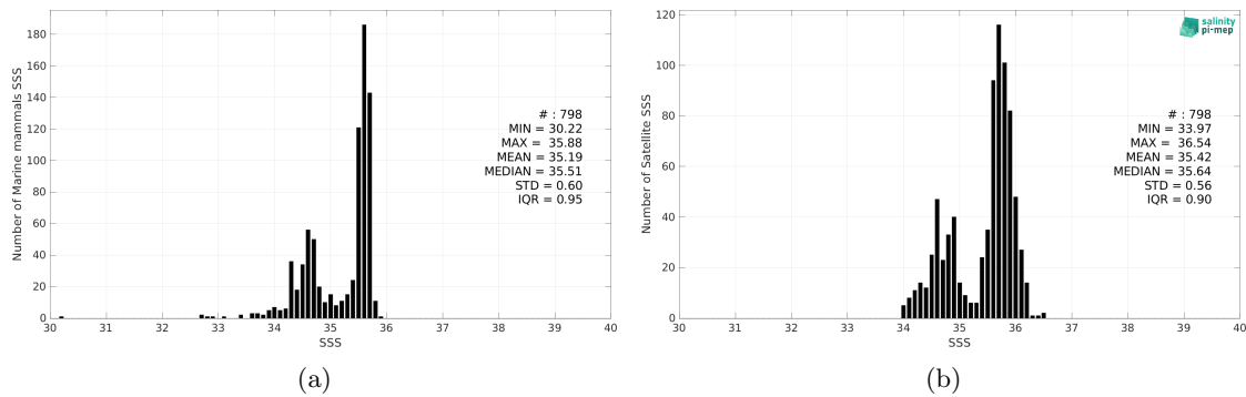
Figure 2: Histograms of SSS from Marine mammals (a) and SMOS SSS L3 v332 - 9 Days (CATDS-CPDC) (b) considering all match-up pairs per bins of 0.1 over the South Pacific Ocean Pi-MEP region and for the full satellite product period.
