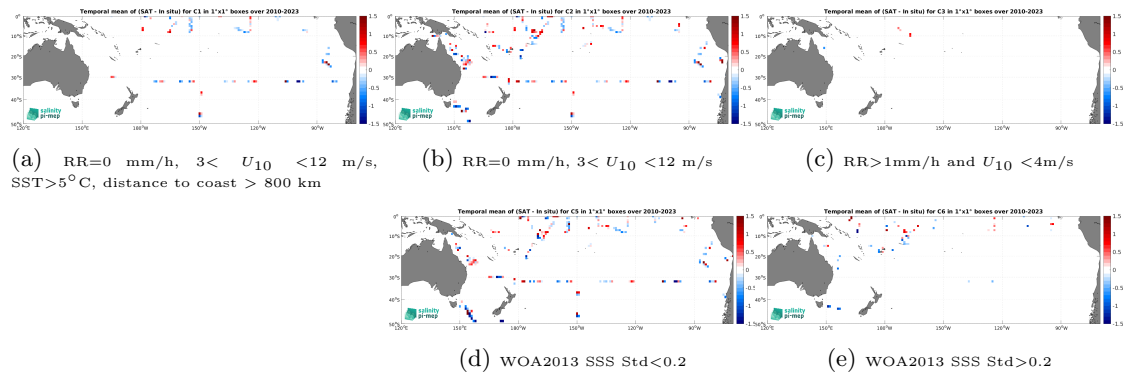
Figure 12: Temporal mean gridded over spatial boxes of size 1^\circ \times 1^\circ of \Delta\text{SSS} (SMOS SSS L2Q v331 - 0.25 Deg (CATDS-CPDC) - TSG (SAMOS)) for 5 different subdatasets corresponding to:RR=0 mm/h, 3 < U_{10} < 12 m/s, SST >5^\circ\text{C} , distance to coast > 800 km (a), RR=0 mm/h, 3 < U_{10} < 12 m/s (b), RR >1 mm/h and U_{10} < 4 m/s (c), WOA2013 SSS Std <0.2 (d), WOA2013 SSS Std >0.2 (e).
