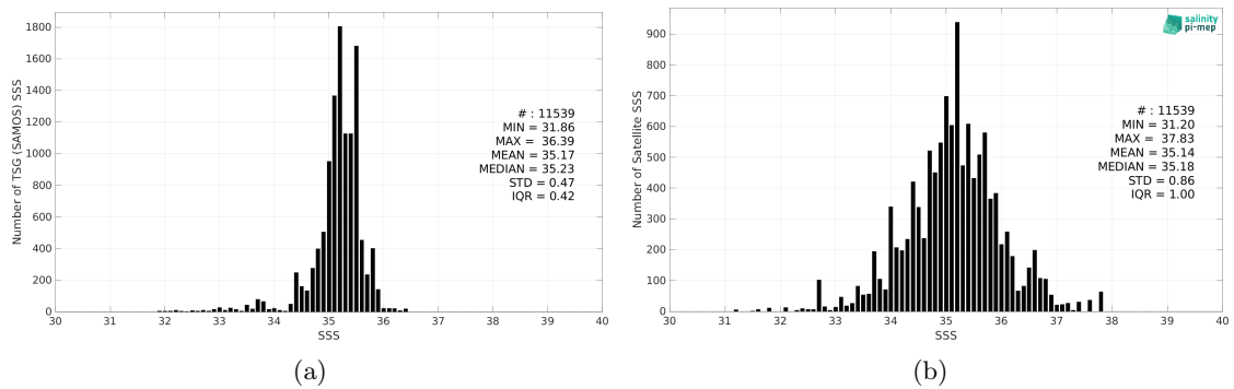
Figure 2: Histograms of SSS from TSG (SAMOS) (a) and SMOS SSS L2Q v331 - 0.25 Deg (CATDS-CPDC) (b) considering all match-up pairs per bins of 0.1 over the South Pacific Ocean Pi-MEP region and for the full satellite product period.
