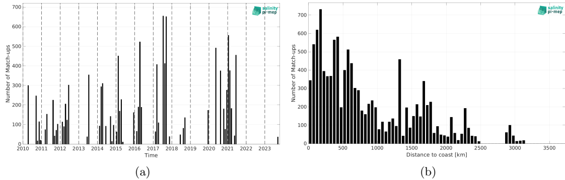
Figure 1: Number of match-ups between TSG (SAMOS) and SMOS SSS L2Q v331 - 0.25 Deg (CATDS-CPDC) SSS as a function of time (a) and as function of the distance to coast (b) over the South Pacific Ocean Pi-MEP region and for the full satellite product period.
