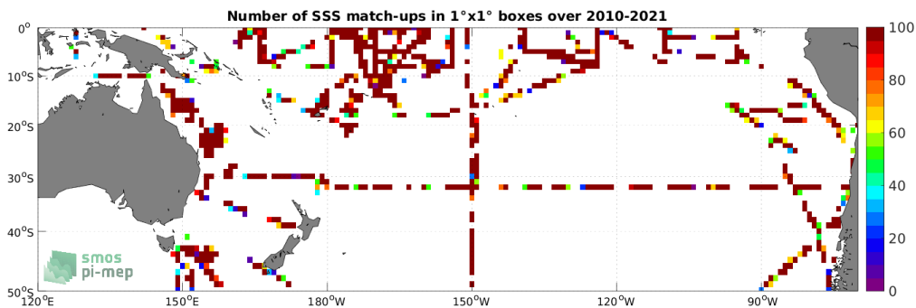
Figure 4: Number of SSS match-ups between TSG (SAMOS) SSS and the SMOS SSS L2Q v331 - 0.25 Deg (CATDS-CPDC) SSS product for the South Pacific Ocean Pi-MEP region over 1^\circ \times 1^\circ boxes and for the full satellite product period.
