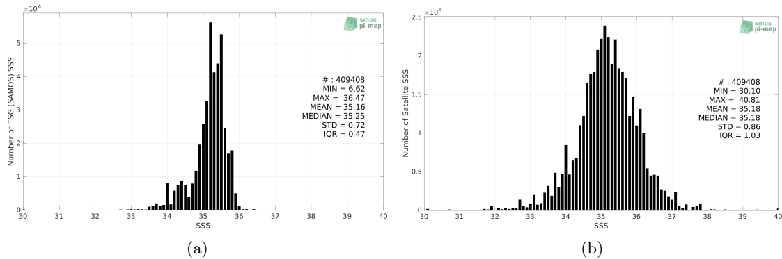
Figure 2: Histograms of SSS from TSG (SAMOS) (a) and SMOS SSS L2Q v331 - 0.25 Deg (CATDS-CPDC) (b) considering all match-up pairs per bins of 0.1 over the South Pacific Ocean Pi-MEP region and for the full satellite product period.
