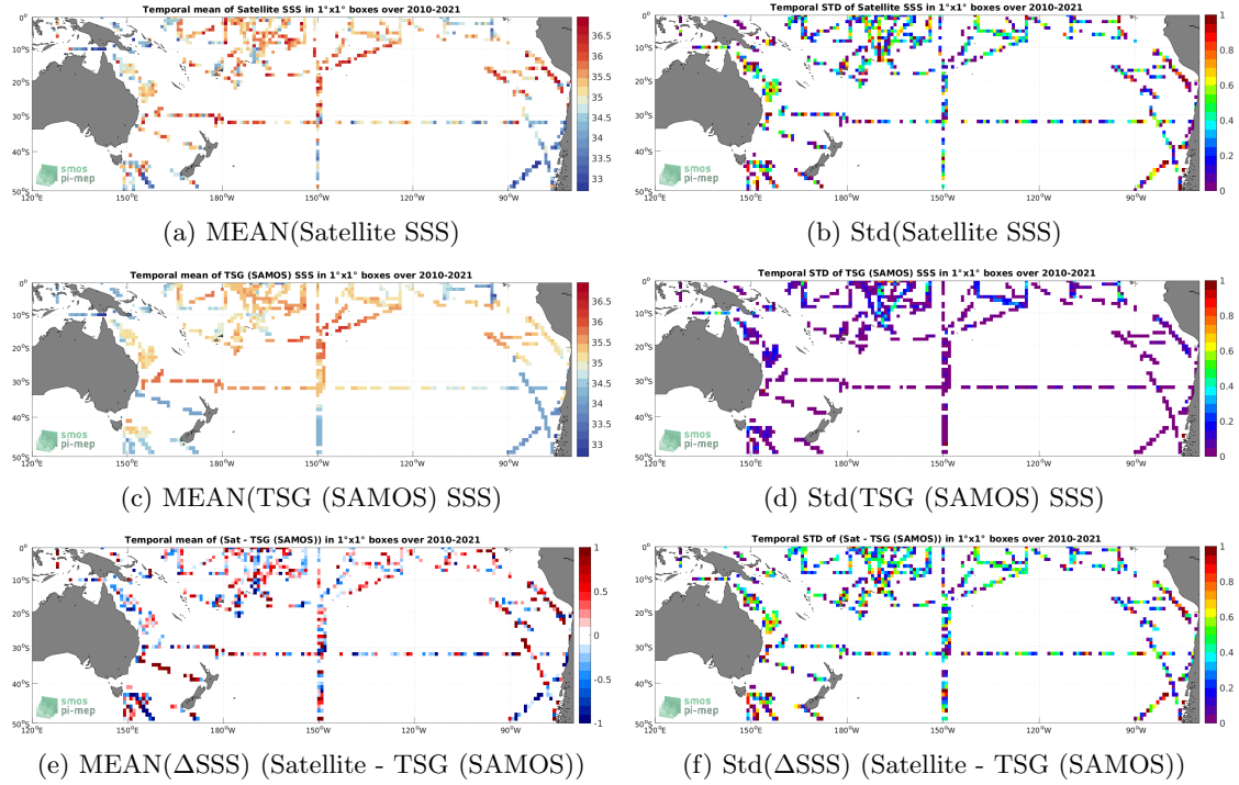
Figure 6: Temporal mean (left) and Std (right) of SSS from SMOS SSS L2Q v331 - 0.25 Deg (CATDS-CPDC) (top), TSG (SAMOS) (middle), and of \Delta SSS (Satellite - TSG (SAMOS)). Only match-up pairs are used to generate these maps.
