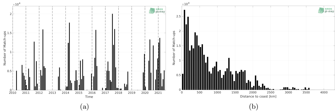
Figure 1: Number of match-ups between TSG (SAMOS) and SMOS SSS L2Q v331 - 0.25 Deg (CATDS-CPDC) SSS as a function of time (a) and as function of the distance to coast (b) over the South Pacific Ocean Pi-MEP region and for the full satellite product period.
