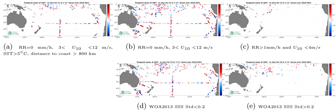
Figure 12: Temporal mean gridded over spatial boxes of size 1^\circ \times 1^\circ of \Delta SSS (SMOS SSS L2Q v331 - 0.25 Deg (CATDS-CPDC) - TSG (SAMOS)) for 5 different subdatasets corresponding to:RR=0 mm/h, 3 < U_{10} < 12 m/s, SST >5^\circ\text{C} , distance to coast > 800 km (a), RR=0 mm/h, 3 < U_{10} < 12 m/s (b), RR >1 mm/h and U_{10} < 4 m/s (c), WOA2013 SSS Std <0.2 (d), WOA2013 SSS Std >0.2 (e).
