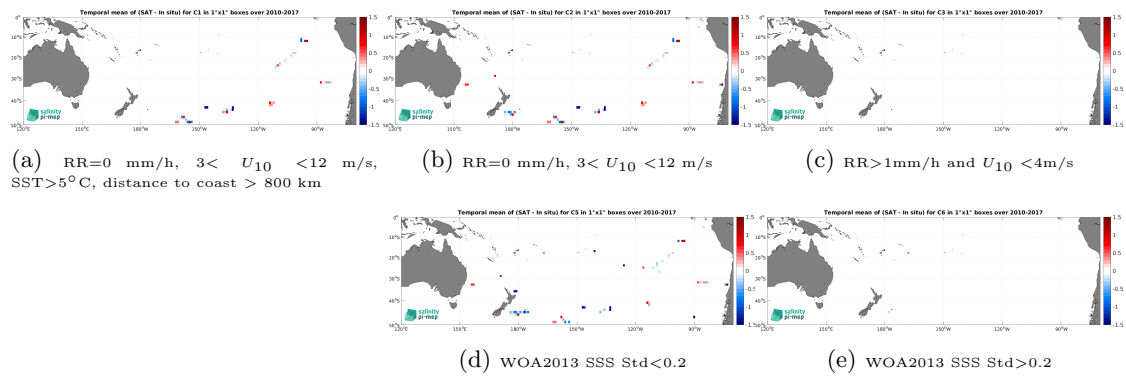
Figure 12: Temporal mean gridded over spatial boxes of size 1^\circ \times 1^\circ of \Delta SSS (SMOS SSS L2Q v331 - 0.25 Deg (CATDS-CPDC) - TSG (GOSUD-Sailing-ship)) for 5 different subdatasets corresponding to:RR=0 mm/h, 3 < U_{10} < 12 m/s, SST>5°C, distance to coast > 800 km (a), RR=0 mm/h, 3 < U_{10} < 12 m/s (b), RR>1mm/h and U_{10} < 4 m/s (c), WOA2013 SSS Std<0.2 (d), WOA2013 SSS Std>0.2 (e).
