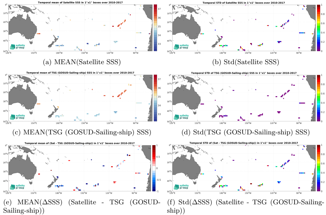
Figure 6: Temporal mean (left) and Std (right) of SSS from SMOS SSS L2Q v331 - 0.25 Deg (CATDS-CPDC) (top), TSG (GOSUD-Sailing-ship) (middle), and of \Delta SSS (Satellite - TSG (GOSUD-Sailing-ship)). Only match-up pairs are used to generate these maps.
