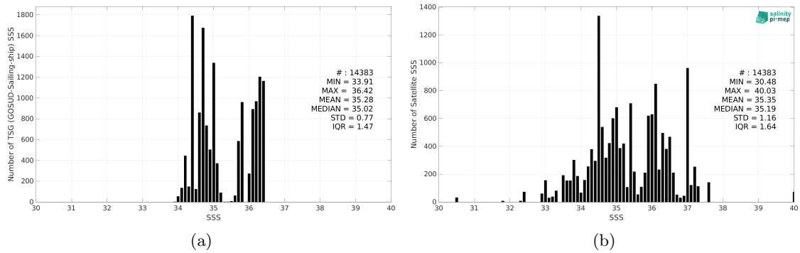
Figure 2: Histograms of SSS from TSG (GOSUD-Sailing-ship) (a) and SMOS SSS L2Q v331 - 0.25 Deg (CATDS-CPDC) (b) considering all match-up pairs per bins of 0.1 over the South Pacific Ocean Pi-MEP region and for the full satellite product period.
