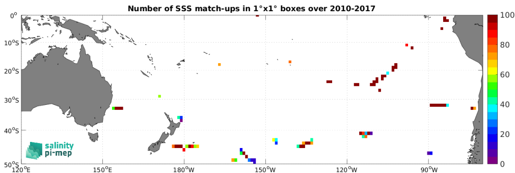
Figure 4: Number of SSS match-ups between TSG (GOSUD-Sailing-ship) SSS and the SMOS SSS L2Q v331 - 0.25 Deg (CATDS-CPDC) SSS product for the South Pacific Ocean Pi-MEP region over 1^\circ \times 1^\circ boxes and for the full satellite product period.
