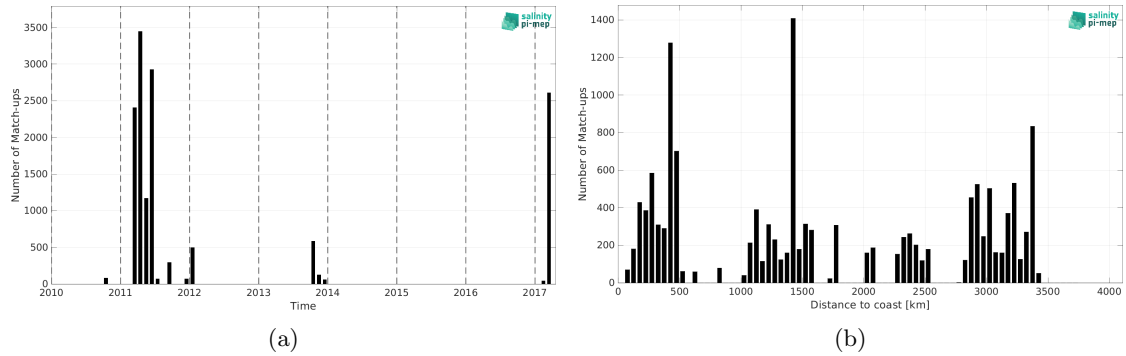
Figure 1: Number of match-ups between TSG (GOSUD-Sailing-ship) and SMOS SSS L2Q v331 - 0.25 Deg (CATDS-CPDC) SSS as a function of time (a) and as function of the distance to coast (b) over the South Pacific Ocean Pi-MEP region and for the full satellite product period.
