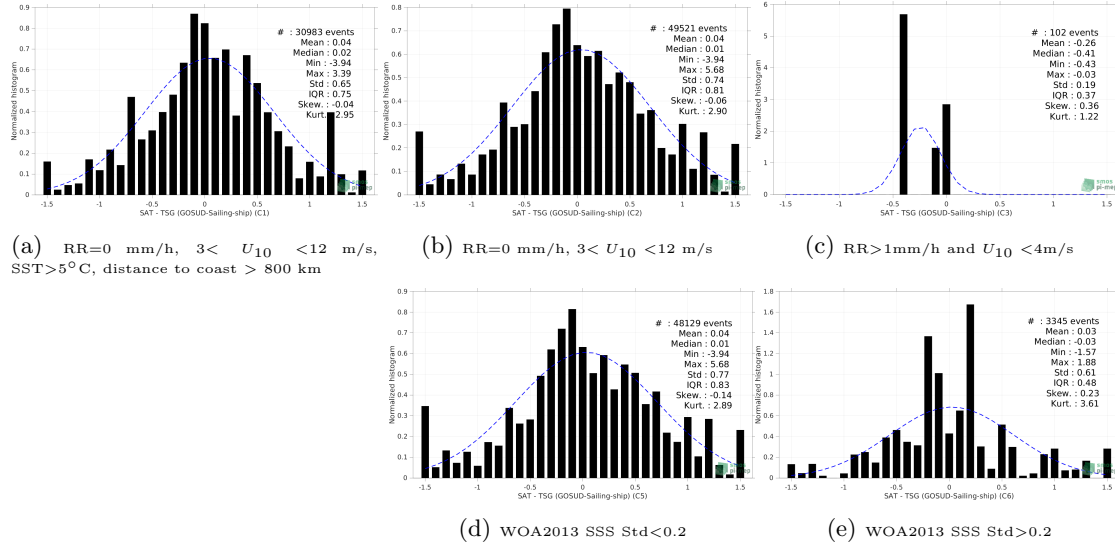
Figure 13: Normalized histogram of \Delta SSS (SMOS SSS L2Q v331 - 0.25 Deg (CATDS-CPDC) - TSG (GOSUD-Sailing-ship)) for 5 different subdatasets corresponding to: RR=0 mm/h, 3 < U_{10} < 12 m/s, SST>5°C, distance to coast > 800 km (a), RR=0 mm/h, 3 < U_{10} < 12 m/s (b), RR>1mm/h and U_{10} < 4 m/s (c), WOA2013 SSS Std<0.2 (d), WOA2013 SSS Std>0.2 (e).
