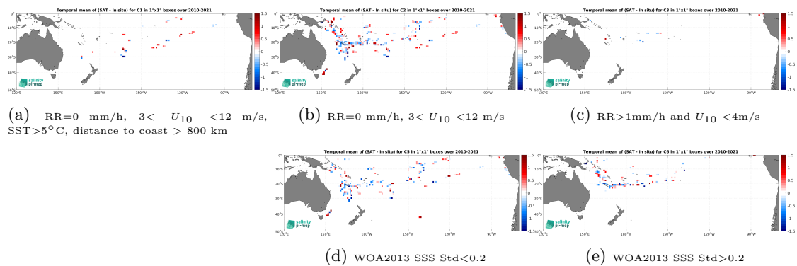
Figure 12: Temporal mean gridded over spatial boxes of size 1^\circ \times 1^\circ of \Delta\text{SSS} (SMOS SSS L2Q v331 - 0.25 Deg (CATDS-CPDC) - TSG (GOSUD-Research-vessel)) for 5 different subdatasets corresponding to:RR=0 mm/h, 3 < U_{10} < 12 m/s, SST>5°C, distance to coast > 800 km (a), RR=0 mm/h, 3 < U_{10} < 12 m/s (b), RR>1mm/h and U_{10} < 4 m/s (c), WOA2013 SSS Std<0.2 (d), WOA2013 SSS Std>0.2 (e).
