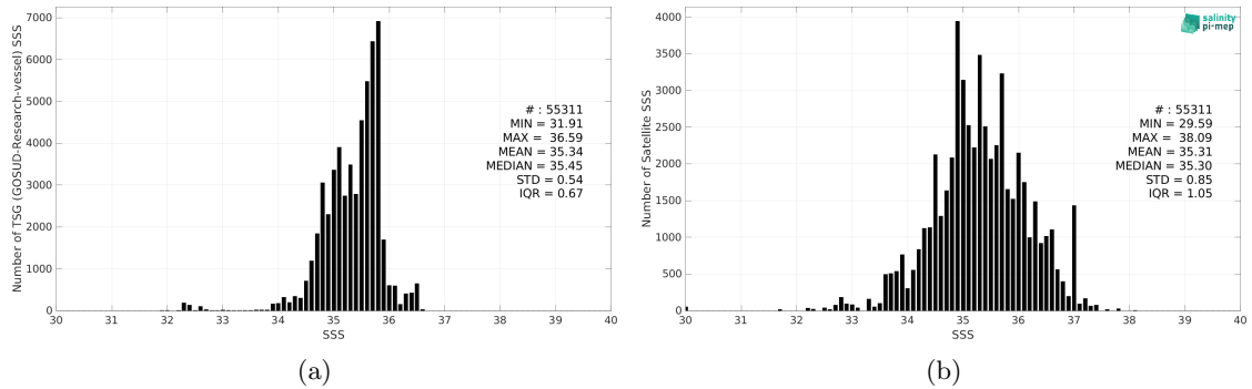
Figure 2: Histograms of SSS from TSG (GOSUD-Research-vessel) (a) and SMOS SSS L2Q v331 - 0.25 Deg (CATDS-CPDC) (b) considering all match-up pairs per bins of 0.1 over the South Pacific Ocean Pi-MEP region and for the full satellite product period.
