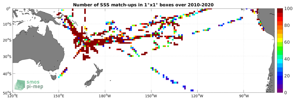
Figure 4: Number of SSS match-ups between TSG (GOSUD-Research-vessel) SSS and the SMOS SSS L2Q v331 - 0.25 Deg (CATDS-CPDC) SSS product for the South Pacific Ocean Pi-MEP region over 1^\circ \times 1^\circ boxes and for the full satellite product period.
