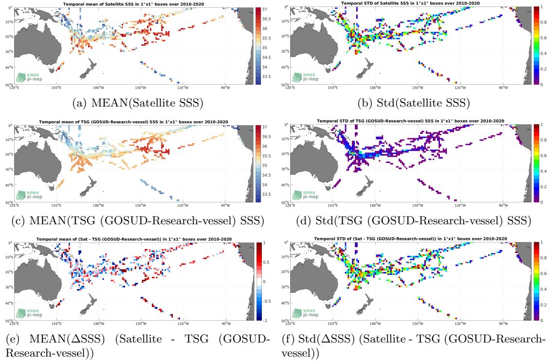
Figure 6: Temporal mean (left) and Std (right) of SSS from SMOS SSS L2Q v331 - 0.25 Deg (CATDS-CPDC) (top), TSG (GOSUD-Research-vessel) (middle), and of \Delta SSS (Satellite - TSG (GOSUD-Research-vessel)). Only match-up pairs are used to generate these maps.
