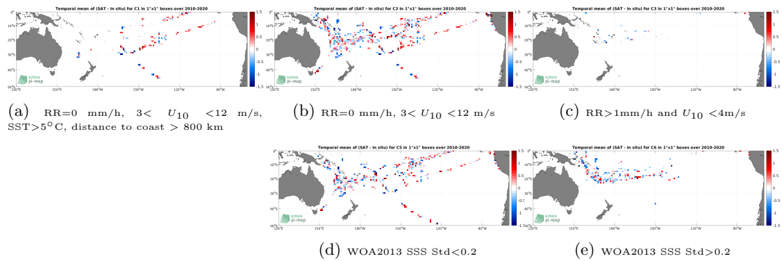
Figure 12: Temporal mean gridded over spatial boxes of size 1^\circ \times 1^\circ of \Delta SSS (SMOS SSS L2Q v331 - 0.25 Deg (CATDS-CPDC) - TSG (GOSUD-Research-vessel)) for 5 different subdatasets corresponding to:RR=0 mm/h, 3 < U_{10} < 12 m/s, SST >5^\circ\text{C} , distance to coast > 800 km (a), RR=0 mm/h, 3 < U_{10} < 12 m/s (b), RR >1 mm/h and U_{10} < 4 m/s (c), WOA2013 SSS Std <0.2 (d), WOA2013 SSS Std >0.2 (e).
