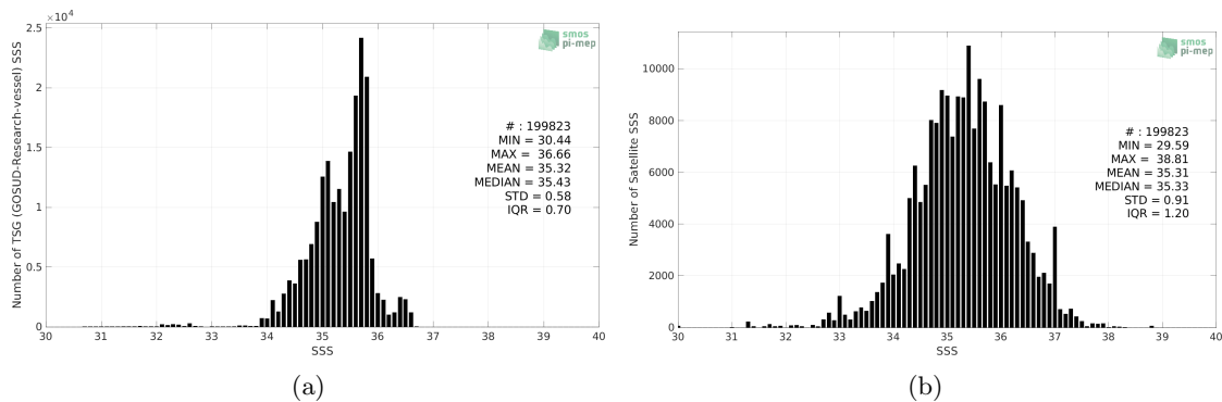
Figure 2: Histograms of SSS from TSG (GOSUD-Research-vessel) (a) and SMOS SSS L2Q v331 - 0.25 Deg (CATDS-CPDC) (b) considering all match-up pairs per bins of 0.1 over the South Pacific Ocean Pi-MEP region and for the full satellite product period.
