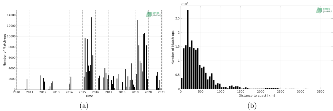
Figure 1: Number of match-ups between TSG (GOSUD-Research-vessel) and SMOS SSS L2Q v331 - 0.25 Deg (CATDS-CPDC) SSS as a function of time (a) and as function of the distance to coast (b) over the South Pacific Ocean Pi-MEP region and for the full satellite product period.
