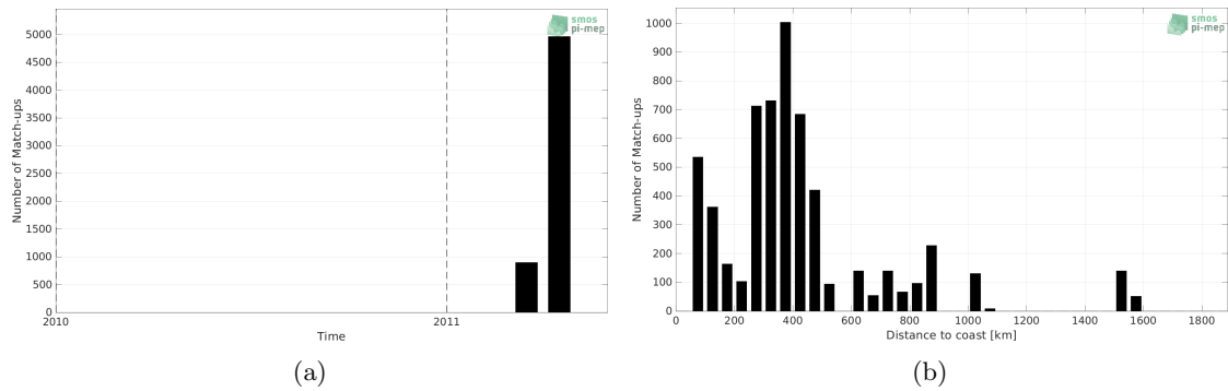
Figure 1: Number of match-ups between TSG (CSIC-UTM) and SMOS SSS L2Q v331 - 0.25 Deg (CATDS-CPDC) SSS as a function of time (a) and as function of the distance to coast (b) over the South Pacific Ocean Pi-MEP region and for the full satellite product period.
