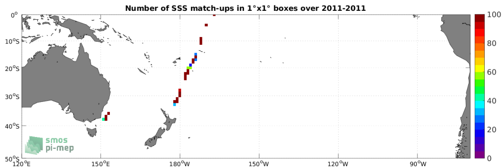
Figure 4: Number of SSS match-ups between TSG (CSIC-UTM) SSS and the SMOS SSS L2Q v331 - 0.25 Deg (CATDS-CPDC) SSS product for the South Pacific Ocean Pi-MEP region over 1^\circ \times 1^\circ boxes and for the full satellite product period.
