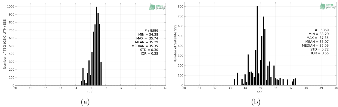
Figure 2: Histograms of SSS from TSG (CSIC-UTM) (a) and SMOS SSS L2Q v331 - 0.25 Deg (CATDS-CPDC) (b) considering all match-up pairs per bins of 0.1 over the South Pacific Ocean Pi-MEP region and for the full satellite product period.
