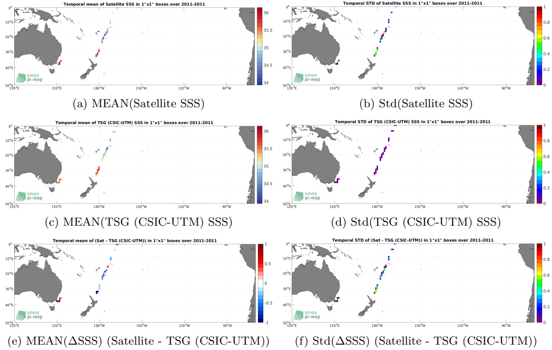
Figure 6: Temporal mean (left) and Std (right) of SSS from SMOS SSS L2Q v331 - 0.25 Deg (CATDS-CPDC) (top), TSG (CSIC-UTM) (middle), and of \Delta SSS (Satellite - TSG (CSIC-UTM)). Only match-up pairs are used to generate these maps.
