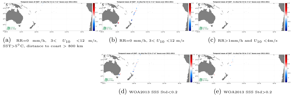
Figure 12: Temporal mean gridded over spatial boxes of size 1^{\circ}\times 1^{\circ} of \Delta\text{SSS} (SMOS SSS L2Q v331 - 0.25 Deg (CATDS-CPDC) - TSG (CSIC-UTM)) for 5 different subdatasets corresponding to:RR=0 mm/h, 3 < U_{10} < 12 m/s, SST >5^{\circ}\text{C} , distance to coast > 800 km (a), RR=0 mm/h, 3 < U_{10} < 12 m/s (b), RR >1 mm/h and U_{10} < 4 m/s (c), WOA2013 SSS Std <0.2 (d), WOA2013 SSS Std >0.2 (e).
