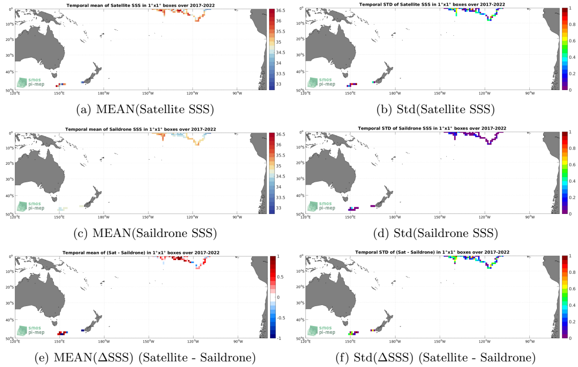
Figure 6: Temporal mean (left) and Std (right) of SSS from SMOS SSS L2Q v331 - 0.25 Deg (CATDS-CPDC) (top), Saildrone (middle), and of \Delta SSS (Satellite - Saildrone). Only match-up pairs are used to generate these maps.
