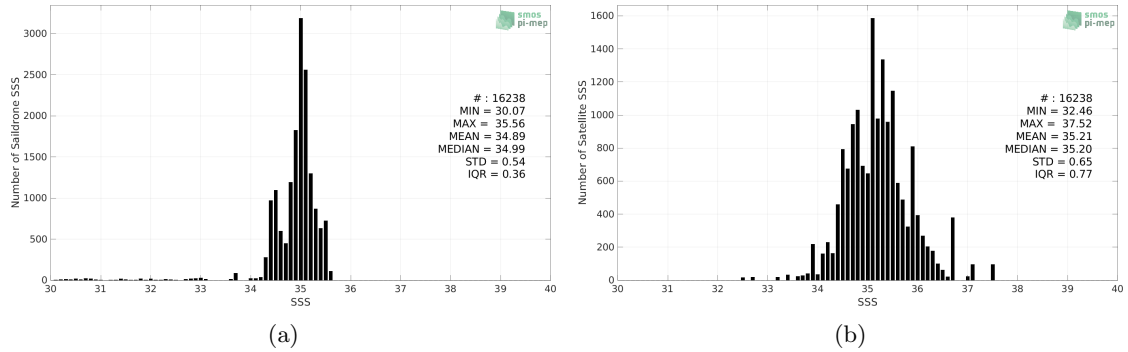
Figure 2: Histograms of SSS from Saildrone (a) and SMOS SSS L2Q v331 - 0.25 Deg (CATDS-CPDC) (b) considering all match-up pairs per bins of 0.1 over the South Pacific Ocean Pi-MEP region and for the full satellite product period.
