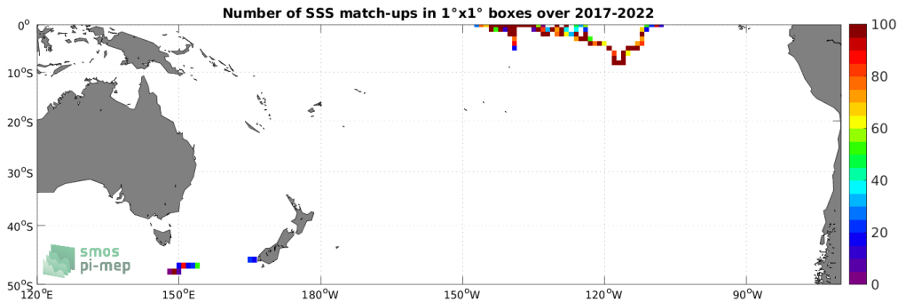
Figure 4: Number of SSS match-ups between Saildrone SSS and the SMOS SSS L2Q v331 - 0.25 Deg (CATDS-CPDC) SSS product for the South Pacific Ocean Pi-MEP region over 1^\circ \times 1^\circ boxes and for the full satellite product period.
