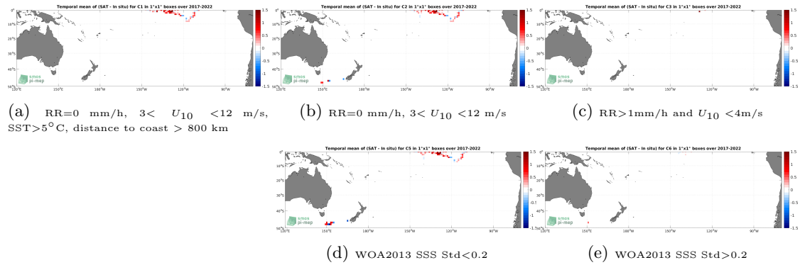
Figure 12: Temporal mean gridded over spatial boxes of size 1^\circ \times 1^\circ of \Delta SSS (SMOS SSS L2Q v331 - 0.25 Deg (CATDS-CPDC) - Sailydrone) for 5 different subdatasets corresponding to:RR=0 mm/h, 3 < U_{10} < 12 m/s, SST >5^\circ C, distance to coast > 800 km (a), RR=0 mm/h, 3 < U_{10} < 12 m/s (b), RR >1 mm/h and U_{10} < 4 m/s (c), WOA2013 SSS Std <0.2 (d), WOA2013 SSS Std >0.2 (e).
