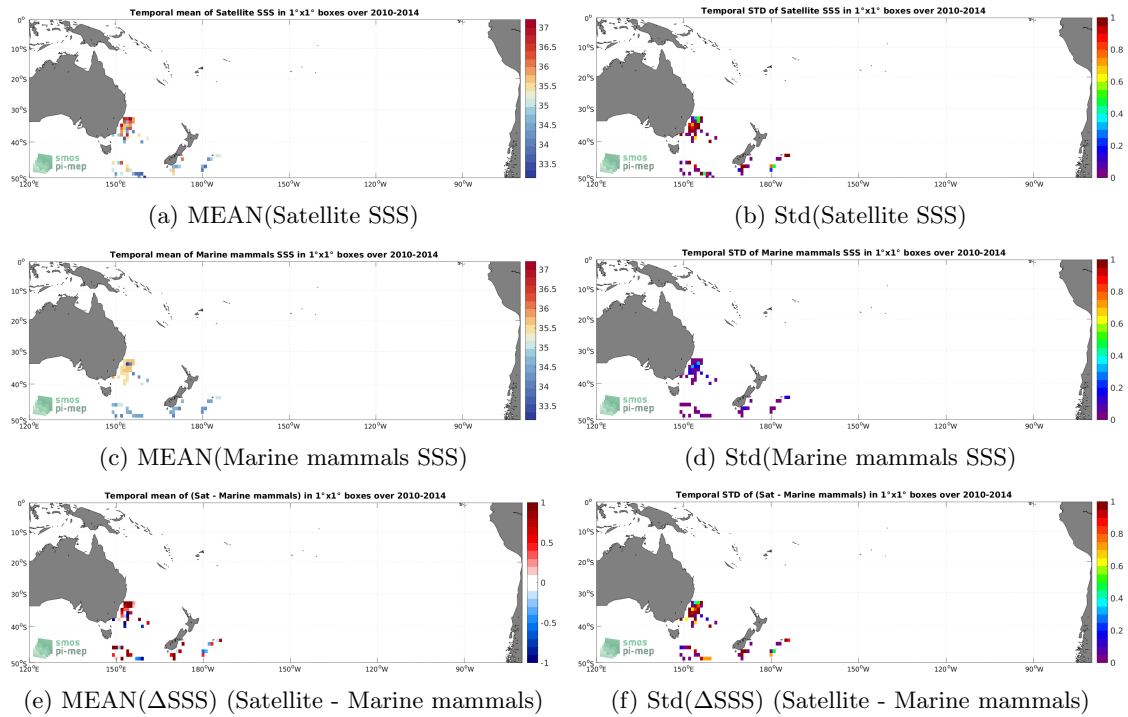
Figure 6: Temporal mean (left) and Std (right) of SSS from SMOS SSS L2Q v331 - 0.25 Deg (CATDS-CPDC) (top), Marine mammals (middle), and of \Delta SSS (Satellite - Marine mammals). Only match-up pairs are used to generate these maps.
