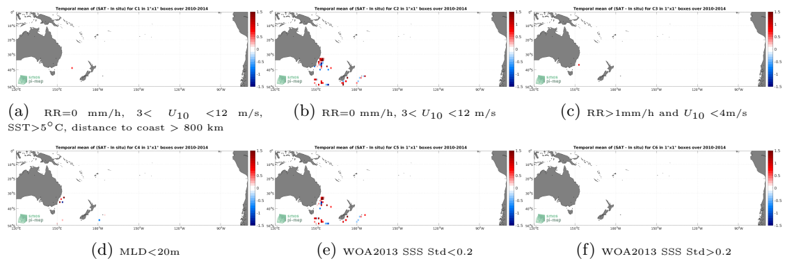
Figure 12: Temporal mean gridded over spatial boxes of size 1^\circ \times 1^\circ of \Delta SSS (SMOS SSS L2Q v331 - 0.25 Deg (CATDS-CPDC) - Marine mammals) for 6 different subdatasets corresponding to:RR=0 mm/h, 3 < U_{10} < 12 m/s, SST >5^\circ C, distance to coast > 800 km (a), RR=0 mm/h, 3 < U_{10} < 12 m/s (b), RR >1 mm/h and U_{10} < 4 m/s (c),MLD <20 m (d),WOA2013 SSS Std <0.2 (e),WOA2013 SSS Std >0.2 (f).
