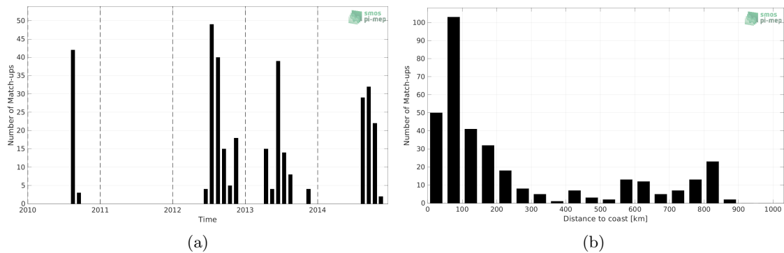
Figure 1: Number of match-ups between Marine mammals and SMOS SSS L2Q v331 - 0.25 Deg (CATDS-CPDC) SSS as a function of time (a) and as function of the distance to coast (b) over the South Pacific Ocean Pi-MEP region and for the full satellite product period.
