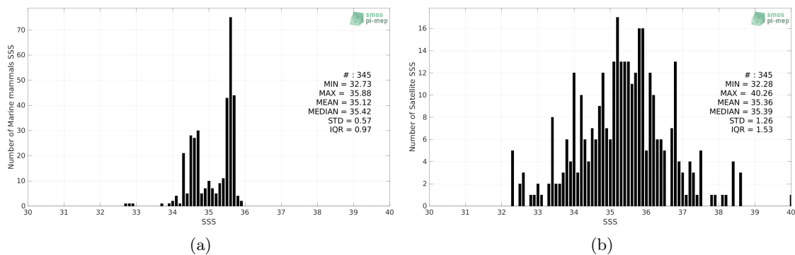
Figure 2: Histograms of SSS from Marine mammals (a) and SMOS SSS L2Q v331 - 0.25 Deg (CATDS-CPDC) (b) considering all match-up pairs per bins of 0.1 over the South Pacific Ocean Pi-MEP region and for the full satellite product period.
