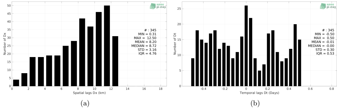
Figure 5: Histograms of the spatial (a) and temporal (b) lags between the location/time of the Marine mammals measurement and the date of the corresponding SMOS SSS L2Q v331 - 0.25 Deg (CATDS-CPDC) SSS pixel.
