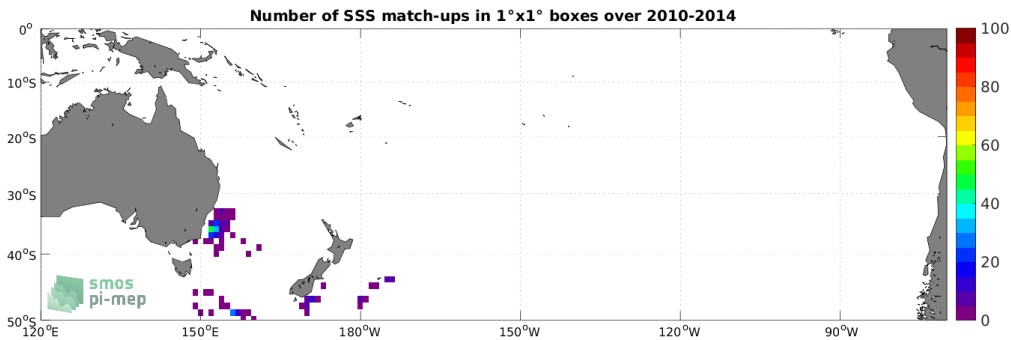
Figure 4: Number of SSS match-ups between Marine mammals SSS and the SMOS SSS L2Q v331 - 0.25 Deg (CATDS-CPDC) SSS product for the South Pacific Ocean Pi-MEP region over 1^\circ \times 1^\circ boxes and for the full satellite product period.
