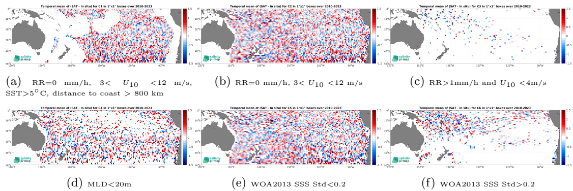
Figure 12: Temporal mean gridded over spatial boxes of size 1^\circ \times 1^\circ of \Delta SSS (SMOS SSS L2Q v331 - 0.25 Deg (CATDS-CPDC) - Argo) for 6 different subdatasets corresponding to:RR=0 mm/h, 3 < U_{10} < 12 m/s, SST >5^\circ C, distance to coast > 800 km (a), RR=0 mm/h, 3 < U_{10} < 12 m/s (b), RR >1 mm/h and U_{10} < 4 m/s (c),MLD <20 m (d),WOA2013 SSS Std <0.2 (e),WOA2013 SSS Std >0.2 (f).
