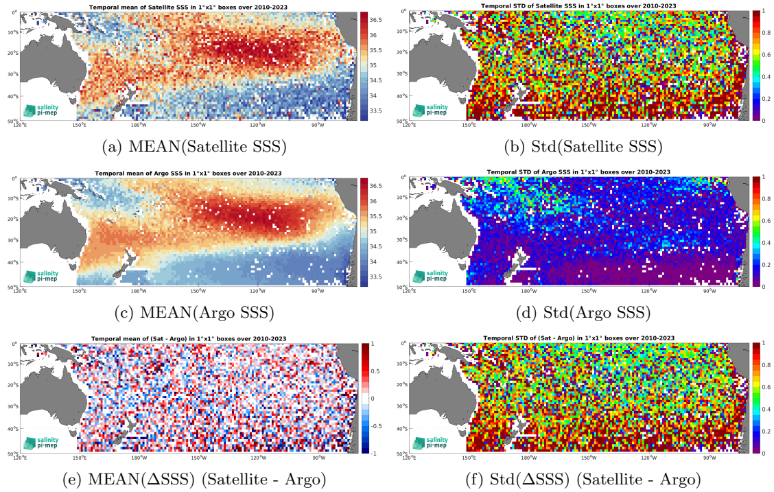
Figure 6: Temporal mean (left) and Std (right) of SSS from SMOS SSS L2Q v331 - 0.25 Deg (CATDS-CPDC) (top), Argo (middle), and of \Delta SSS (Satellite - Argo). Only match-up pairs are used to generate these maps.
