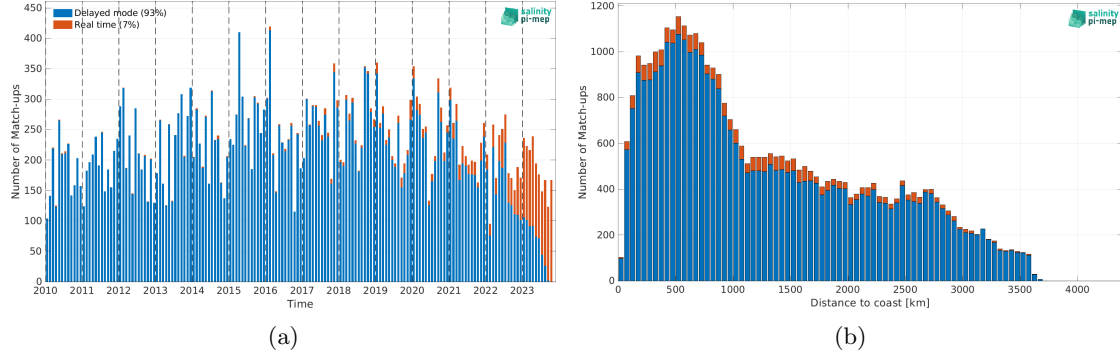
Figure 1: Number of match-ups between Argo and SMOS SSS L2Q v331 - 0.25 Deg (CATDS-CPDC) SSS as a function of time (a) and as function of the distance to coast (b) over the South Pacific Ocean Pi-MEP region and for the full satellite product period.
