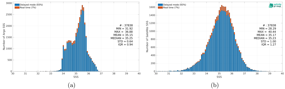
Figure 2: Histograms of SSS from Argo (a) and SMOS SSS L2Q v331 - 0.25 Deg (CATDS-CPDC) (b) considering all match-up pairs per bins of 0.1 over the South Pacific Ocean Pi-MEP region and for the full satellite product period.
