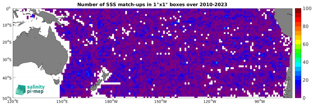
Figure 4: Number of SSS match-ups between Argo SSS and the SMOS SSS L2Q v331 - 0.25 Deg (CATDS-CPDC) SSS product for the South Pacific Ocean Pi-MEP region over 1^\circ \times 1^\circ boxes and for the full satellite product period.
