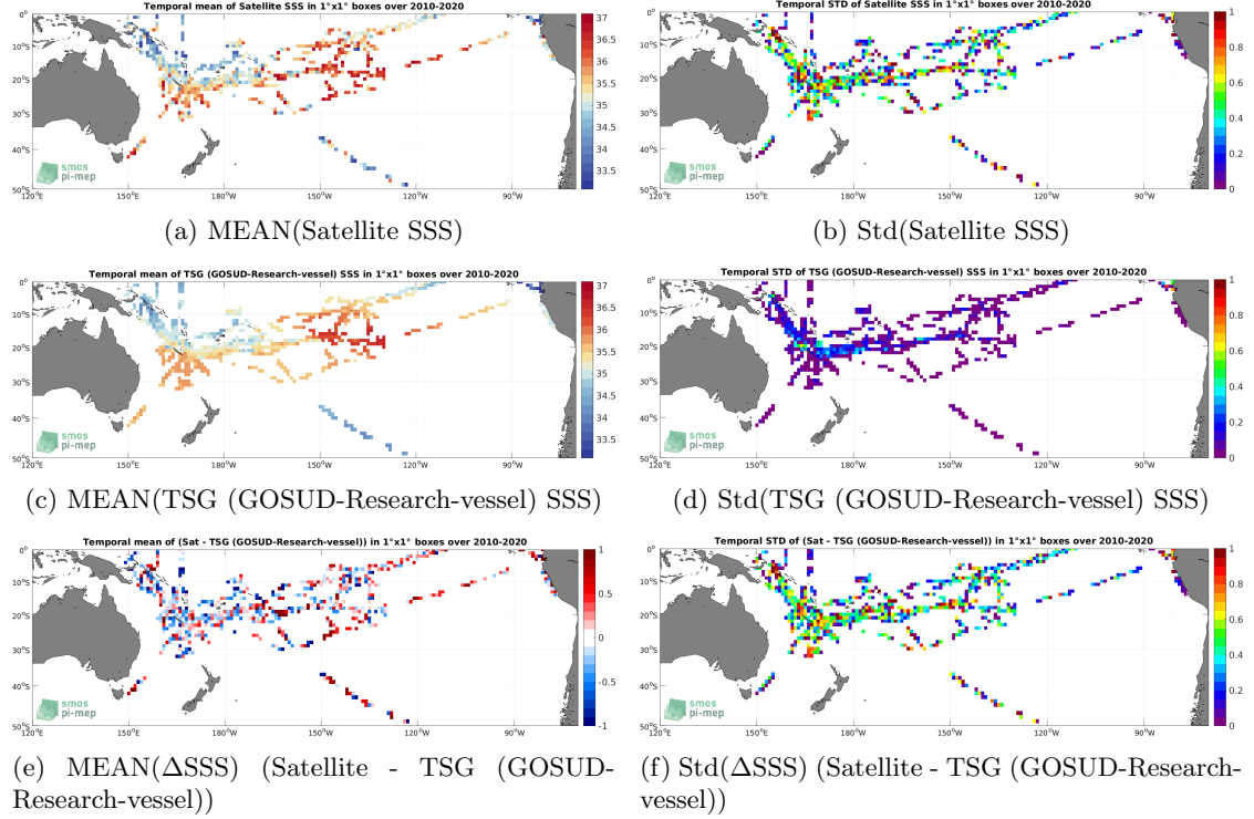
Figure 6: Temporal mean (left) and Std (right) of SSS from SMOS SSS L2Q v330 - 0.25 Deg (CATDS-CPDC) (top), TSG (GOSUD-Research-vessel) (middle), and of \Delta SSS (Satellite - TSG (GOSUD-Research-vessel)). Only match-up pairs are used to generate these maps.
