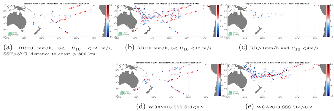
Figure 12: Temporal mean gridded over spatial boxes of size 1^\circ \times 1^\circ of \Delta SSS (SMOS SSS L2Q v330 - 0.25 Deg (CATDS-CPDC) - TSG (GOSUD-Research-vessel)) for 5 different subdatasets corresponding to:RR=0 mm/h, 3 < U_{10} < 12 m/s, SST >5^\circ\text{C} , distance to coast > 800 km (a), RR=0 mm/h, 3 < U_{10} < 12 m/s (b), RR >1 mm/h and U_{10} < 4 m/s (c), WOA2013 SSS Std <0.2 (d), WOA2013 SSS Std >0.2 (e).
