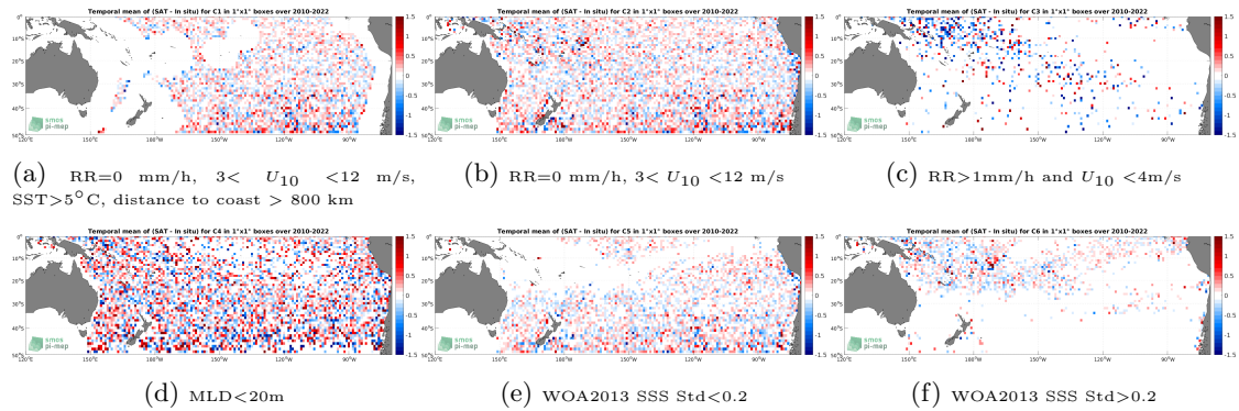
Figure 12: Temporal mean gridded over spatial boxes of size 1^\circ \times 1^\circ of \Delta SSS (SMOS SSS L2Q v330 - 0.25 Deg (CATDS-CPDC) - Argo) for 6 different subdatasets corresponding to:RR=0 mm/h, 3 < U_{10} < 12 m/s, SST >5^\circ C, distance to coast > 800 km (a), RR=0 mm/h, 3 < U_{10} < 12 m/s (b), RR >1 mm/h and U_{10} < 4 m/s (c),MLD <20 m (d),WOA2013 SSS Std <0.2 (e),WOA2013 SSS Std >0.2 (f).
