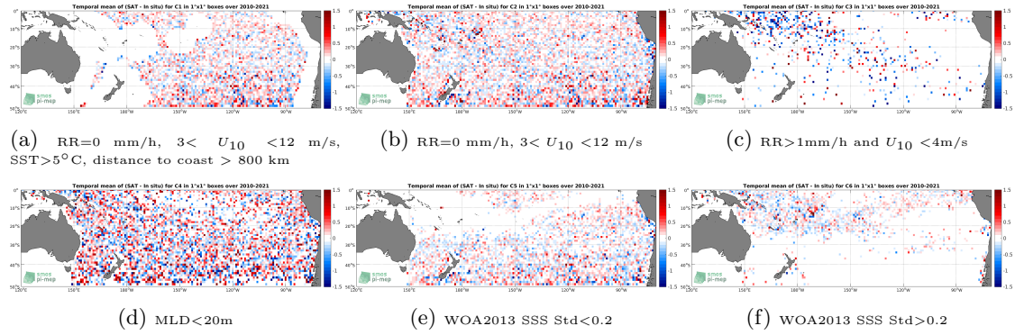
Figure 12: Temporal mean gridded over spatial boxes of size 1^\circ \times 1^\circ of \Delta SSS (SMOS SSS L2Q v330 - 0.25 Deg (CATDS-CPDC) - Argo) for 6 different subdatasets corresponding to: RR=0 mm/h, 3 < U_{10} < 12 m/s, SST > 5^\circ C , distance to coast > 800 km (a), RR=0 mm/h, 3 < U_{10} < 12 m/s (b), RR > 1 mm/h and U_{10} < 4 m/s (c), MLD < 20 m (d), WOA2013 SSS Std < 0.2 (e), WOA2013 SSS Std > 0.2 (f).
