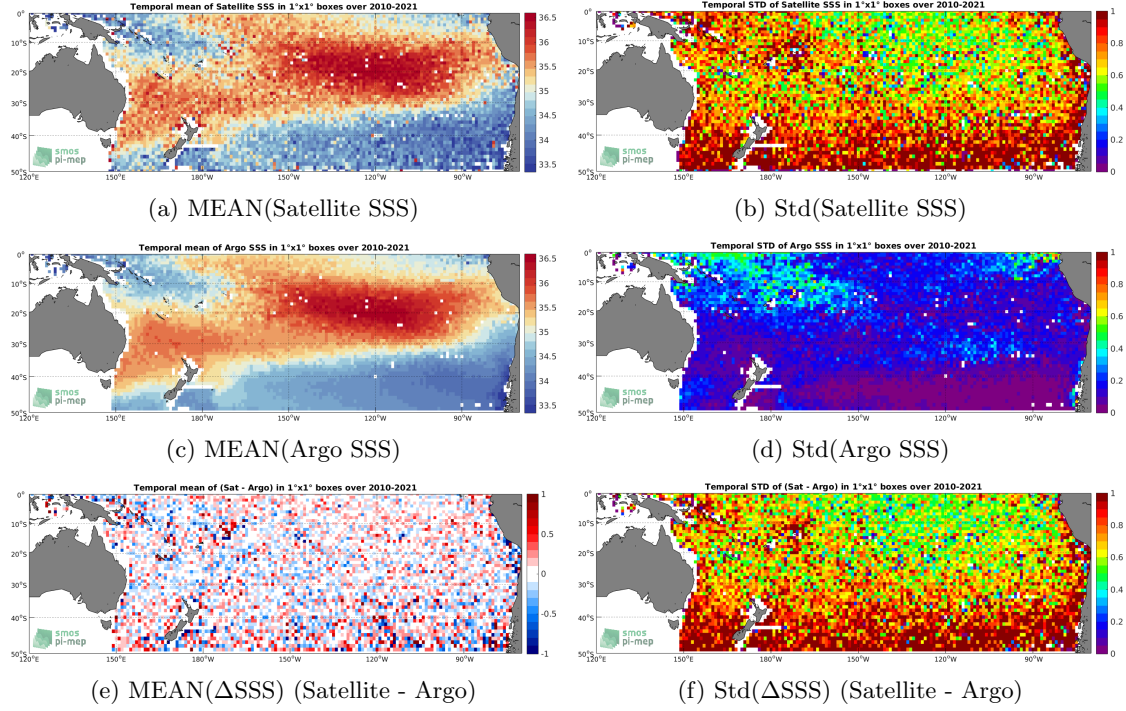
Figure 6: Temporal mean (left) and Std (right) of SSS from SMOS SSS L2Q v330 - 0.25 Deg (CATDS-CPDC) (top), Argo (middle), and of \Delta SSS (Satellite - Argo). Only match-up pairs are used to generate these maps.
