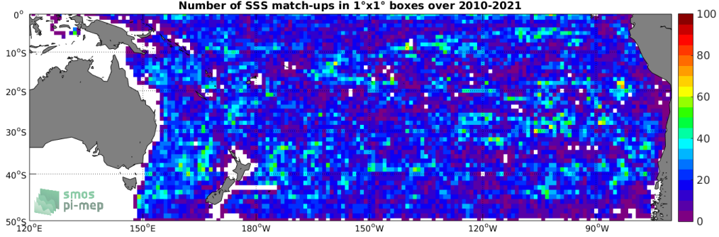
Figure 4: Number of SSS match-ups between Argo SSS and the SMOS SSS L2Q v330 - 0.25 Deg (CATDS-CPDC) SSS product for the South Pacific Ocean Pi-MEP region over 1^\circ \times 1^\circ boxes and for the full satellite product period.
