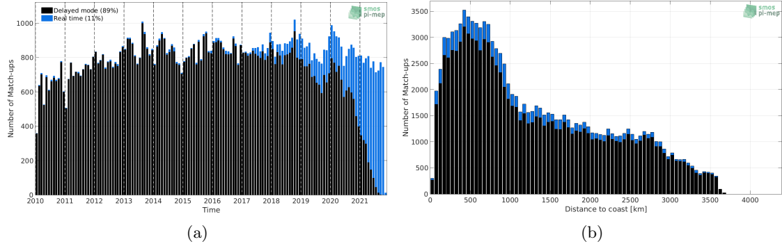
Figure 1: Number of match-ups between Argo and SMOS SSS L2Q v330 - 0.25 Deg (CATDS-CPDC) SSS as a function of time (a) and as function of the distance to coast (b) over the South Pacific Ocean Pi-MEP region and for the full satellite product period.
