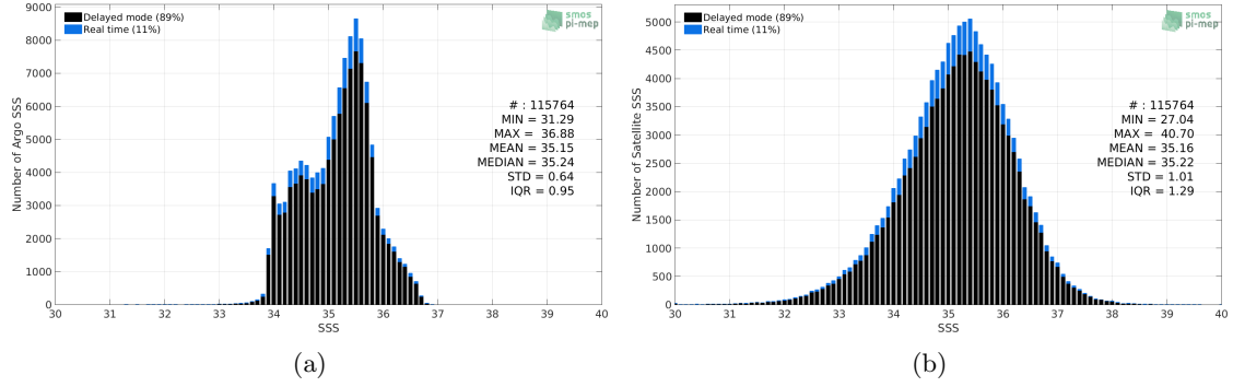
Figure 2: Histograms of SSS from Argo (a) and SMOS SSS L2Q v330 - 0.25 Deg (CATDS-CPDC) (b) considering all match-up pairs per bins of 0.1 over the South Pacific Ocean Pi-MEP region and for the full satellite product period.
