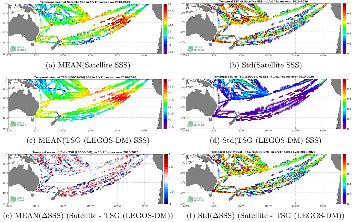
Figure 6: Temporal mean (left) and Std (right) of SSS from SMOS SSS L2Q v321 - 0.25 Deg (CATDS-CPDC) (top), TSG (LEGOS-DM) (middle), and of \Delta SSS (Satellite - TSG (LEGOS-DM)). Only match-up pairs are used to generate these maps.
