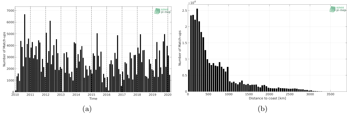
Figure 1: Number of match-ups between TSG (LEGOS-DM) and SMOS SSS L2Q v321 - 0.25 Deg (CATDS-CPDC) SSS as a function of time (a) and as function of the distance to coast (b) over the South Pacific Ocean Pi-MEP region and for the full satellite product period.
