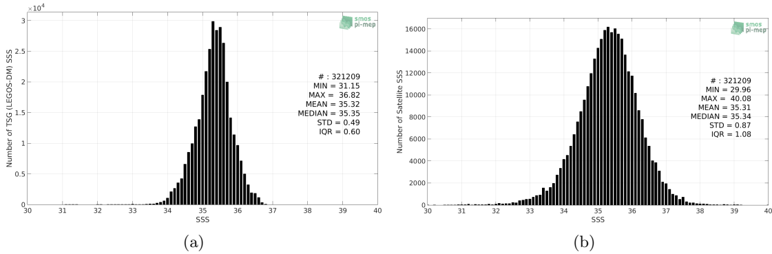
Figure 2: Histograms of SSS from TSG (LEGOS-DM) (a) and SMOS SSS L2Q v321 - 0.25 Deg (CATDS-CPDC) (b) considering all match-up pairs per bins of 0.1 over the South Pacific Ocean Pi-MEP region and for the full satellite product period.
