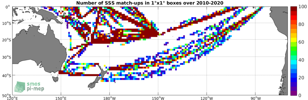
Figure 4: Number of SSS match-ups between TSG (LEGOS-DM) SSS and the SMOS SSS L2Q v321 - 0.25 Deg (CATDS-CPDC) SSS product for the South Pacific Ocean Pi-MEP region over 1^\circ \times 1^\circ boxes and for the full satellite product period.
