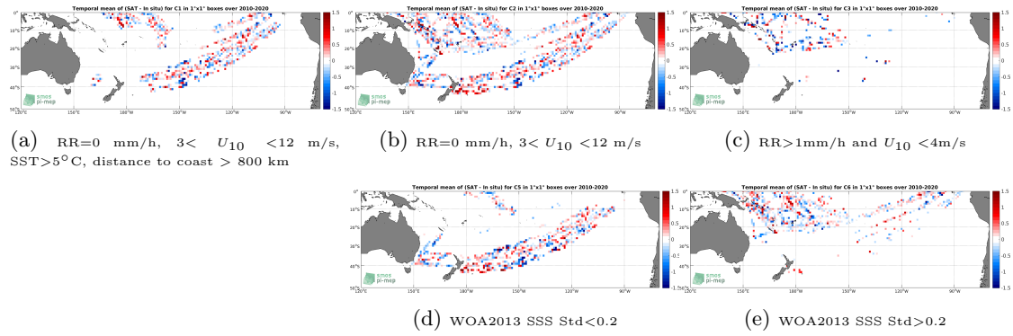
Figure 12: Temporal mean gridded over spatial boxes of size 1^\circ \times 1^\circ of \Delta SSS (SMOS SSS L2Q v321 - 0.25 Deg (CATDS-CPDC) - TSG (LEGOS-DM)) for 5 different subdatasets corresponding to: RR=0 mm/h, 3 < U_{10} < 12 m/s, SST >5^\circ C, distance to coast > 800 km (a), RR=0 mm/h, 3 < U_{10} < 12 m/s (b), RR>1 mm/h and U_{10} < 4 m/s (c), WOA2013 SSS Std <0.2 (d), WOA2013 SSS Std >0.2 (e).
