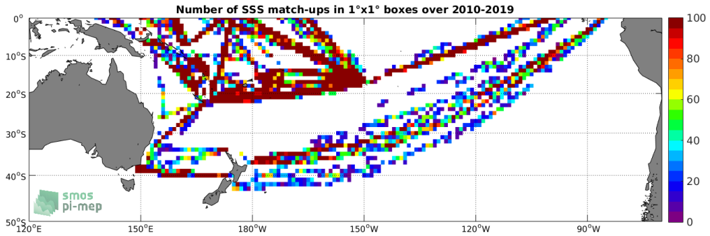
Figure 4: Number of SSS match-ups between TSG (LEGOS-DM) SSS and the SMOS SSS L2Q v321 - 0.25 Deg (CATDS-CPDC) SSS product for the South Pacific Ocean Pi-MEP region over 1°x1° boxes and for the full satellite product period.
