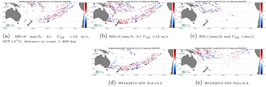
Figure 12: Temporal mean gridded over spatial boxes of size 1^\circ \times 1^\circ of \Delta SSS (SMOS L2Q v321 - 0.25 Deg (CATDS-CPDC) - TSG-LEGOS-DM) for 5 different subdatasets corresponding to: RR=0 mm/h, 3 < U_{10} < 12 m/s, SST > 5^\circ\text{C} , distance to coast > 800 km (a), RR=0 mm/h, 3 < U_{10} < 12 m/s (b), RR > 1\text{mm/h} and U_{10} < 4\text{m/s} (c), WOA2013 SSS Std < 0.2 (d), WOA2013 SSS Std > 0.2 (e).
