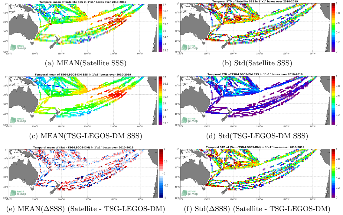
Figure 6: Temporal mean (left) and Std (right) of SSS from SMOS L2Q v321 - 0.25 Deg (CATDS-CPDC) (top), TSG-LEGOS-DM (middle), and of \Delta SSS (Satellite - TSG-LEGOS-DM). Only match-up pairs are used to generate these maps.
