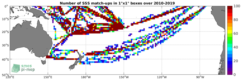
Figure 4: Number of SSS match-ups between TSG-LEGOS-DM SSS and the SMOS L2Q v321 - 0.25 Deg (CATDS-CPDC) SSS product for the South Pacific Ocean Pi-MEP region over 1°x1° boxes and for the full satellite product period.
