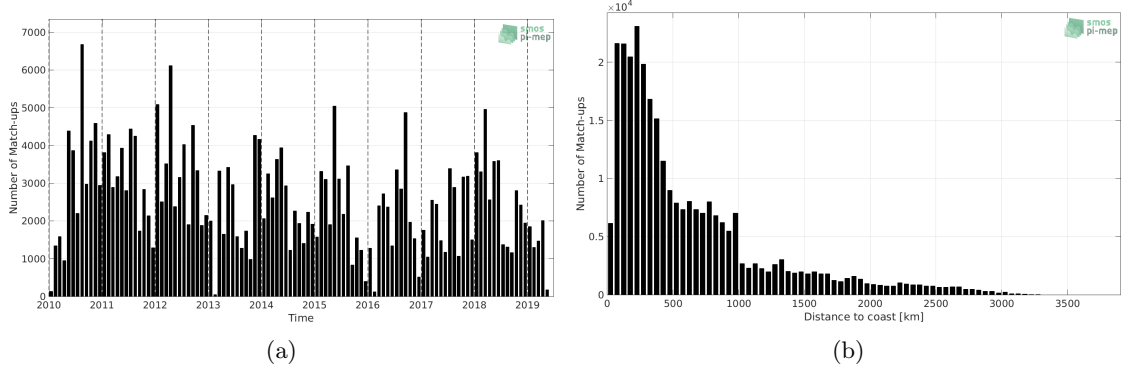
Figure 1: Number of match-ups between TSG-LEGOS-DM and SMOS L2Q v321 - 0.25 Deg (CATDS-CPDC) SSS as a function of time (a) and as function of the distance to coast (b) over the South Pacific Ocean Pi-MEP region and for the full satellite product period.
