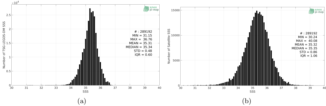
Figure 2: Histograms of SSS from TSG-LEGOS-DM (a) and SMOS L2Q v321 - 0.25 Deg (CATDS-CPDC) (b) considering all match-up pairs per bins of 0.1 over the South Pacific Ocean Pi-MEP region and for the full satellite product period.
