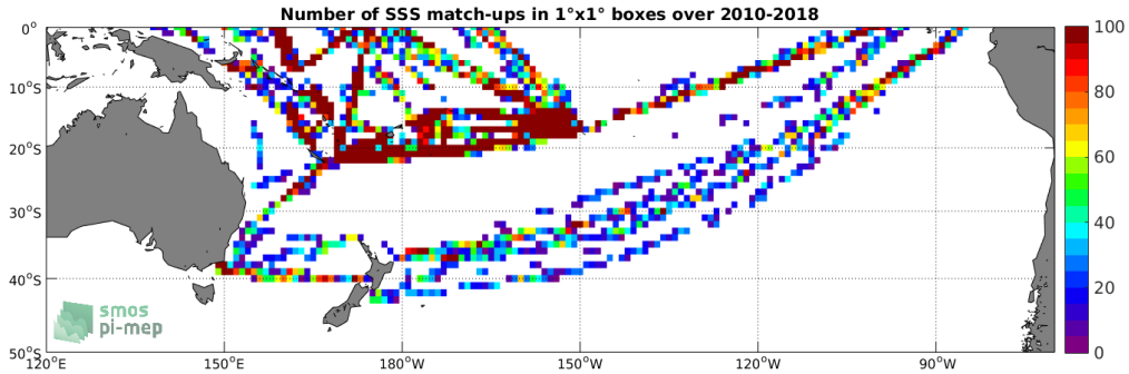
Figure 4: Number of SSS match-ups between TSG-LEGOS-DM SSS and the SMOS-L3-CATDS-CPDC-V321-L2Q SSS product for the South Pacific Ocean Pi-MEP region over 1°x1° boxes and for the full satellite product period.
