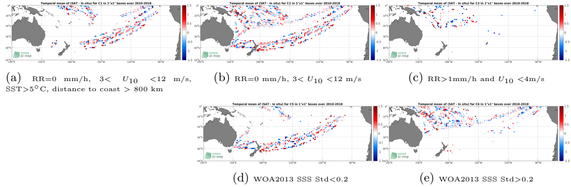
Figure 12: Temporal mean gridded over spatial boxes of size 1^\circ \times 1^\circ of \Delta SSS (SMOS-L3-CATDS-CPDC-V321-L2Q - TSG-LEGOS-DM) for 5 different subdatasets corresponding to: RR=0 mm/h, 3 < U_{10} < 12 m/s, SST > 5^\circ\text{C} , distance to coast > 800 km (a), RR=0 mm/h, 3 < U_{10} < 12 m/s (b), RR > 1 mm/h and U_{10} < 4 m/s (c), WOA2013 SSS Std < 0.2 (d), WOA2013 SSS Std > 0.2 (e).
