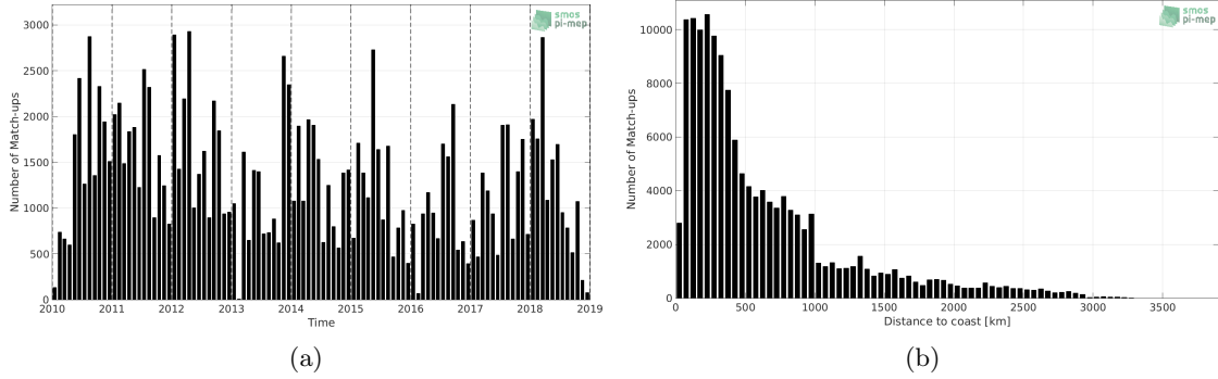
Figure 1: Number of match-ups between TSG-LEGOS-DM and SMOS-L3-CATDS-CPDC-V321-L2Q SSS as a function of time (a) and as function of the distance to coast (b) over the South Pacific Ocean Pi-MEP region and for the full satellite product period.
