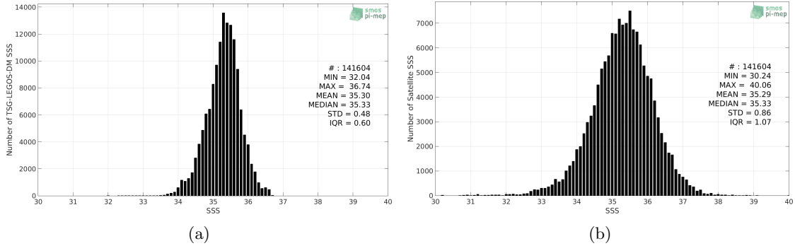
Figure 2: Histograms of SSS from TSG-LEGOS-DM (a) and SMOS-L3-CATDS-CPDC-V321-L2Q (b) considering all match-up pairs per bins of 0.1 over the South Pacific Ocean Pi-MEP region and for the full satellite product period.
