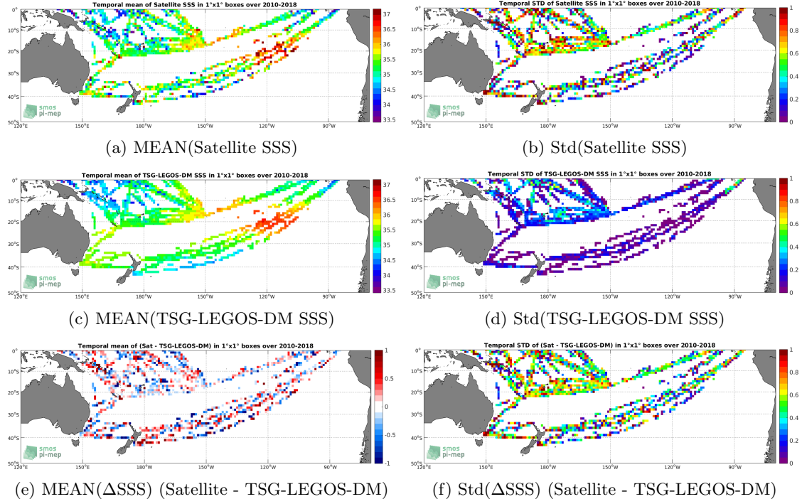
Figure 6: Temporal mean (left) and Std (right) of SSS from SMOS-L3-CATDS-CPDC-V321-L2Q (top), TSG-LEGOS-DM (middle), and of \Delta SSS (Satellite - TSG-LEGOS-DM). Only match-up pairs are used to generate these maps.
