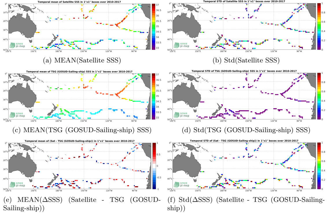
Figure 6: Temporal mean (left) and Std (right) of SSS from SMOS SSS L2Q v321 - 0.25 Deg (CATDS-CPDC) (top), TSG (GOSUD-Sailing-ship) (middle), and of \Delta SSS (Satellite - TSG (GOSUD-Sailing-ship)). Only match-up pairs are used to generate these maps.
