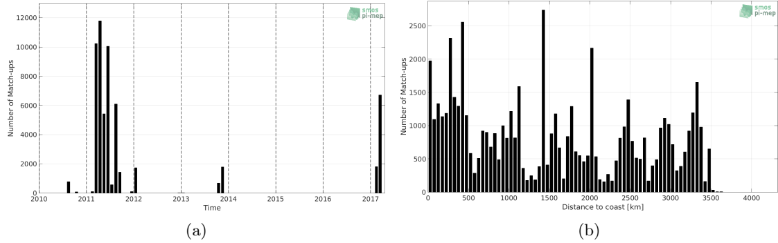
Figure 1: Number of match-ups between TSG (GOSUD-Sailing-ship) and SMOS SSS L2Q v321 - 0.25 Deg (CATDS-CPDC) SSS as a function of time (a) and as function of the distance to coast (b) over the South Pacific Ocean Pi-MEP region and for the full satellite product period.
