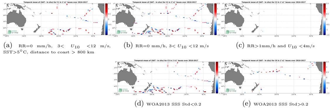
Figure 12: Temporal mean gridded over spatial boxes of size 1^\circ \times 1^\circ of \Delta SSS (SMOS SSS L2Q v321 - 0.25 Deg (CATDS-CPDC) - TSG (GOSUD-Sailing-ship)) for 5 different subdatasets corresponding to: RR=0 mm/h, 3 < U_{10} < 12 m/s, SST > 5^\circ C , distance to coast > 800 km (a), RR=0 mm/h, 3 < U_{10} < 12 m/s (b), RR > 1 mm/h and U_{10} < 4 m/s (c), WOA2013 SSS Std < 0.2 (d), WOA2013 SSS Std > 0.2 (e).
