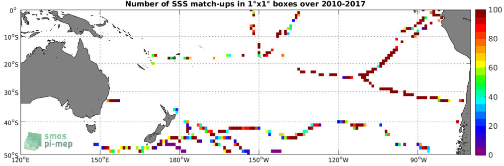
Figure 4: Number of SSS match-ups between TSG (GOSUD-Sailing-ship) SSS and the SMOS SSS L2Q v321 - 0.25 Deg (CATDS-CPDC) SSS product for the South Pacific Ocean Pi-MEP region over 1^\circ \times 1^\circ boxes and for the full satellite product period.
