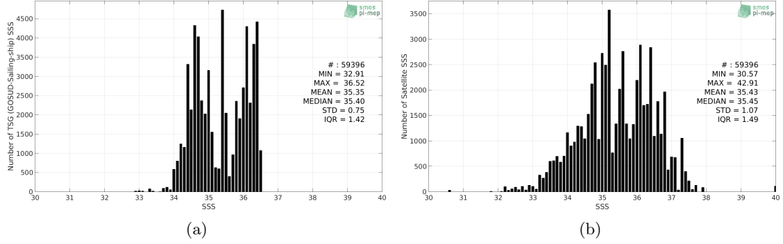
Figure 2: Histograms of SSS from TSG (GOSUD-Sailing-ship) (a) and SMOS SSS L2Q v321 - 0.25 Deg (CATDS-CPDC) (b) considering all match-up pairs per bins of 0.1 over the South Pacific Ocean Pi-MEP region and for the full satellite product period.
