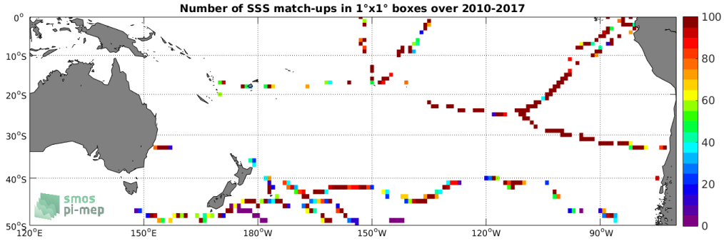
Figure 4: Number of SSS match-ups between TSG (GOSUD-Sailing-ship) SSS and the SMOS SSS L2Q v321 - 0.25 Deg (CATDS-CPDC) SSS product for the South Pacific Ocean Pi-MEP region over 1°x1° boxes and for the full satellite product period.
