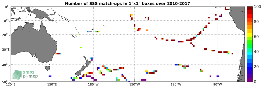
Figure 4: Number of SSS match-ups between TSG-GOSUD-Sailing-ship SSS and the SMOS-L3-CATDS-CPDC-V321-L2Q SSS product for the South Pacific Ocean Pi-MEP region over 1°x1° boxes and for the full satellite product period.
