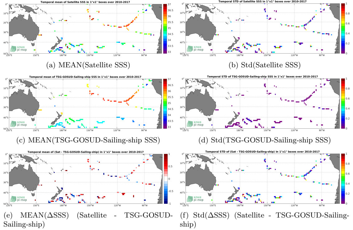
Figure 6: Temporal mean (left) and Std (right) of SSS from SMOS-L3-CATDS-CPDC-V321-L2Q (top), TSG-GOSUD-Sailing-ship (middle), and of \Delta SSS (Satellite - TSG-GOSUD-Sailing-ship). Only match-up pairs are used to generate these maps.
