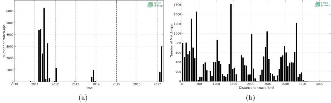
Figure 1: Number of match-ups between TSG-GOSUD-Sailing-ship and SMOS-L3-CATDS-CPDC-V321-L2Q SSS as a function of time (a) and as function of the distance to coast (b) over the South Pacific Ocean Pi-MEP region and for the full satellite product period.
