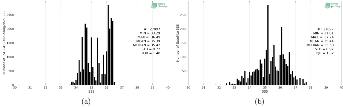
Figure 2: Histograms of SSS from TSG-GOSUD-Sailing-ship (a) and SMOS-L3-CATDS-CPDC-V321-L2Q (b) considering all match-up pairs per bins of 0.1 over the South Pacific Ocean Pi-MEP region and for the full satellite product period.
