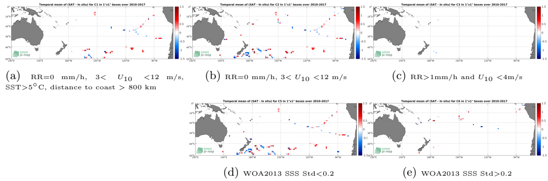
Figure 12: Temporal mean gridded over spatial boxes of size 1^\circ \times 1^\circ of \Delta SSS (SMOS-L3-CATDS-CPDC-V321-L2Q - TSG-GOSUD-Sailing-ship) for 5 different subdatasets corresponding to: RR=0 mm/h, 3 < U_{10} < 12 m/s, SST > 5^\circ\text{C} , distance to coast > 800 km (a), RR=0 mm/h, 3 < U_{10} < 12 m/s (b), RR > 1 mm/h and U_{10} < 4 m/s (c), WOA2013 SSS Std < 0.2 (d), WOA2013 SSS Std > 0.2 (e).
