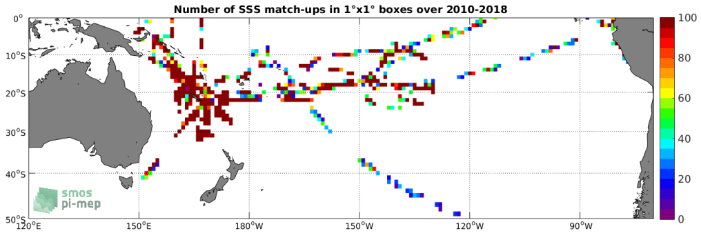
Figure 4: Number of SSS match-ups between TSG (GOSUD-Research-vessel) SSS and the SMOS SSS L2Q v321 - 0.25 Deg (CATDS-CPDC) SSS product for the South Pacific Ocean Pi-MEP region over 1°x1° boxes and for the full satellite product period.
