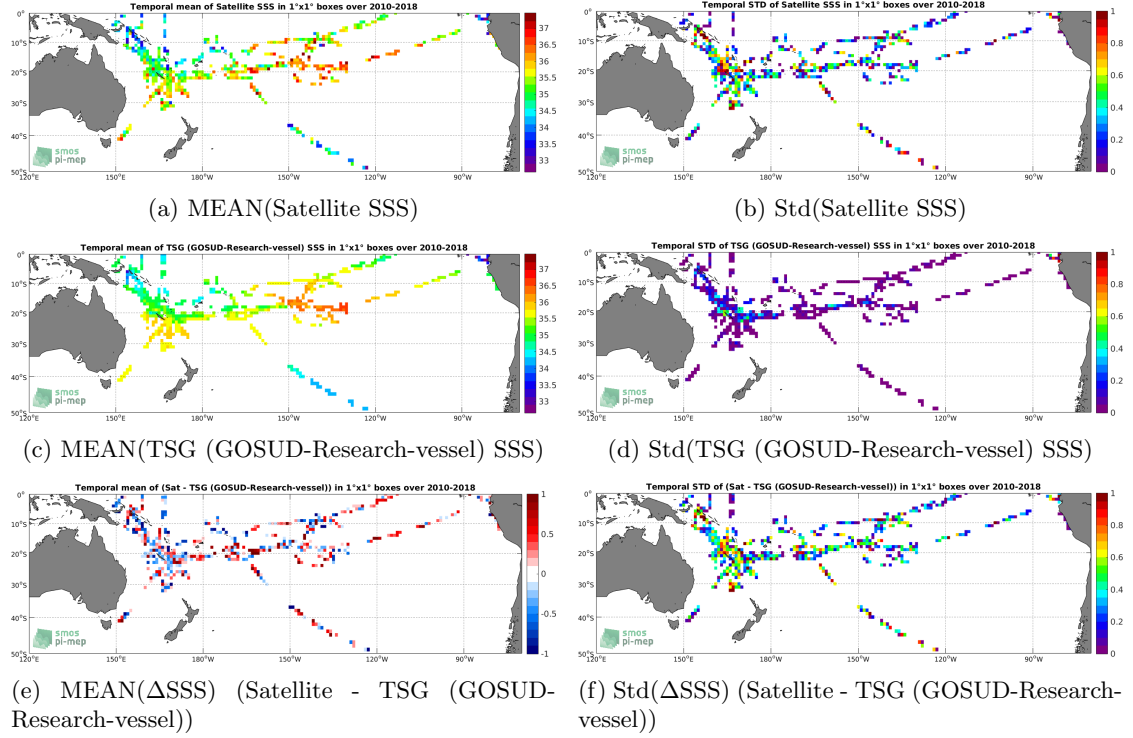
Figure 6: Temporal mean (left) and Std (right) of SSS from SMOS SSS L2Q v321 - 0.25 Deg (CATDS-CPDC) (top), TSG (GOSUD-Research-vessel) (middle), and of \Delta SSS (Satellite - TSG (GOSUD-Research-vessel)). Only match-up pairs are used to generate these maps.
