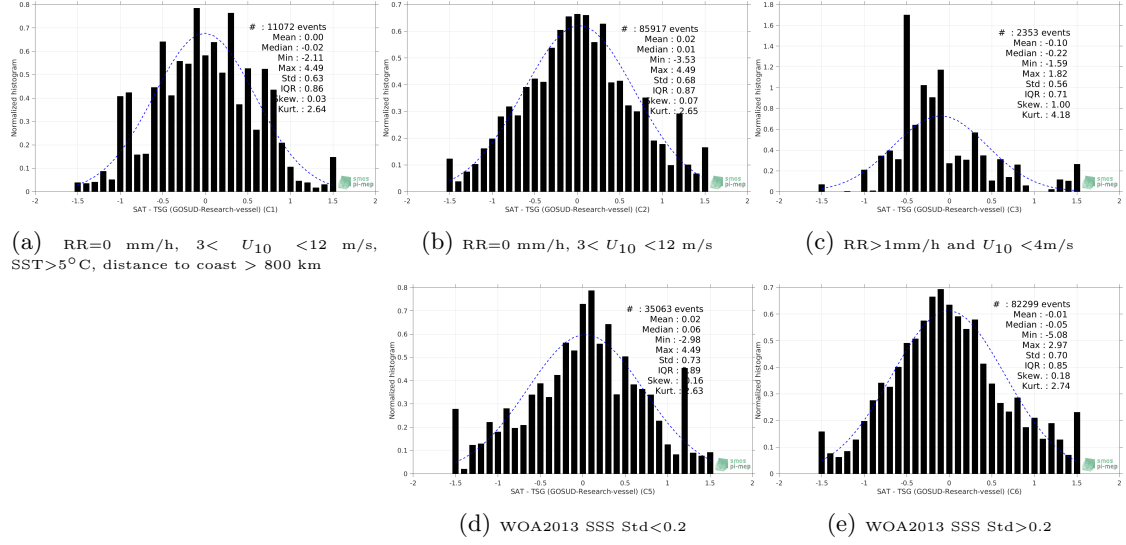
Figure 13: Normalized histogram of \Delta\text{SSS} (SMOS SSS L2Q v321 - 0.25 Deg (CATDS-CPDC) - TSG (GOSUD-Research-vessel)) for 5 different subdatasets corresponding to: RR=0 mm/h, 3 < U_{10} < 12 m/s, SST>5°C, distance to coast > 800 km (a), RR=0 mm/h, 3 < U_{10} < 12 m/s (b), RR>1mm/h and U_{10} < 4 m/s (c), WOA2013 SSS Std<0.2 (d), WOA2013 SSS Std>0.2 (e).
