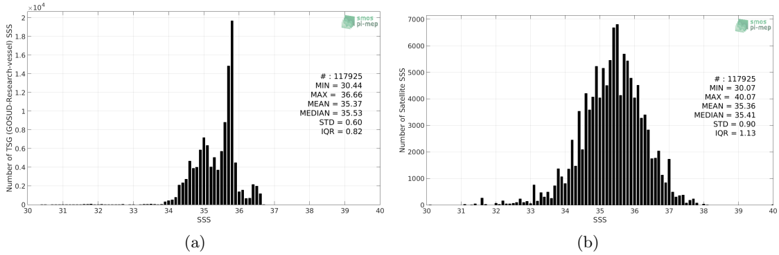
Figure 2: Histograms of SSS from TSG (GOSUD-Research-vessel) (a) and SMOS SSS L2Q v321 - 0.25 Deg (CATDS-CPDC) (b) considering all match-up pairs per bins of 0.1 over the South Pacific Ocean Pi-MEP region and for the full satellite product period.
