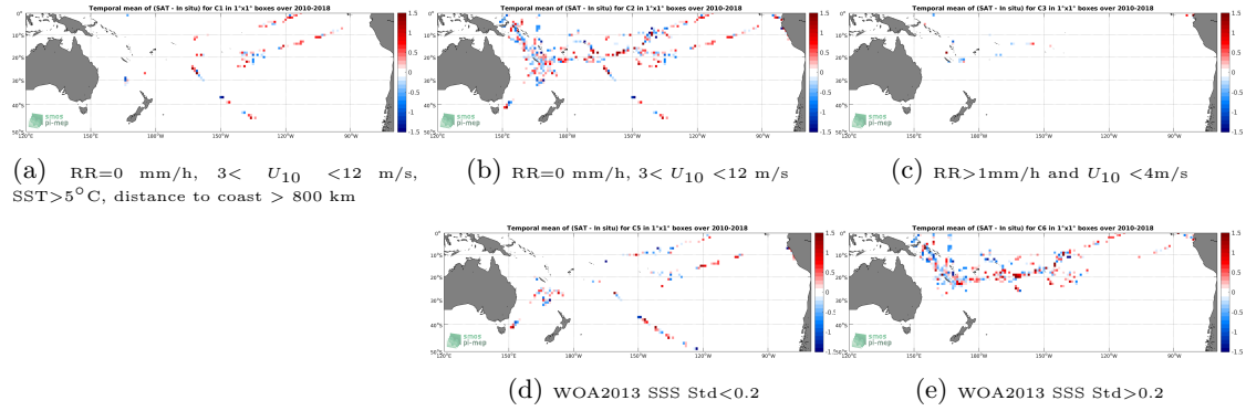
Figure 12: Temporal mean gridded over spatial boxes of size 1^\circ \times 1^\circ of \Delta SSS (SMOS SSS L2Q v321 - 0.25 Deg (CATDS-CPDC) - TSG (GOSUD-Research-vessel)) for 5 different subdatasets corresponding to: RR=0 mm/h, 3 < U_{10} < 12 m/s, SST > 5^\circ\text{C} , distance to coast > 800 km (a), RR=0 mm/h, 3 < U_{10} < 12 m/s (b), RR > 1 mm/h and U_{10} < 4 m/s (c), WOA2013 SSS Std < 0.2 (d), WOA2013 SSS Std > 0.2 (e).
