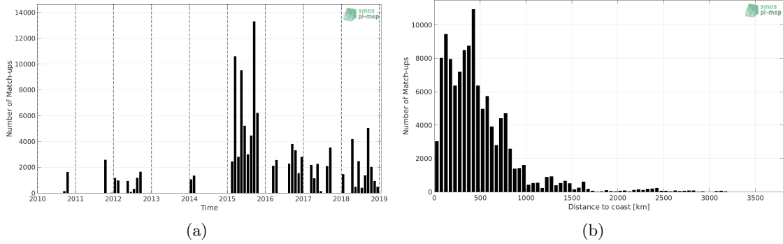
Figure 1: Number of match-ups between TSG-GOSUD-Research-vessel and SMOS L2Q v321 - 0.25 Deg (CATDS-CPDC) SSS as a function of time (a) and as function of the distance to coast (b) over the South Pacific Ocean Pi-MEP region and for the full satellite product period.
