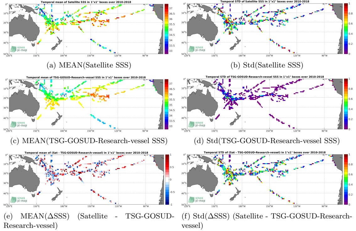
Figure 6: Temporal mean (left) and Std (right) of SSS from SMOS L2Q v321 - 0.25 Deg (CATDS-CPDC) (top), TSG-GOSUD-Research-vessel (middle), and of \Delta SSS (Satellite - TSG-GOSUD-Research-vessel). Only match-up pairs are used to generate these maps.
