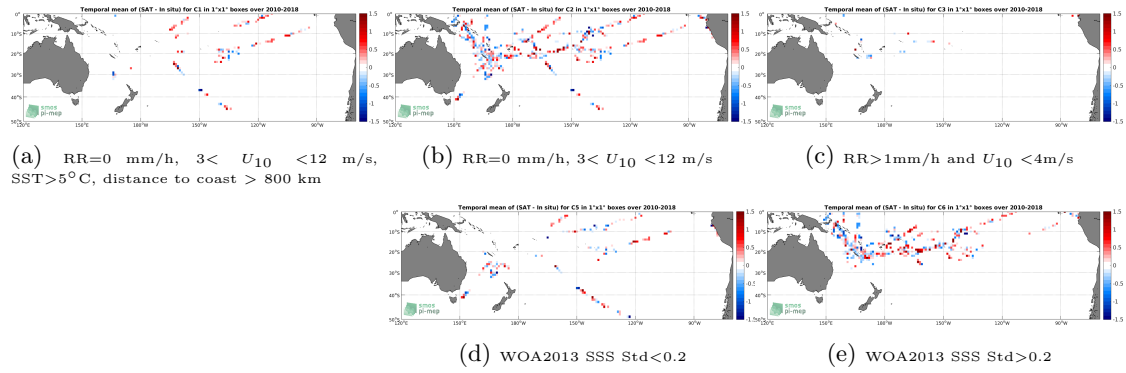
Figure 12: Temporal mean gridded over spatial boxes of size 1^\circ \times 1^\circ of \Delta SSS (SMOS L2Q v321 - 0.25 Deg (CATDS-CPDC) - TSG-GOSUD-Research-vessel) for 5 different subdatasets corresponding to: RR=0 mm/h, 3 < U_{10} < 12 m/s, SST >5^\circ\text{C} , distance to coast > 800 km (a), RR=0 mm/h, 3 < U_{10} < 12 m/s (b), RR >1 mm/h and U_{10} < 4 m/s (c), WOA2013 SSS Std <0.2 (d), WOA2013 SSS Std >0.2 (e).
