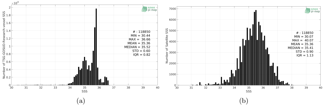
Figure 2: Histograms of SSS from TSG-GOSUD-Research-vessel (a) and SMOS L2Q v321 - 0.25 Deg (CATDS-CPDC) (b) considering all match-up pairs per bins of 0.1 over the South Pacific Ocean Pi-MEP region and for the full satellite product period.
