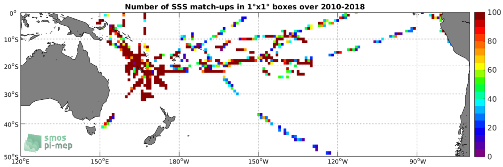
Figure 4: Number of SSS match-ups between TSG-GOSUD-Research-vessel SSS and the SMOS L2Q v321 - 0.25 Deg (CATDS-CPDC) SSS product for the South Pacific Ocean Pi-MEP region over 1°x1° boxes and for the full satellite product period.
