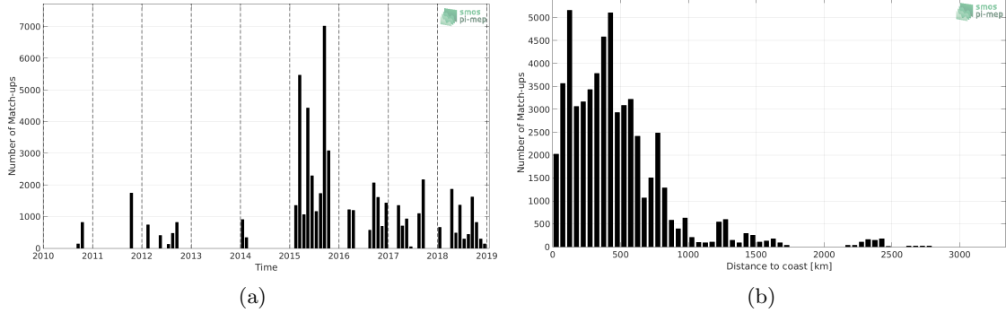
Figure 1: Number of match-ups between TSG-GOSUD-Research-vessel and SMOS-L3-CATDS-CPDC-V321-L2Q SSS as a function of time (a) and as function of the distance to coast (b) over the South Pacific Ocean Pi-MEP region and for the full satellite product period.
