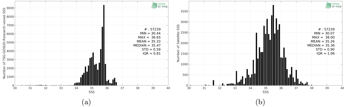
Figure 2: Histograms of SSS from TSG-GOSUD-Research-vessel (a) and SMOS-L3-CATDS-CPDC-V321-L2Q (b) considering all match-up pairs per bins of 0.1 over the South Pacific Ocean Pi-MEP region and for the full satellite product period.
