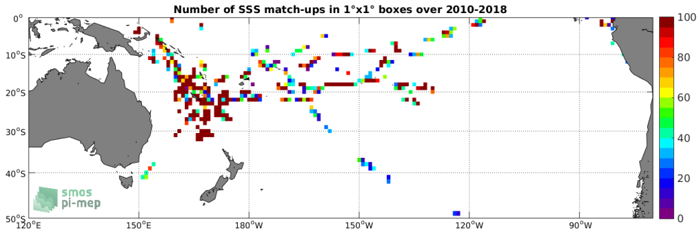
Figure 4: Number of SSS match-ups between TSG-GOSUD-Research-vessel SSS and the SMOS-L3-CATDS-CPDC-V321-L2Q SSS product for the South Pacific Ocean Pi-MEP region over 1°x1° boxes and for the full satellite product period.
