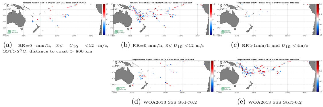
Figure 12: Temporal mean gridded over spatial boxes of size 1^\circ \times 1^\circ of \Delta SSS (SMOS-L3-CATDS-CPDC-V321-L2Q - TSG-GOSUD-Research-vessel) for 5 different subdatasets corresponding to: RR=0 mm/h, 3 < U_{10} < 12 m/s, SST > 5^\circ C , distance to coast > 800 km (a), RR=0 mm/h, 3 < U_{10} < 12 m/s (b), RR > 1 mm/h and U_{10} < 4 m/s (c), WOA2013 SSS Std < 0.2 (d), WOA2013 SSS Std > 0.2 (e).
