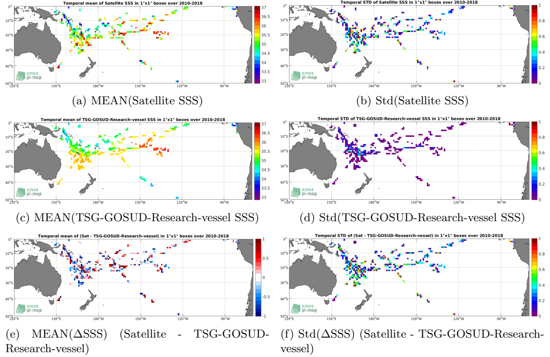
Figure 6: Temporal mean (left) and Std (right) of SSS from SMOS-L3-CATDS-CPDC-V321-L2Q (top), TSG-GOSUD-Research-vessel (middle), and of \Delta SSS (Satellite - TSG-GOSUD-Research-vessel). Only match-up pairs are used to generate these maps.
