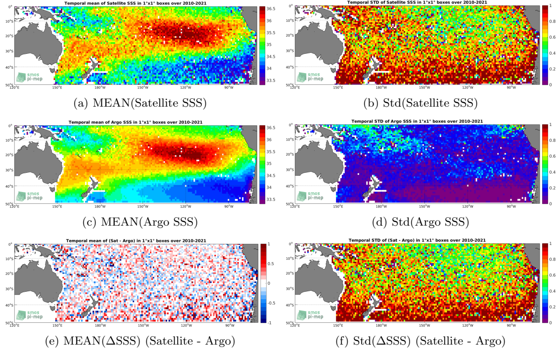
Figure 6: Temporal mean (left) and Std (right) of SSS from SMOS SSS L2Q v321 - 0.25 Deg (CATDS-CPDC) (top), Argo (middle), and of \Delta SSS (Satellite - Argo). Only match-up pairs are used to generate these maps.
