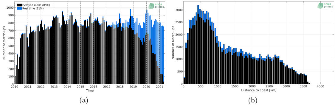
Figure 1: Number of match-ups between Argo and SMOS SSS L2Q v321 - 0.25 Deg (CATDS-CPDC) SSS as a function of time (a) and as function of the distance to coast (b) over the South Pacific Ocean Pi-MEP region and for the full satellite product period.
