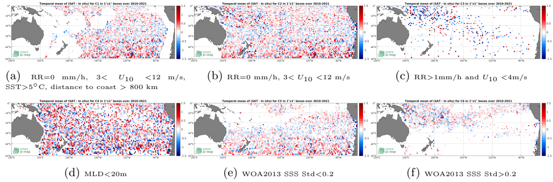
Figure 12: Temporal mean gridded over spatial boxes of size 1^\circ \times 1^\circ of \Delta SSS (SMOS SSS L2Q v321 - 0.25 Deg (CATDS-CPDC) - Argo) for 6 different subdatasets corresponding to: RR=0 mm/h, 3 < U_{10} < 12 m/s, SST > 5^\circ C , distance to coast > 800 km (a), RR=0 mm/h, 3 < U_{10} < 12 m/s (b), RR > 1 mm/h and U_{10} < 4 m/s (c), MLD < 20 m (d), WOA2013 SSS Std < 0.2 (e), WOA2013 SSS Std > 0.2 (f).
