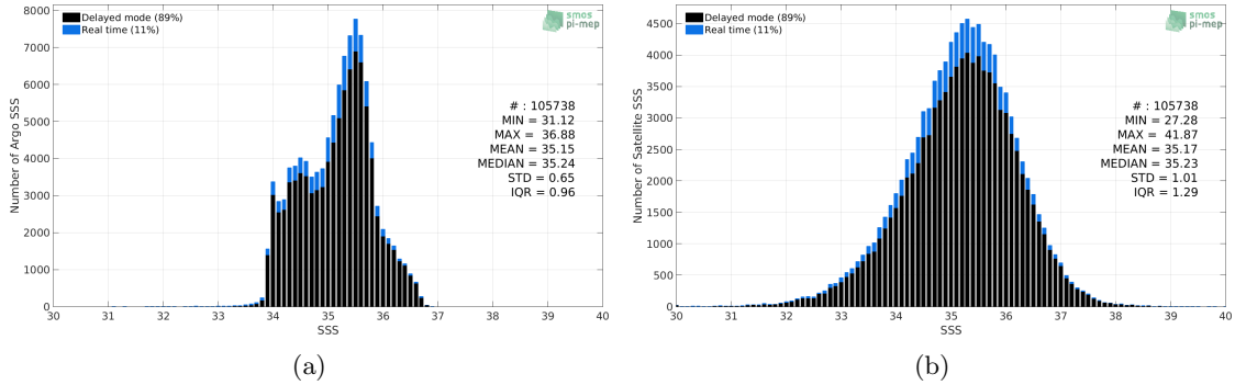
Figure 2: Histograms of SSS from Argo (a) and SMOS SSS L2Q v321 - 0.25 Deg (CATDS-CPDC) (b) considering all match-up pairs per bins of 0.1 over the South Pacific Ocean Pi-MEP region and for the full satellite product period.
