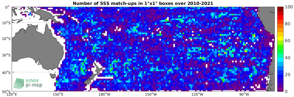
Figure 4: Number of SSS match-ups between Argo SSS and the SMOS SSS L2Q v321 - 0.25 Deg (CATDS-CPDC) SSS product for the South Pacific Ocean Pi-MEP region over 1^\circ \times 1^\circ boxes and for the full satellite product period.
