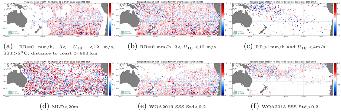
Figure 12: Temporal mean gridded over spatial boxes of size 1^\circ \times 1^\circ of \Delta SSS (SMOS L2Q v321 - 0.25 Deg (CATDS-CPDC) - Argo) for 6 different subdatasets corresponding to: RR=0 mm/h, 3 < U_{10} < 12 m/s, SST > 5^\circ C , distance to coast > 800 km (a), RR=0 mm/h, 3 < U_{10} < 12 m/s (b), RR > 1 mm/h and U_{10} < 4 m/s (c), MLD < 20 m (d), WOA2013 SSS Std < 0.2 (e), WOA2013 SSS Std > 0.2 (f).
