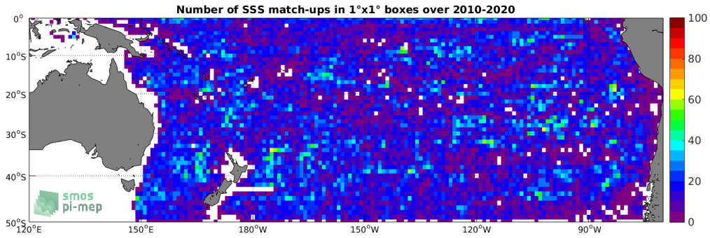
Figure 4: Number of SSS match-ups between Argo SSS and the SMOS L2Q v321 - 0.25 Deg (CATDS-CPDC) SSS product for the South Pacific Ocean Pi-MEP region over 1°x1° boxes and for the full satellite product period.
