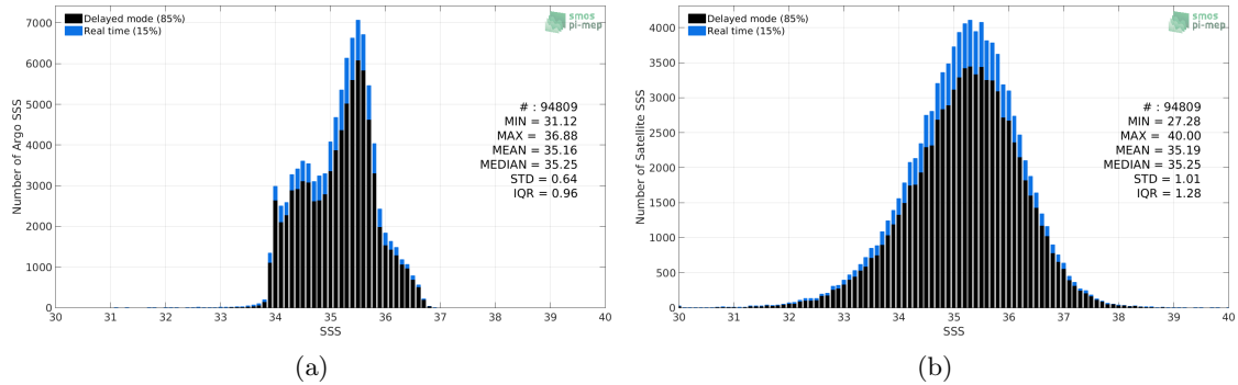
Figure 2: Histograms of SSS from Argo (a) and SMOS L2Q v321 - 0.25 Deg (CATDS-CPDC) (b) considering all match-up pairs per bins of 0.1 over the South Pacific Ocean Pi-MEP region and for the full satellite product period.
