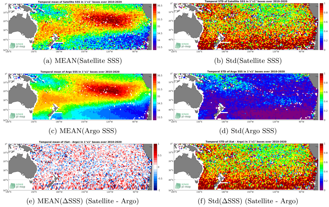
Figure 6: Temporal mean (left) and Std (right) of SSS from SMOS L2Q v321 - 0.25 Deg (CATDS-CPDC) (top), Argo (middle), and of \Delta SSS (Satellite - Argo). Only match-up pairs are used to generate these maps.
