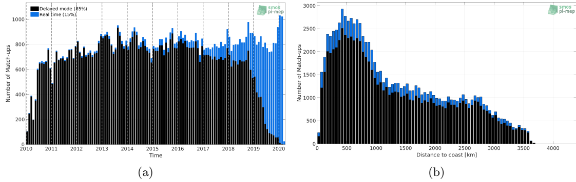
Figure 1: Number of match-ups between Argo and SMOS L2Q v321 - 0.25 Deg (CATDS-CPDC) SSS as a function of time (a) and as function of the distance to coast (b) over the South Pacific Ocean Pi-MEP region and for the full satellite product period.
