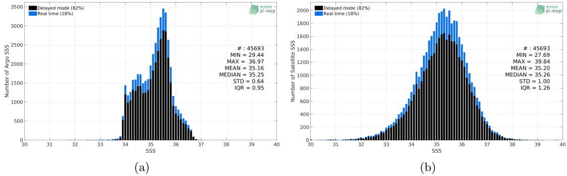
Figure 2: Histograms of SSS from Argo (a) and SMOS-L3-CATDS-CPDC-V321-L2Q (b) considering all match-up pairs per bins of 0.1 over the South Pacific Ocean Pi-MEP region and for the full satellite product period.
