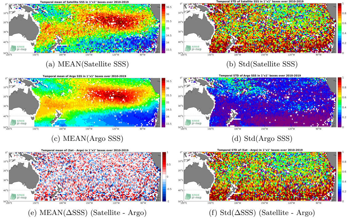
Figure 6: Temporal mean (left) and Std (right) of SSS from SMOS-L3-CATDS-CPDC-V321-L2Q (top), Argo (middle), and of \Delta SSS (Satellite - Argo). Only match-up pairs are used to generate these maps.
