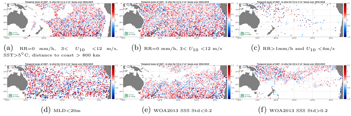
Figure 12: Temporal mean gridded over spatial boxes of size 1^\circ \times 1^\circ of \Delta SSS (SMOS-L3-CATDS-CPDC-V321-L2Q - Argo) for 6 different subdatasets corresponding to: RR=0 mm/h, 3 < U_{10} < 12 m/s, SST > 5^\circ C , distance to coast > 800 km (a), RR=0 mm/h, 3 < U_{10} < 12 m/s (b), RR > 1 mm/h and U_{10} < 4 m/s (c), MLD < 20 m (d), WOA2013 SSS Std < 0.2 (e), WOA2013 SSS Std > 0.2 (f).
