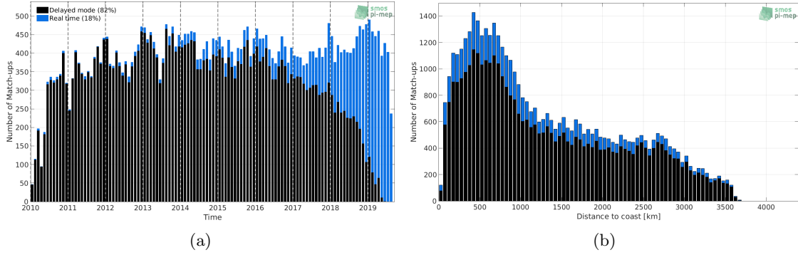
Figure 1: Number of match-ups between Argo and SMOS-L3-CATDS-CPDC-V321-L2Q SSS as a function of time (a) and as function of the distance to coast (b) over the South Pacific Ocean Pi-MEP region and for the full satellite product period.
