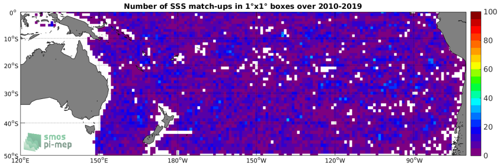
Figure 4: Number of SSS match-ups between Argo SSS and the SMOS-L3-CATDS-CPDC-V321-L2Q SSS product for the South Pacific Ocean Pi-MEP region over 1^\circ \times 1^\circ boxes and for the full satellite product period.
