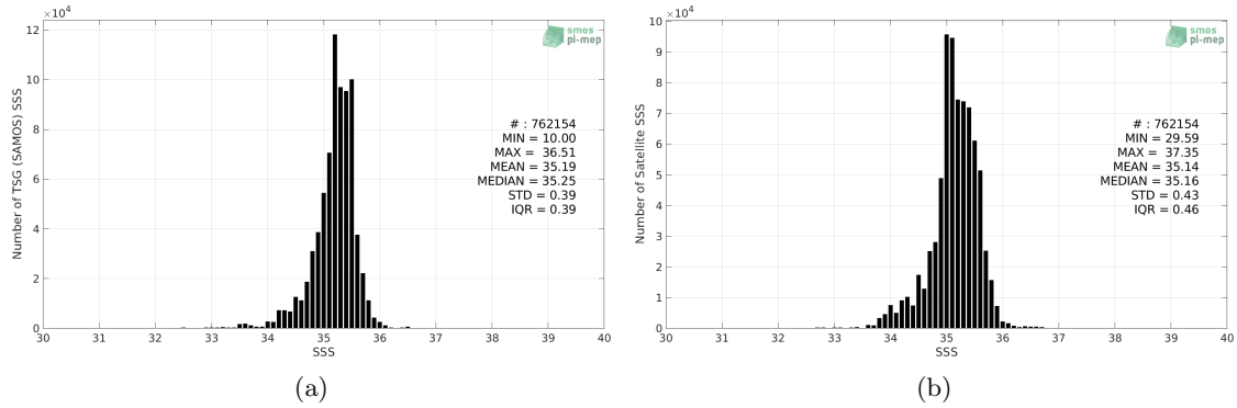
Figure 2: Histograms of SSS from TSG (SAMOS) (a) and SMOS SSS L3 v317 - Monthly - 25 km (CATDS-CPDC) (b) considering all match-up pairs per bins of 0.1 over the South Pacific Ocean Pi-MEP region and for the full satellite product period.
