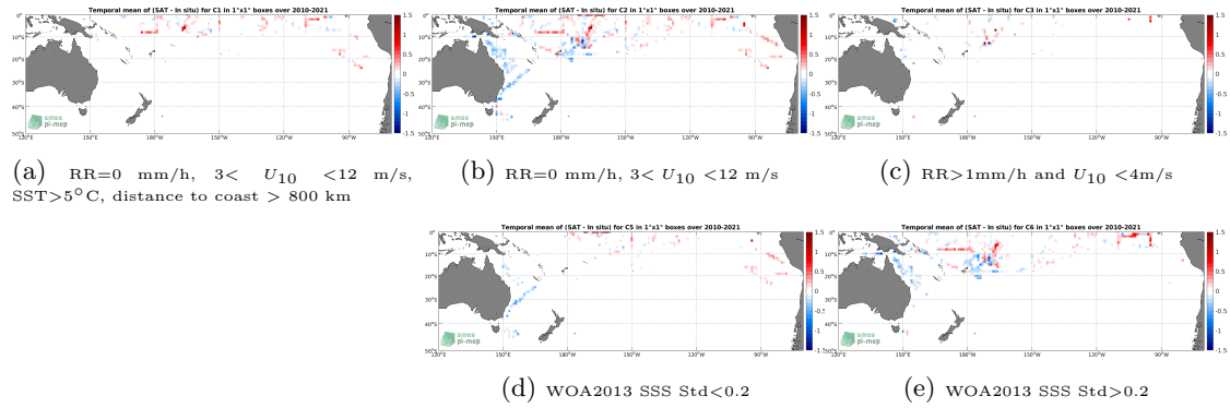
Figure 12: Temporal mean gridded over spatial boxes of size 1^\circ \times 1^\circ of \Delta SSS (SMOS SSS L3 v317 - Monthly - 25 km (CATDS-CPDC) - TSG (SAMOS)) for 5 different subdatasets corresponding to: RR=0 mm/h, 3 < U_{10} < 12 m/s, SST > 5^\circ C , distance to coast > 800 km (a), RR=0 mm/h, 3 < U_{10} < 12 m/s (b), RR > 1 mm/h and U_{10} < 4 m/s (c), WOA2013 SSS Std < 0.2 (d), WOA2013 SSS Std > 0.2 (e).
