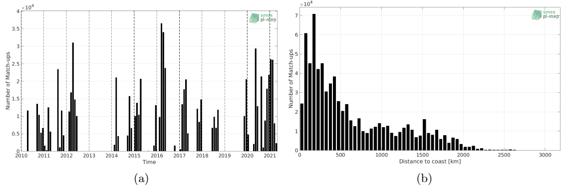
Figure 1: Number of match-ups between TSG (SAMOS) and SMOS SSS L3 v317 - Monthly - 25 km (CATDS-CPDC) SSS as a function of time (a) and as function of the distance to coast (b) over the South Pacific Ocean Pi-MEP region and for the full satellite product period.
