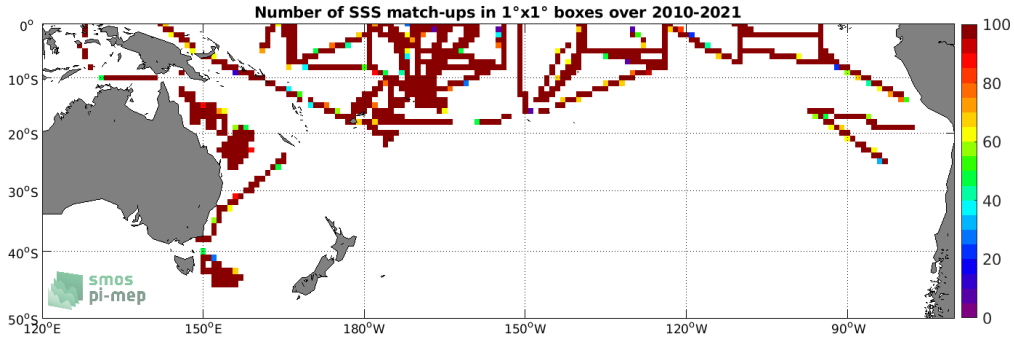
Figure 4: Number of SSS match-ups between TSG (SAMOS) SSS and the SMOS SSS L3 v317 - Monthly - 25 km (CATDS-CPDC) SSS product for the South Pacific Ocean Pi-MEP region over 1^\circ \times 1^\circ boxes and for the full satellite product period.
