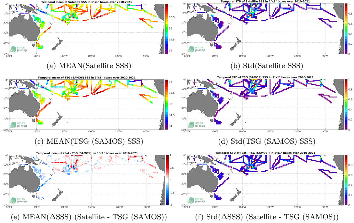
Figure 6: Temporal mean (left) and Std (right) of SSS from SMOS SSS L3 v317 - Monthly - 25 km (CATDS-CPDC) (top), TSG (SAMOS) (middle), and of \Delta SSS (Satellite - TSG (SAMOS)). Only match-up pairs are used to generate these maps.
