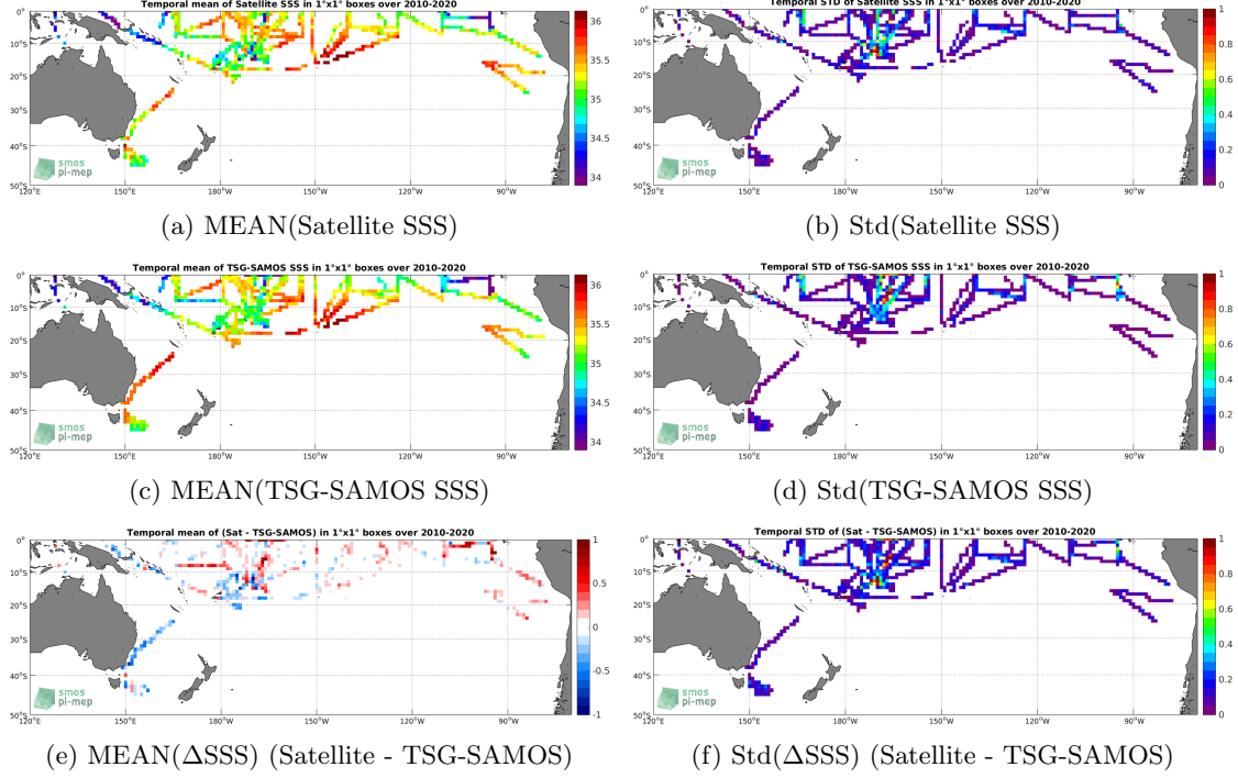
Figure 6: Temporal mean (left) and Std (right) of SSS from SMOS L3 v317 - Monthly - 25 km (CATDS-CPDC) (top), TSG-SAMOS (middle), and of \Delta SSS (Satellite - TSG-SAMOS). Only match-up pairs are used to generate these maps.
