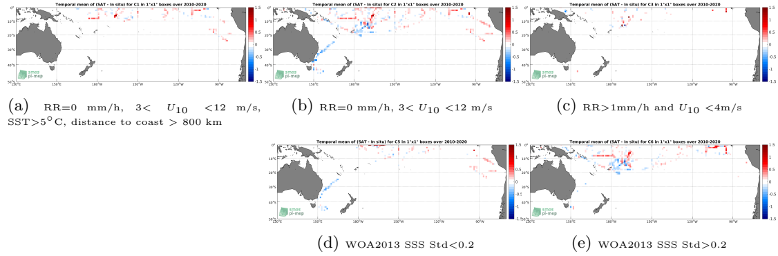
Figure 12: Temporal mean gridded over spatial boxes of size 1^\circ \times 1^\circ of \Delta SSS (SMOS L3 v317 - Monthly - 25 km (CATDS-CPDC) - TSG-SAMOS) for 5 different subdatasets corresponding to: RR=0 mm/h, 3 < U_{10} < 12 m/s, SST > 5^\circ C , distance to coast > 800 km (a), RR=0 mm/h, 3 < U_{10} < 12 m/s (b), RR > 1 mm/h and U_{10} < 4 m/s (c), WOA2013 SSS Std < 0.2 (d), WOA2013 SSS Std > 0.2 (e).
