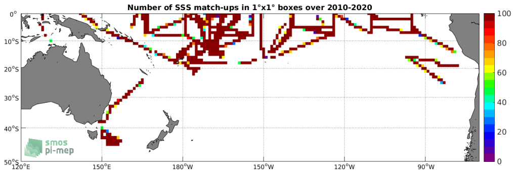
Figure 4: Number of SSS match-ups between TSG-SAMOS SSS and the SMOS L3 v317 - Monthly - 25 km (CATDS-CPDC) SSS product for the South Pacific Ocean Pi-MEP region over 1°x1° boxes and for the full satellite product period.
