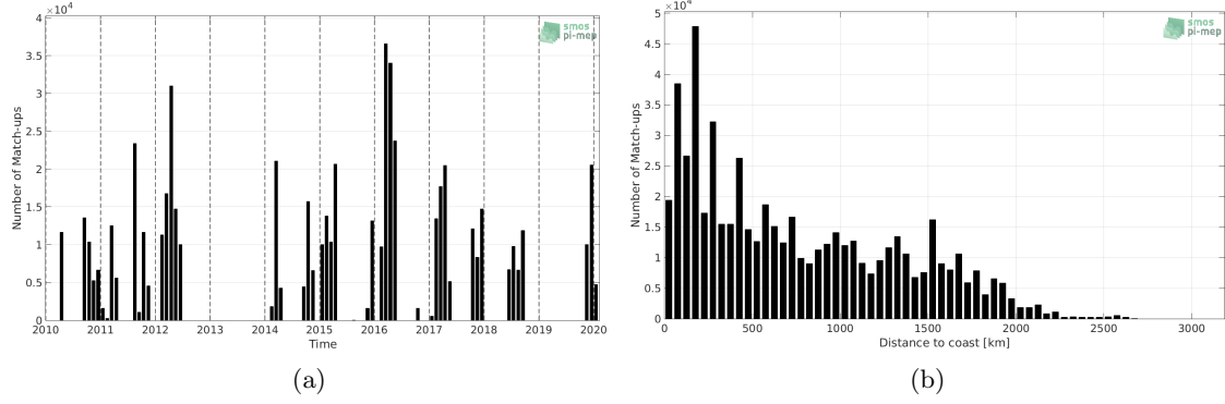
Figure 1: Number of match-ups between TSG-SAMOS and SMOS L3 v317 - Monthly - 25 km (CATDS-CPDC) SSS as a function of time (a) and as function of the distance to coast (b) over the South Pacific Ocean Pi-MEP region and for the full satellite product period.
