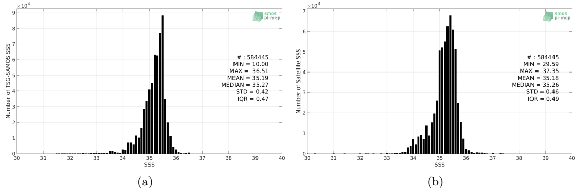
Figure 2: Histograms of SSS from TSG-SAMOS (a) and SMOS L3 v317 - Monthly - 25 km (CATDS-CPDC) (b) considering all match-up pairs per bins of 0.1 over the South Pacific Ocean Pi-MEP region and for the full satellite product period.
