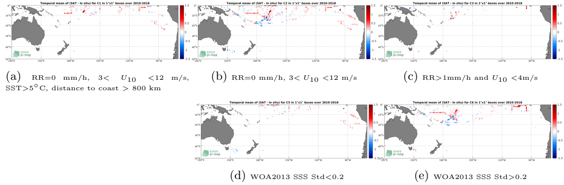
Figure 12: Temporal mean gridded over spatial boxes of size 1^\circ \times 1^\circ of \Delta SSS (SMOS-L3-CATDS-CPDC-V317-MONTHLY-25KM - TSG-SAMOS) for 5 different subdatasets corresponding to: RR=0 mm/h, 3 < U_{10} < 12 m/s, SST > 5^\circ C , distance to coast > 800 km (a), RR=0 mm/h, 3 < U_{10} < 12 m/s (b), RR > 1 mm/h and U_{10} < 4 m/s (c), WOA2013 SSS Std < 0.2 (d), WOA2013 SSS Std > 0.2 (e).
