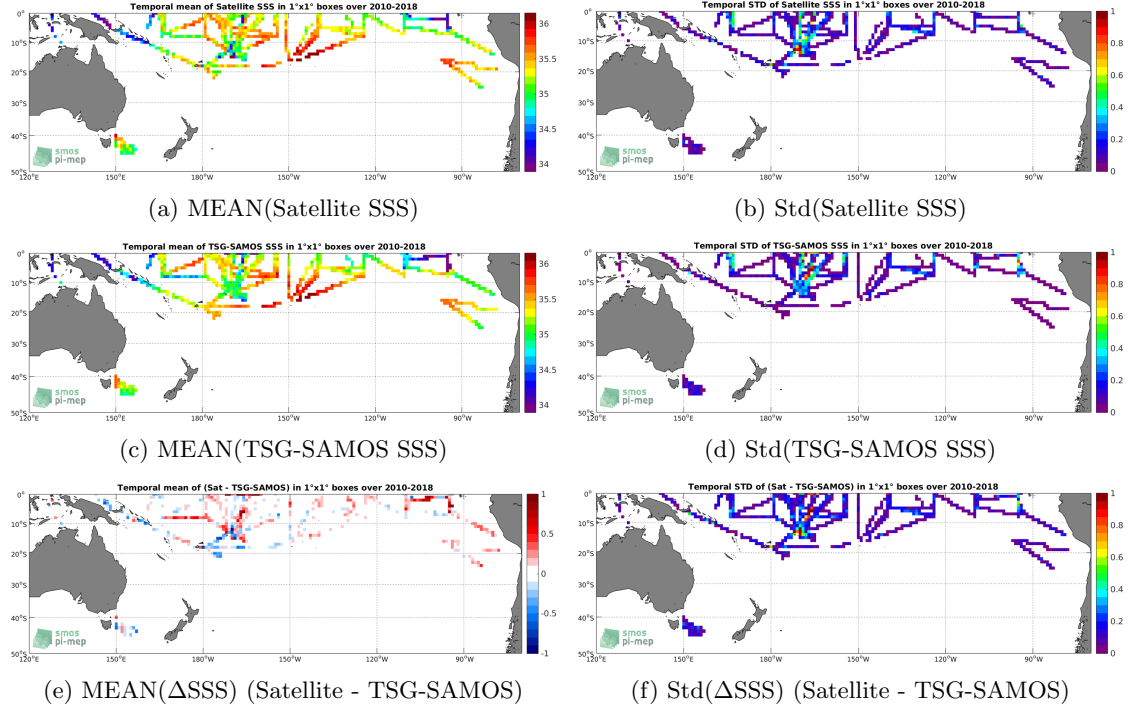
Figure 6: Temporal mean (left) and Std (right) of SSS from SMOS-L3-CATDS-CPDC-V317-MONTHLY-25KM (top), TSG-SAMOS (middle), and of \Delta SSS (Satellite - TSG-SAMOS). Only match-up pairs are used to generate these maps.
