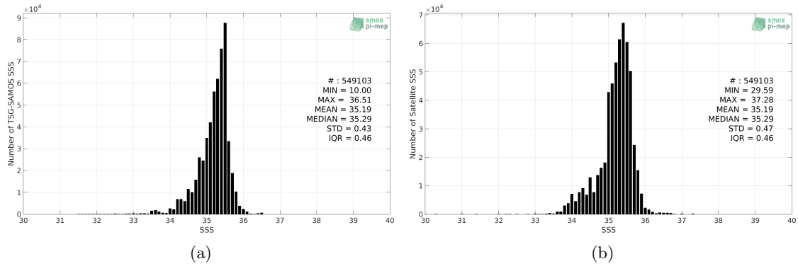
Figure 2: Histograms of SSS from TSG-SAMOS (a) and SMOS-L3-CATDS-CPDC-V317-MONTHLY-25KM (b) considering all match-up pairs per bins of 0.1 over the South Pacific Ocean Pi-MEP region and for the full satellite product period.
