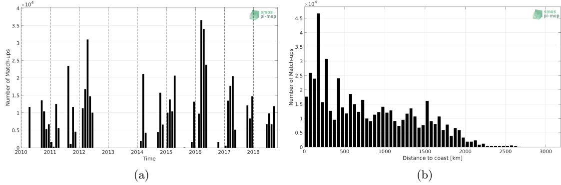
Figure 1: Number of match-ups between TSG-SAMOS and SMOS-L3-CATDS-CPDC-V317-MONTHLY-25KM SSS as a function of time (a) and as function of the distance to coast (b) over the South Pacific Ocean Pi-MEP region and for the full satellite product period.
