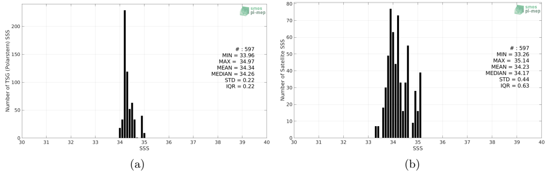
Figure 2: Histograms of SSS from TSG (Polarstern) (a) and SMOS SSS L3 v317 - Monthly - 25 km (CATDS-CPDC) (b) considering all match-up pairs per bins of 0.1 over the South Pacific Ocean Pi-MEP region and for the full satellite product period.
