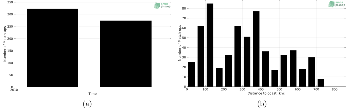
Figure 1: Number of match-ups between TSG (Polarstern) and SMOS SSS L3 v317 - Monthly - 25 km (CATDS-CPDC) SSS as a function of time (a) and as function of the distance to coast (b) over the South Pacific Ocean Pi-MEP region and for the full satellite product period.
