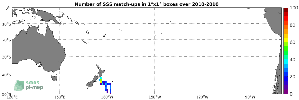
Figure 4: Number of SSS match-ups between TSG (Polarstern) SSS and the SMOS SSS L3 v317 - Monthly - 25 km (CATDS-CPDC) SSS product for the South Pacific Ocean Pi-MEP region over 1^\circ \times 1^\circ boxes and for the full satellite product period.
