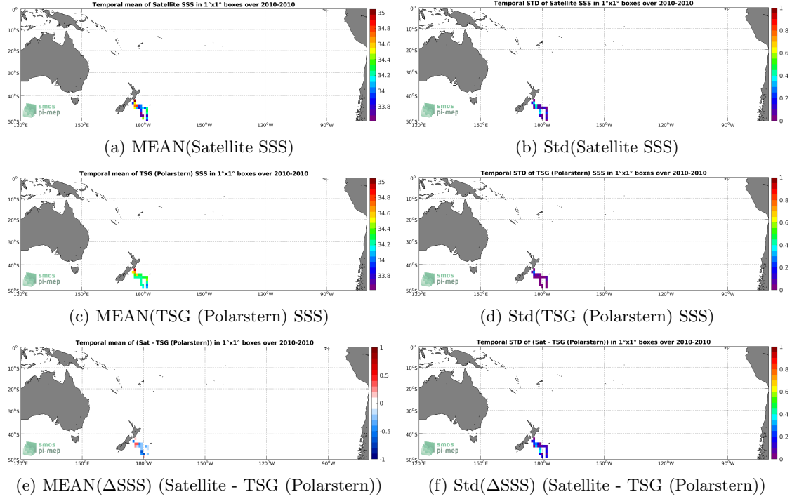
Figure 6: Temporal mean (left) and Std (right) of SSS from SMOS SSS L3 v317 - Monthly - 25 km (CATDS-CPDC) (top), TSG (Polarstern) (middle), and of \Delta SSS (Satellite - TSG (Polarstern)). Only match-up pairs are used to generate these maps.
