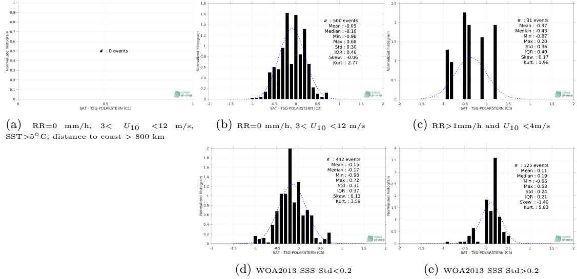
Figure 13: Normalized histogram of \Delta\text{SSS} (SMOS L3 v317 - Monthly - 25 km (CATDS-CPDC) - TSG-POLARSTERN) for 5 different subdatasets corresponding to: RR=0 mm/h, 3 < U_{10} < 12 m/s, SST > 5^\circ\text{C} , distance to coast > 800 km (a), RR=0 mm/h, 3 < U_{10} < 12 m/s (b), RR > 1\text{mm/h} and U_{10} < 4\text{m/s} (c), WOA2013 SSS Std <0.2 (d), WOA2013 SSS Std >0.2 (e).
