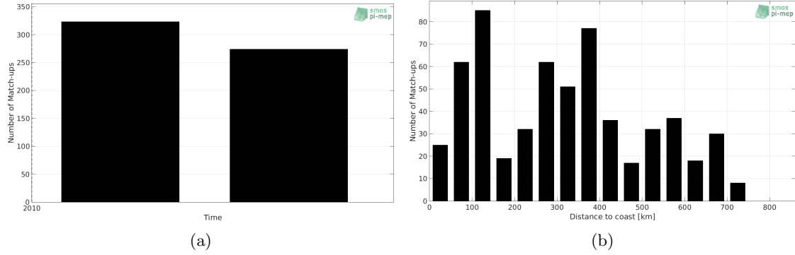
Figure 1: Number of match-ups between TSG-POLARSTERN and SMOS L3 v317 - Monthly - 25 km (CATDS-CPDC) SSS as a function of time (a) and as function of the distance to coast (b) over the South Pacific Ocean Pi-MEP region and for the full satellite product period.
