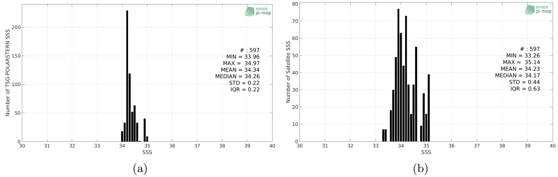
Figure 2: Histograms of SSS from TSG-POLARSTERN (a) and SMOS L3 v317 - Monthly - 25 km (CATDS-CPDC) (b) considering all match-up pairs per bins of 0.1 over the South Pacific Ocean Pi-MEP region and for the full satellite product period.
