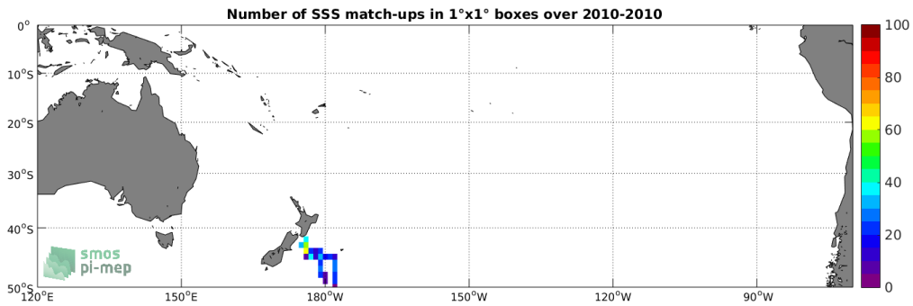
Figure 4: Number of SSS match-ups between TSG-POLARSTERN SSS and the SMOS L3 v317 - Monthly - 25 km (CATDS-CPDC) SSS product for the South Pacific Ocean Pi-MEP region over 1°x1° boxes and for the full satellite product period.
