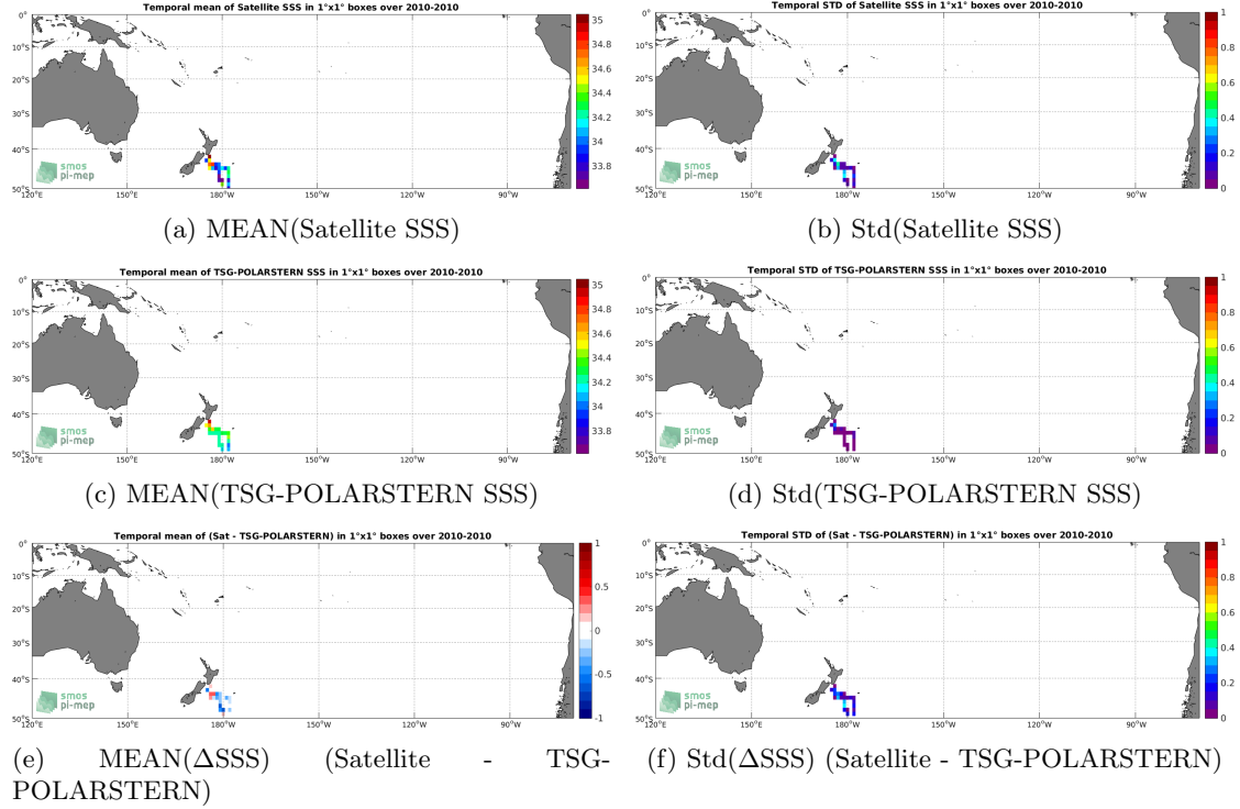
Figure 6: Temporal mean (left) and Std (right) of SSS from SMOS L3 v317 - Monthly - 25 km (CATDS-CPDC) (top), TSG-POLARSTERN (middle), and of \Delta SSS (Satellite - TSG-POLARSTERN). Only match-up pairs are used to generate these maps.
