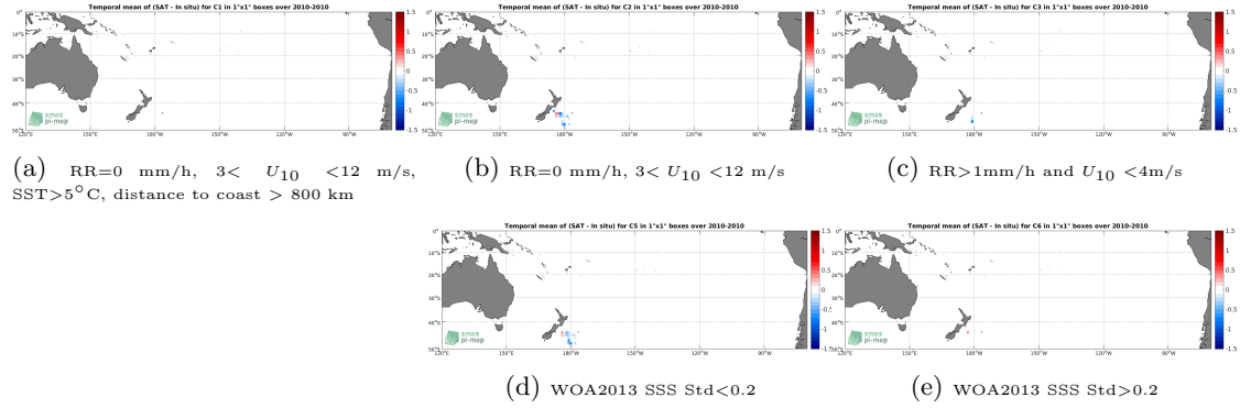
Figure 12: Temporal mean gridded over spatial boxes of size 1^\circ \times 1^\circ of \Delta SSS (SMOS-L3-CATDS-CPDC-V317-MONTHLY-25KM - TSG-POLARSTERN) for 5 different subdatasets corresponding to: RR=0 mm/h, 3 < U_{10} < 12 m/s, SST > 5^\circ C , distance to coast > 800 km (a), RR=0 mm/h, 3 < U_{10} < 12 m/s (b), RR > 1 mm/h and U_{10} < 4 m/s (c), WOA2013 SSS Std < 0.2 (d), WOA2013 SSS Std > 0.2 (e).
