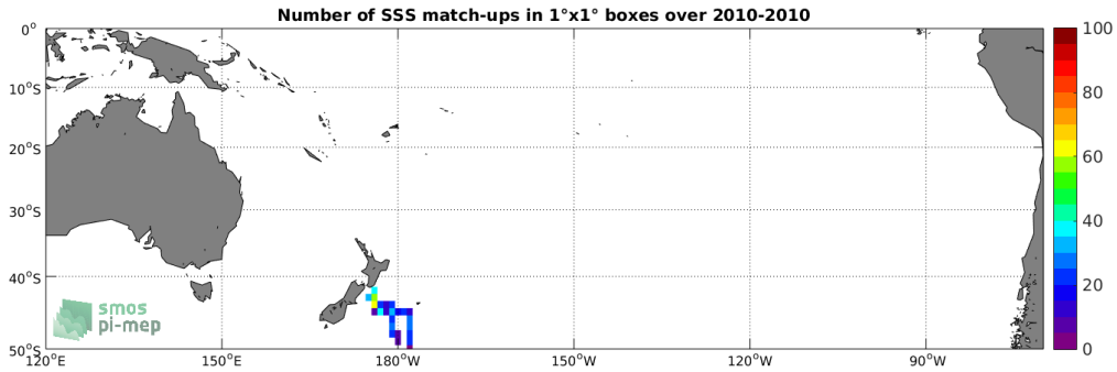
Figure 4: Number of SSS match-ups between TSG-POLARSTERN SSS and the SMOS-L3-CATDS-CPDC-V317-MONTHLY-25KM SSS product for the South Pacific Ocean Pi-MEP region over 1°x1° boxes and for the full satellite product period.
