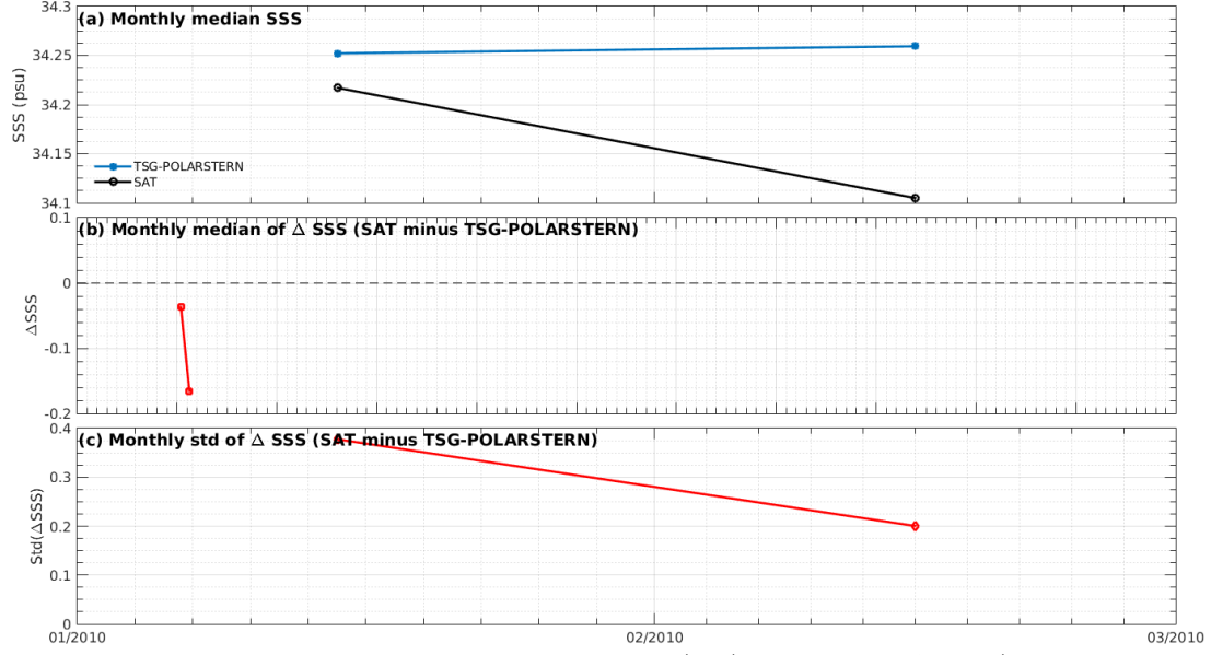
Figure 7: Time series of the monthly median SSS (top), median of \Delta SSS (Satellite - TSG-POLARSTERN) and Std of \Delta SSS (Satellite - TSG-POLARSTERN) over the South Pacific Ocean Pi-MEP region considering all match-ups collected by the Pi-MEP.
