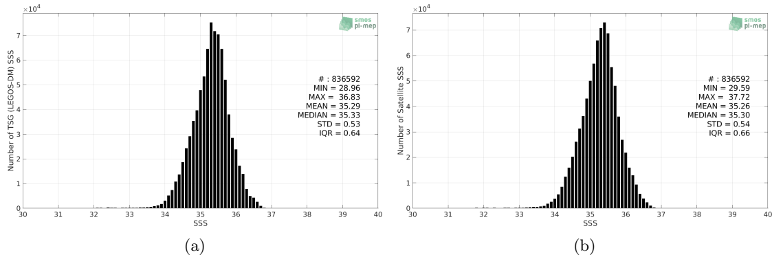
Figure 2: Histograms of SSS from TSG (LEGOS-DM) (a) and SMOS SSS L3 v317 - Monthly - 25 km (CATDS-CPDC) (b) considering all match-up pairs per bins of 0.1 over the South Pacific Ocean Pi-MEP region and for the full satellite product period.
