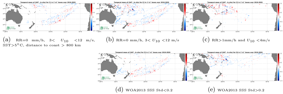
Figure 12: Temporal mean gridded over spatial boxes of size 1^\circ \times 1^\circ of \Delta SSS (SMOS SSS L3 v317 - Monthly - 25 km (CATDS-CPDC) - TSG (LEGOS-DM)) for 5 different subdatasets corresponding to: RR=0 mm/h, 3 < U_{10} < 12 m/s, SST > 5^\circ C , distance to coast > 800 km (a), RR=0 mm/h, 3 < U_{10} < 12 m/s (b), RR > 1 mm/h and U_{10} < 4 m/s (c), WOA2013 SSS Std < 0.2 (d), WOA2013 SSS Std > 0.2 (e).
