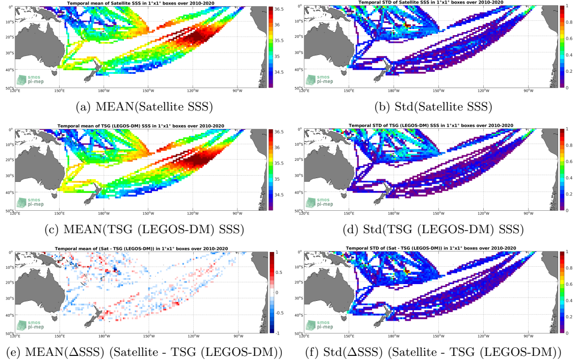
Figure 6: Temporal mean (left) and Std (right) of SSS from SMOS SSS L3 v317 - Monthly - 25 km (CATDS-CPDC) (top), TSG (LEGOS-DM) (middle), and of \Delta SSS (Satellite - TSG (LEGOS-DM)). Only match-up pairs are used to generate these maps.
