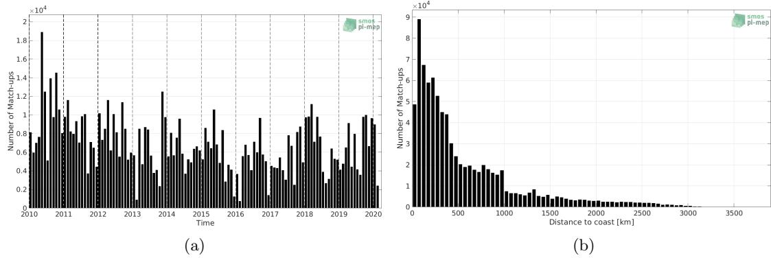
Figure 1: Number of match-ups between TSG (LEGOS-DM) and SMOS SSS L3 v317 - Monthly - 25 km (CATDS-CPDC) SSS as a function of time (a) and as function of the distance to coast (b) over the South Pacific Ocean Pi-MEP region and for the full satellite product period.
