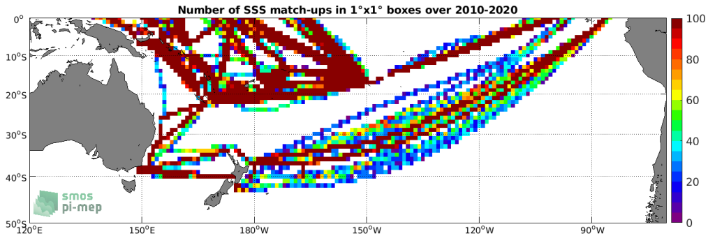
Figure 4: Number of SSS match-ups between TSG (LEGOS-DM) SSS and the SMOS SSS L3 v317 - Monthly - 25 km (CATDS-CPDC) SSS product for the South Pacific Ocean Pi-MEP region over 1^\circ \times 1^\circ boxes and for the full satellite product period.
