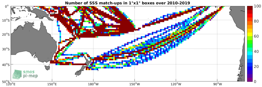
Figure 4: Number of SSS match-ups between TSG (LEGOS-DM) SSS and the SMOS SSS L3 v317 - Monthly - 25 km (CATDS-CPDC) SSS product for the South Pacific Ocean Pi-MEP region over 1°x1° boxes and for the full satellite product period.
