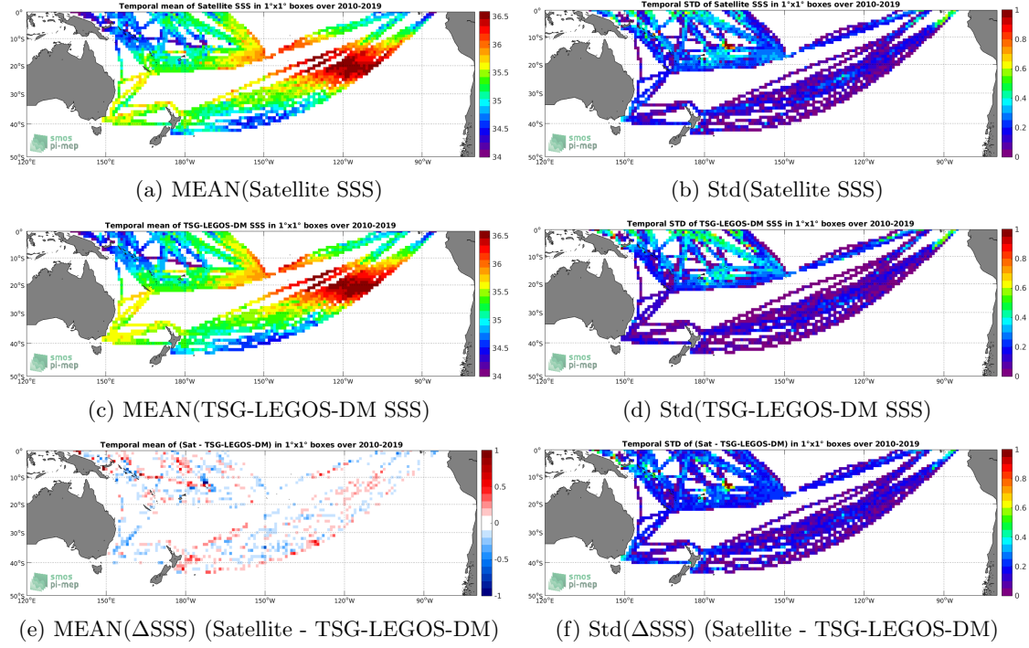
Figure 6: Temporal mean (left) and Std (right) of SSS from SMOS L3 v317 - Monthly - 25 km (CATDS-CPDC) (top), TSG-LEGOS-DM (middle), and of \Delta SSS (Satellite - TSG-LEGOS-DM). Only match-up pairs are used to generate these maps.
