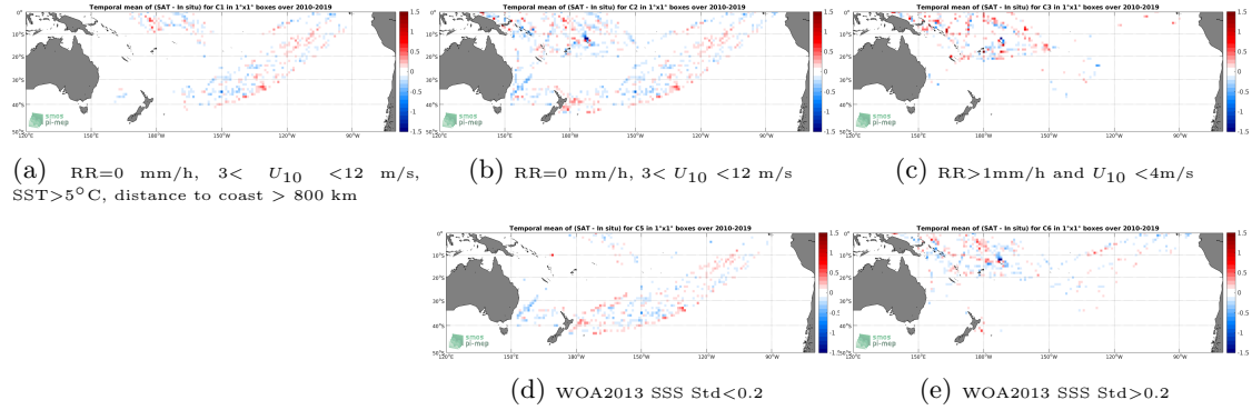
Figure 12: Temporal mean gridded over spatial boxes of size 1^\circ \times 1^\circ of \Delta SSS (SMOS L3 v317 - Monthly - 25 km (CATDS-CPDC) - TSG-LEGOS-DM) for 5 different subdatasets corresponding to: RR=0 mm/h, 3 < U_{10} < 12 m/s, SST > 5^\circ C , distance to coast > 800 km (a), RR=0 mm/h, 3 < U_{10} < 12 m/s (b), RR > 1 mm/h and U_{10} < 4 m/s (c), WOA2013 SSS Std < 0.2 (d), WOA2013 SSS Std > 0.2 (e).
