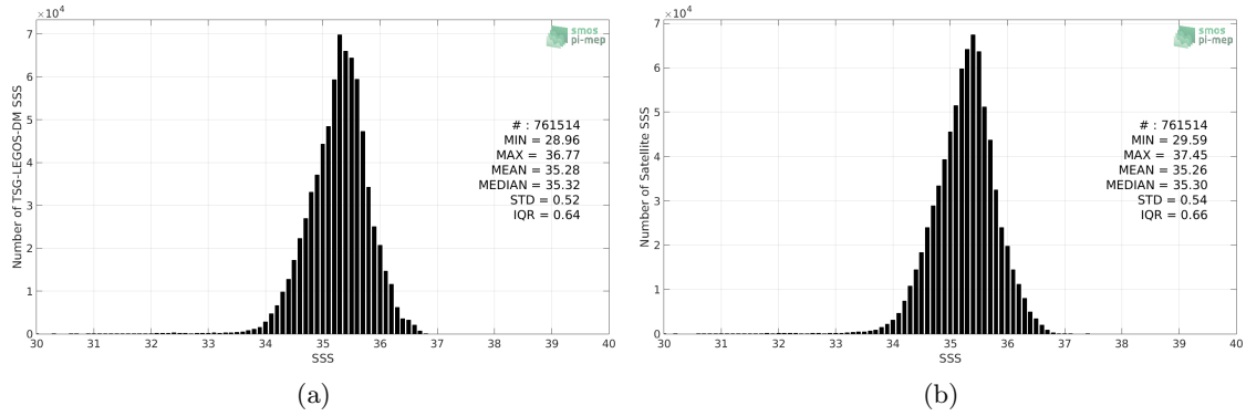
Figure 2: Histograms of SSS from TSG-LEGOS-DM (a) and SMOS L3 v317 - Monthly - 25 km (CATDS-CPDC) (b) considering all match-up pairs per bins of 0.1 over the South Pacific Ocean Pi-MEP region and for the full satellite product period.
