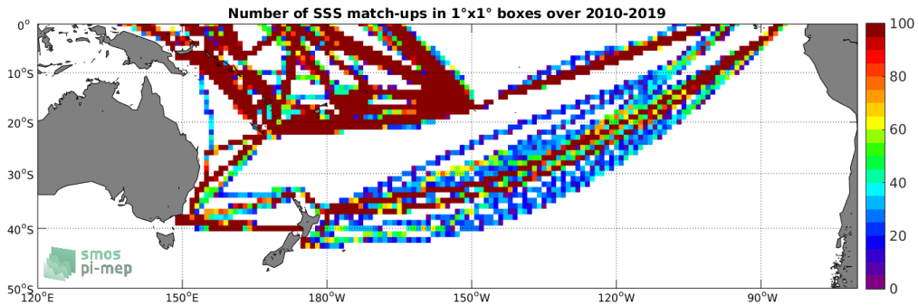
Figure 4: Number of SSS match-ups between TSG-LEGOS-DM SSS and the SMOS L3 v317 - Monthly - 25 km (CATDS-CPDC) SSS product for the South Pacific Ocean Pi-MEP region over 1°x1° boxes and for the full satellite product period.
