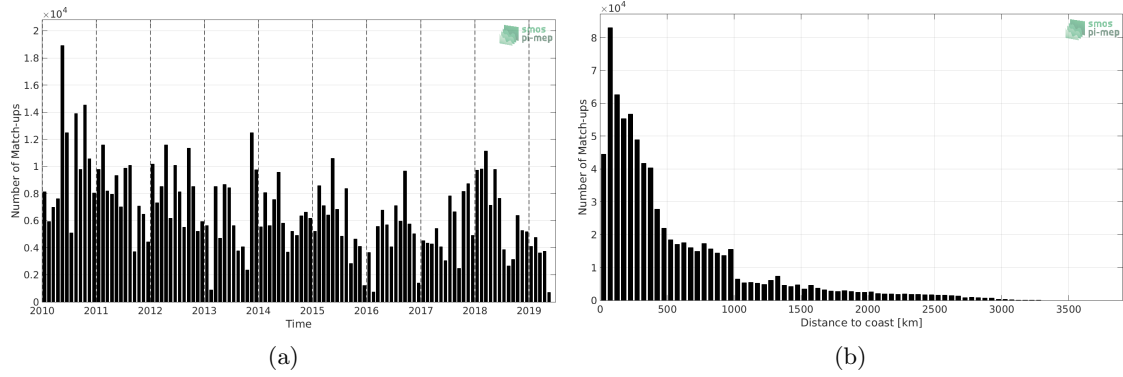
Figure 1: Number of match-ups between TSG-LEGOS-DM and SMOS L3 v317 - Monthly - 25 km (CATDS-CPDC) SSS as a function of time (a) and as function of the distance to coast (b) over the South Pacific Ocean Pi-MEP region and for the full satellite product period.
