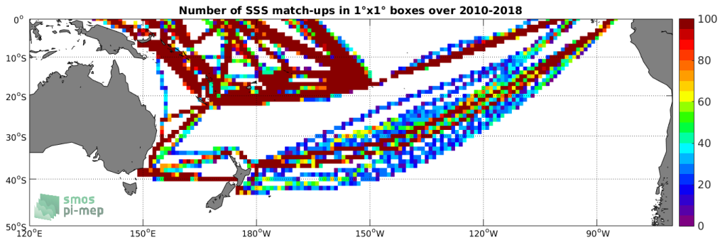
Figure 4: Number of SSS match-ups between TSG-LEGOS-DM SSS and the SMOS-L3-CATDS-CPDC-V317-MONTHLY-25KM SSS product for the South Pacific Ocean Pi-MEP region over 1°x1° boxes and for the full satellite product period.
