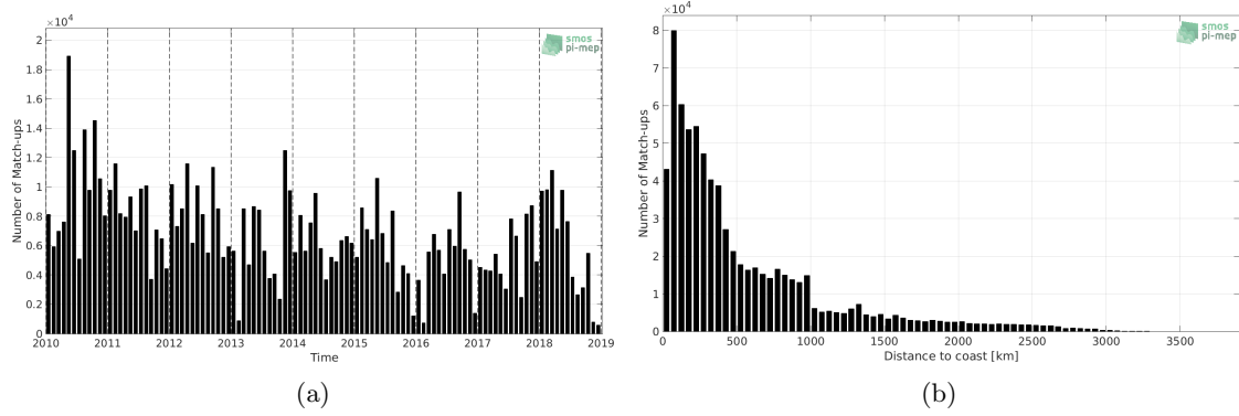
Figure 1: Number of match-ups between TSG-LEGOS-DM and SMOS-L3-CATDS-CPDC-V317-MONTHLY-25KM SSS as a function of time (a) and as function of the distance to coast (b) over the South Pacific Ocean Pi-MEP region and for the full satellite product period.
