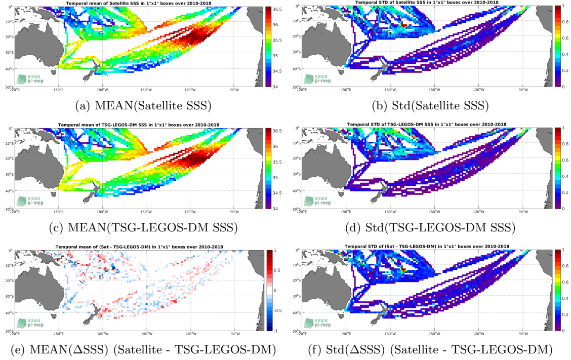
Figure 6: Temporal mean (left) and Std (right) of SSS from SMOS-L3-CATDS-CPDC-V317-MONTHLY-25KM (top), TSG-LEGOS-DM (middle), and of \Delta SSS (Satellite - TSG-LEGOS-DM). Only match-up pairs are used to generate these maps.
