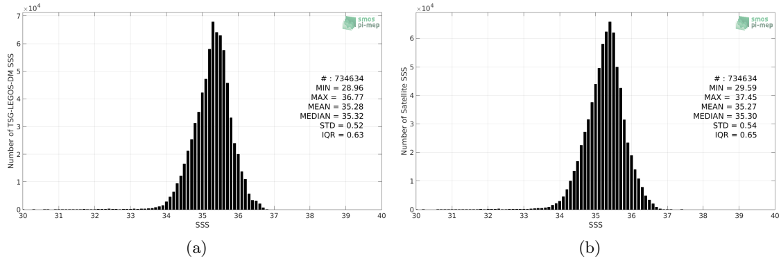
Figure 2: Histograms of SSS from TSG-LEGOS-DM (a) and SMOS-L3-CATDS-CPDC-V317-MONTHLY-25KM (b) considering all match-up pairs per bins of 0.1 over the South Pacific Ocean Pi-MEP region and for the full satellite product period.
