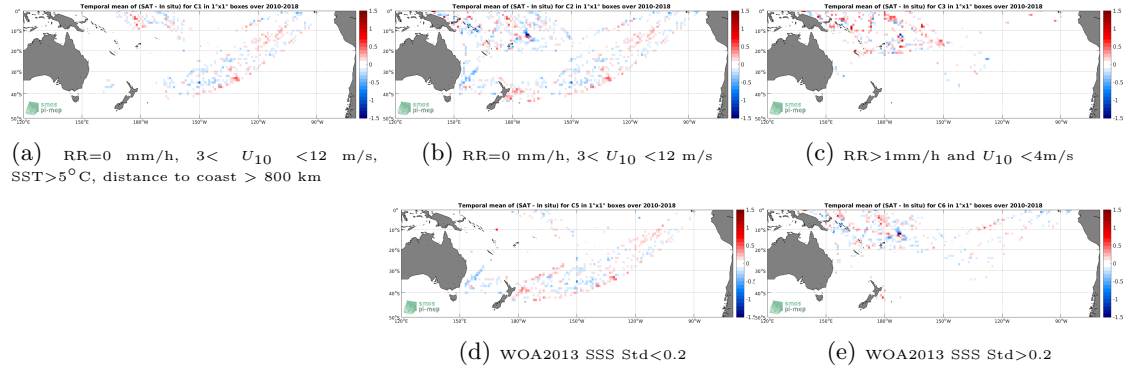
Figure 12: Temporal mean gridded over spatial boxes of size 1^\circ \times 1^\circ of \Delta SSS (SMOS-L3-CATDS-CPDC-V317-MONTHLY-25KM - TSG-LEGOS-DM) for 5 different subdatasets corresponding to: RR=0 mm/h, 3 < U_{10} < 12 m/s, SST > 5^\circ\text{C} , distance to coast > 800 km (a), RR=0 mm/h, 3 < U_{10} < 12 m/s (b), RR > 1 mm/h and U_{10} < 4 m/s (c), WOA2013 SSS Std < 0.2 (d), WOA2013 SSS Std > 0.2 (e).
