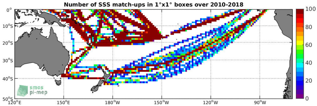
Figure 4: Number of SSS match-ups between TSG-LEGOS-DM SSS and the SMOS-L3-CATDS-CPDC-V317-MONTHLY-25KM SSS product for the South Pacific Ocean Pi-MEP region over 1^\circ \times 1^\circ boxes and for the full satellite product period.
