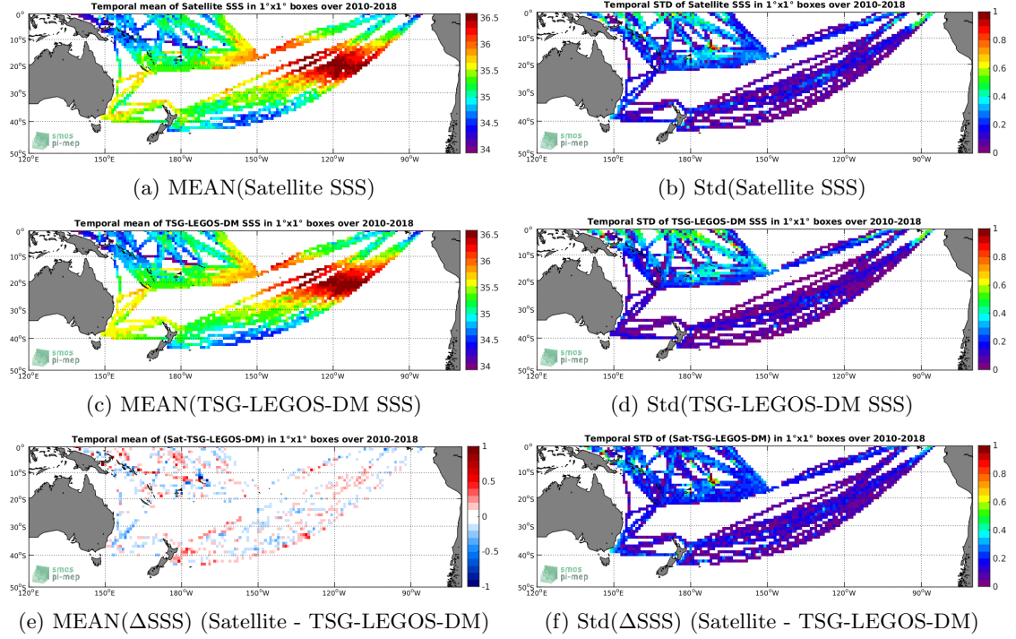
Figure 6: Temporal mean (left) and Std (right) of SSS from SMOS-L3-CATDS-CPDC-V317-MONTHLY-25KM satellite SSS product (in black), TSG-LEGOS-DM (middle), and of \Delta SSS (Satellite - TSG-LEGOS-DM). Only match-up pairs are used to generate these maps.
