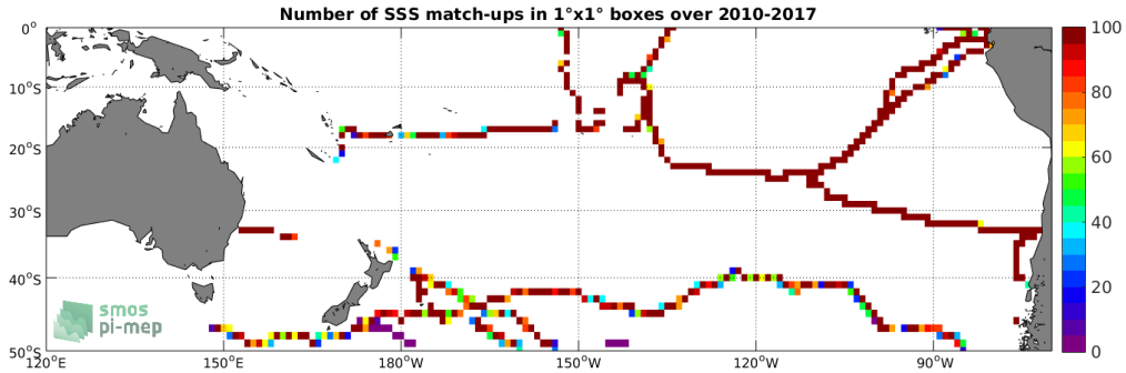
Figure 4: Number of SSS match-ups between TSG (GOSUD-Sailing-ship) SSS and the SMOS SSS L3 v317 - Monthly - 25 km (CATDS-CPDC) SSS product for the South Pacific Ocean Pi-MEP region over 1^\circ \times 1^\circ boxes and for the full satellite product period.
