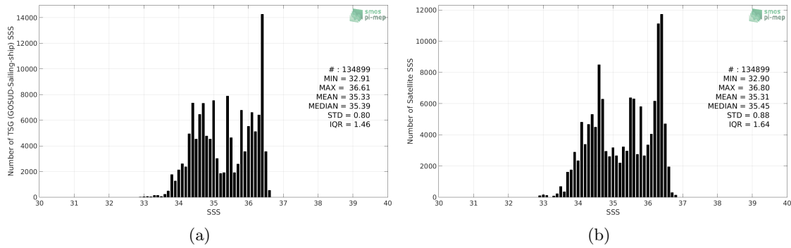
Figure 2: Histograms of SSS from TSG (GOSUD-Sailing-ship) (a) and SMOS SSS L3 v317 - Monthly - 25 km (CATDS-CPDC) (b) considering all match-up pairs per bins of 0.1 over the South Pacific Ocean Pi-MEP region and for the full satellite product period.
