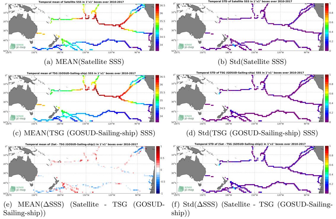
Figure 6: Temporal mean (left) and Std (right) of SSS from SMOS SSS L3 v317 - Monthly - 25 km (CATDS-CPDC) (top), TSG (GOSUD-Sailing-ship) (middle), and of \Delta SSS (Satellite - TSG (GOSUD-Sailing-ship)). Only match-up pairs are used to generate these maps.
