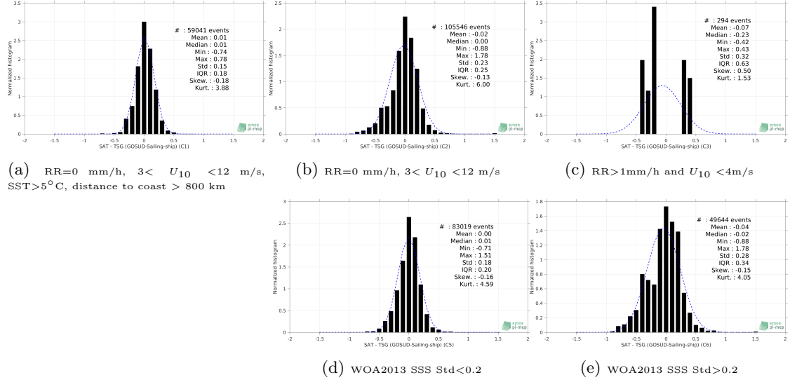
Figure 13: Normalized histogram of \Delta\text{SSS} (SMOS SSS L3 v317 - Monthly - 25 km (CATDS-CPDC) - TSG (GOSUD-Sailing-ship)) for 5 different subdatasets corresponding to: RR=0 mm/h, 3 < U_{10} < 12 m/s, SST > 5^\circ\text{C} , distance to coast > 800 km (a), RR=0 mm/h, 3 < U_{10} < 12 m/s (b), RR > 1\text{mm/h} and U_{10} < 4\text{m/s} (c), WOA2013 SSS Std <0.2 (d), WOA2013 SSS Std >0.2 (e).
