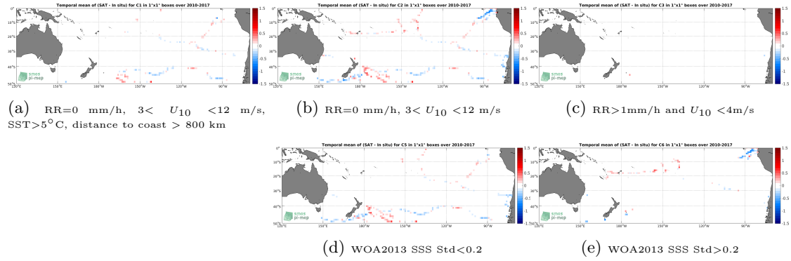
Figure 12: Temporal mean gridded over spatial boxes of size 1^\circ \times 1^\circ of \Delta SSS (SMOS SSS L3 v317 - Monthly - 25 km (CATDS-CPDC) - TSG (GOSUD-Sailing-ship)) for 5 different subdatasets corresponding to: RR=0 mm/h, 3 < U_{10} < 12 m/s, SST >5^\circ\text{C} , distance to coast > 800 km (a), RR=0 mm/h, 3 < U_{10} < 12 m/s (b), RR>1\text{mm/h} and U_{10} < 4\text{m/s} (c), WOA2013 SSS Std <0.2 (d), WOA2013 SSS Std >0.2 (e).
